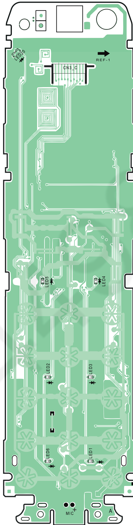
KX-TGEA20 CIRCUIT BOARD (Handset_Main (Bottom View))
