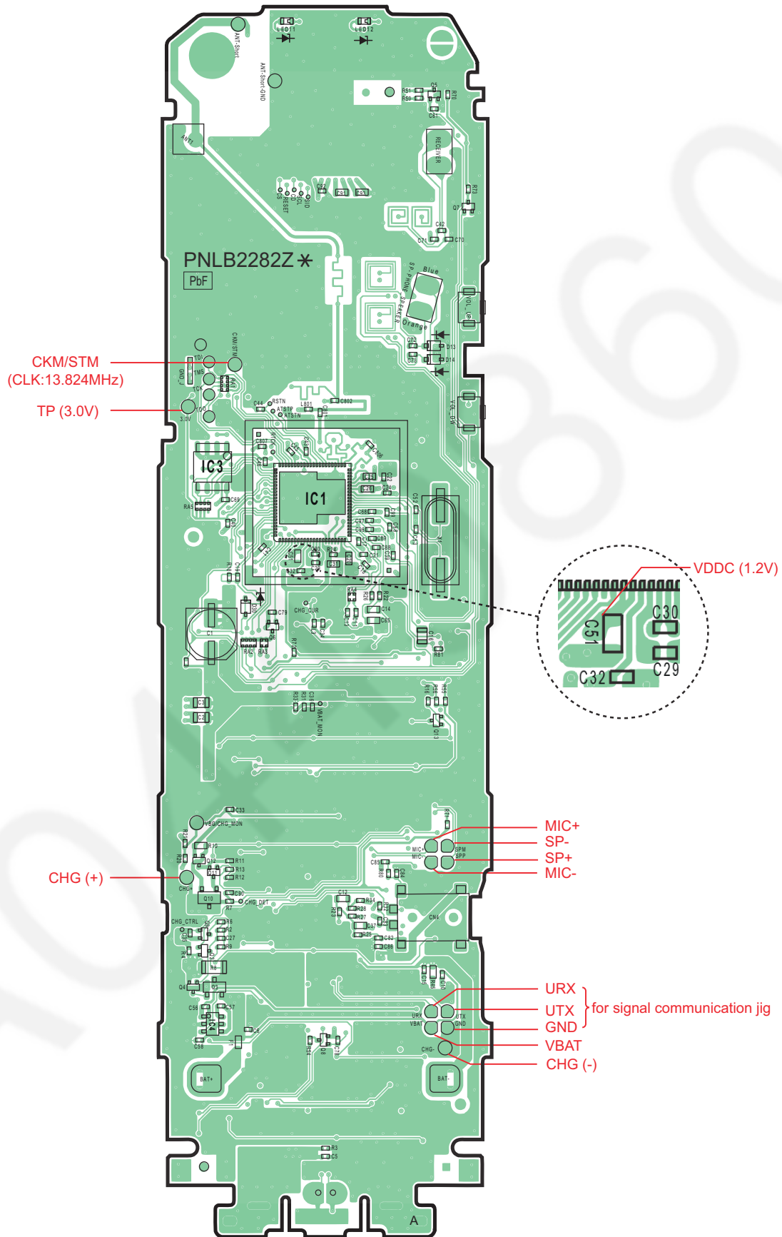
KX-TGEA20 CIRCUIT BOARD (Handset_Main (Component View))
