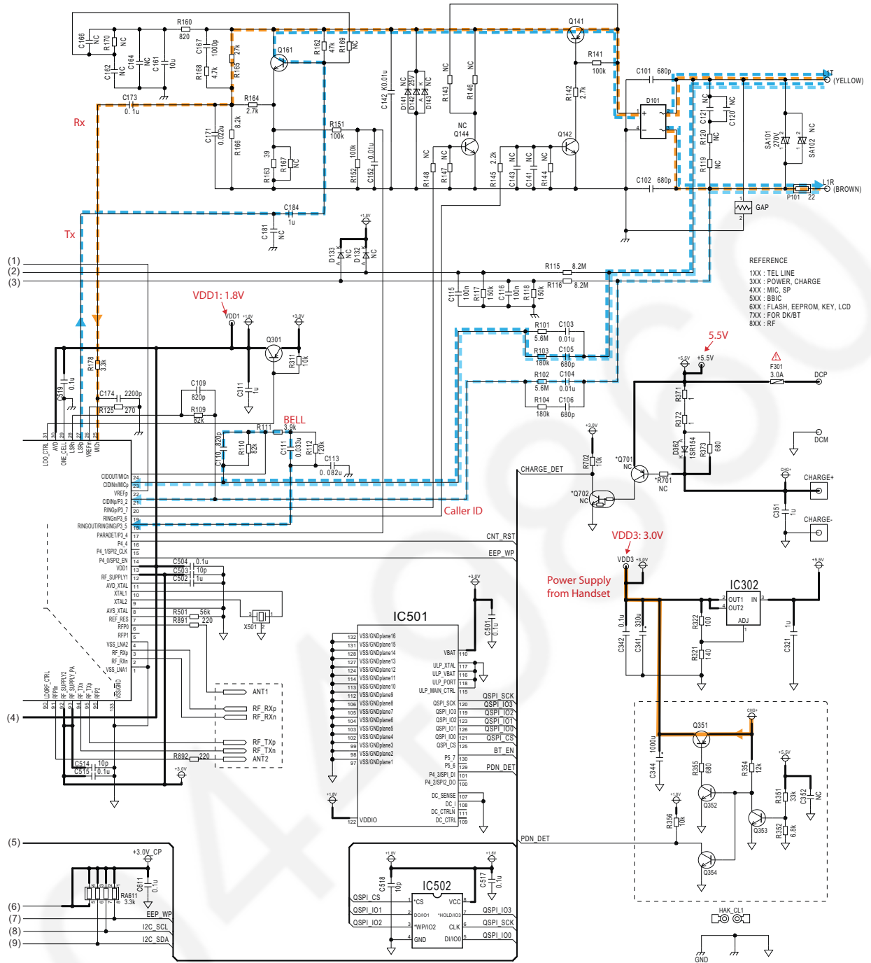
KX-TGE260/262/263/264/TG454 SCHEMATIC DIAGRAM (Base Unit (Main))
