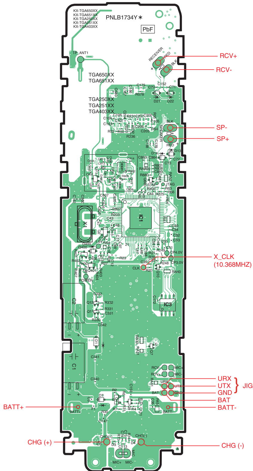
KX-TGA651 CIRCUIT BOARD (Handset_Main (Component View))
