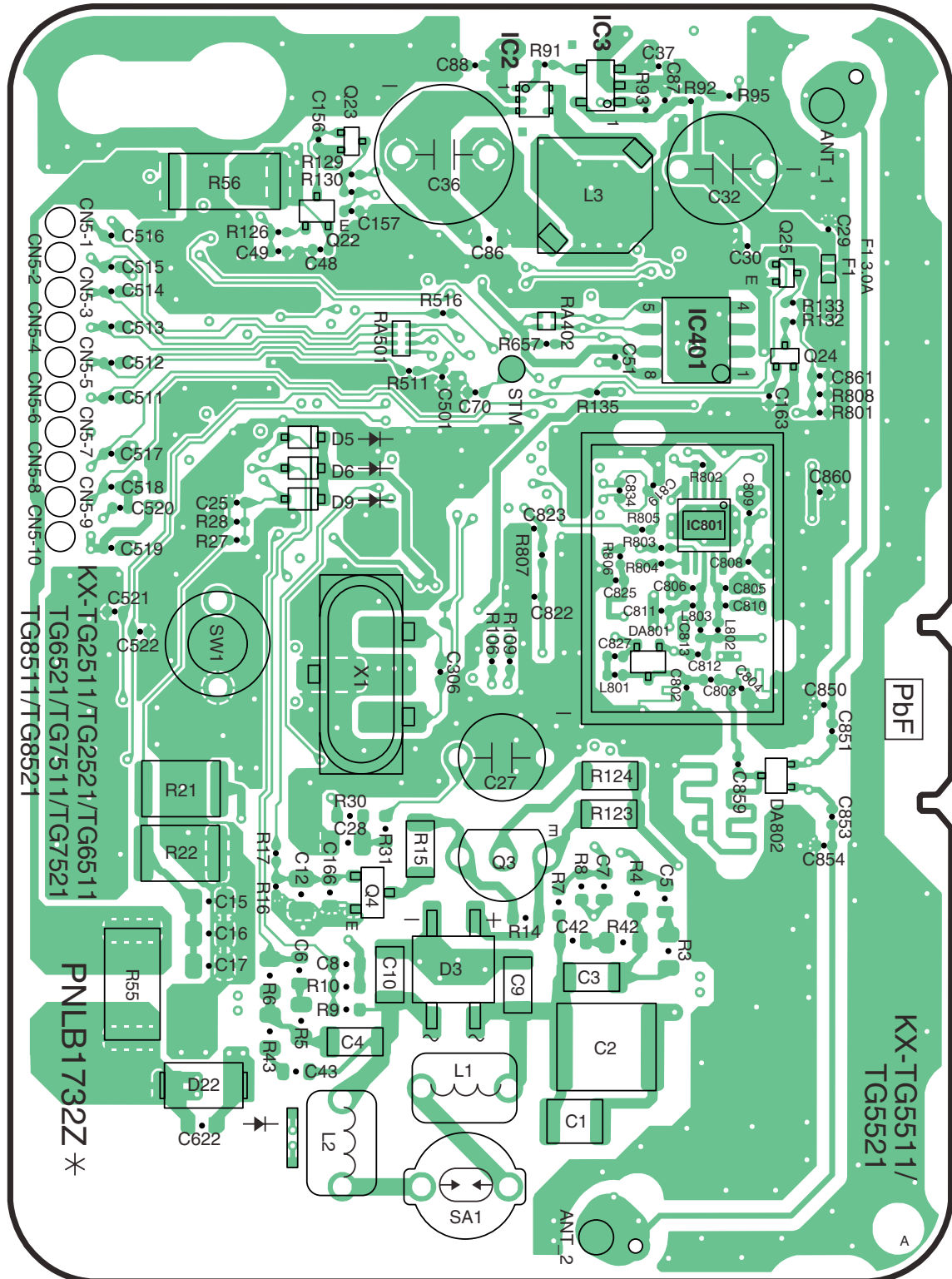
KX-TG6511/6512/6513/6519 CIRCUIT BOARD (Base Unit_Main (Component View))
