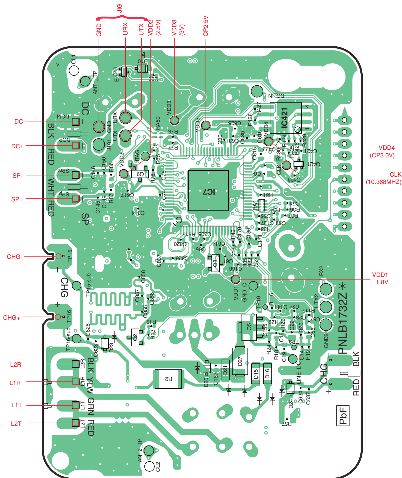
KX-TG6511/6512/6513/6519 CIRCUIT BOARD (Base Unit_Main (Bottom View))
