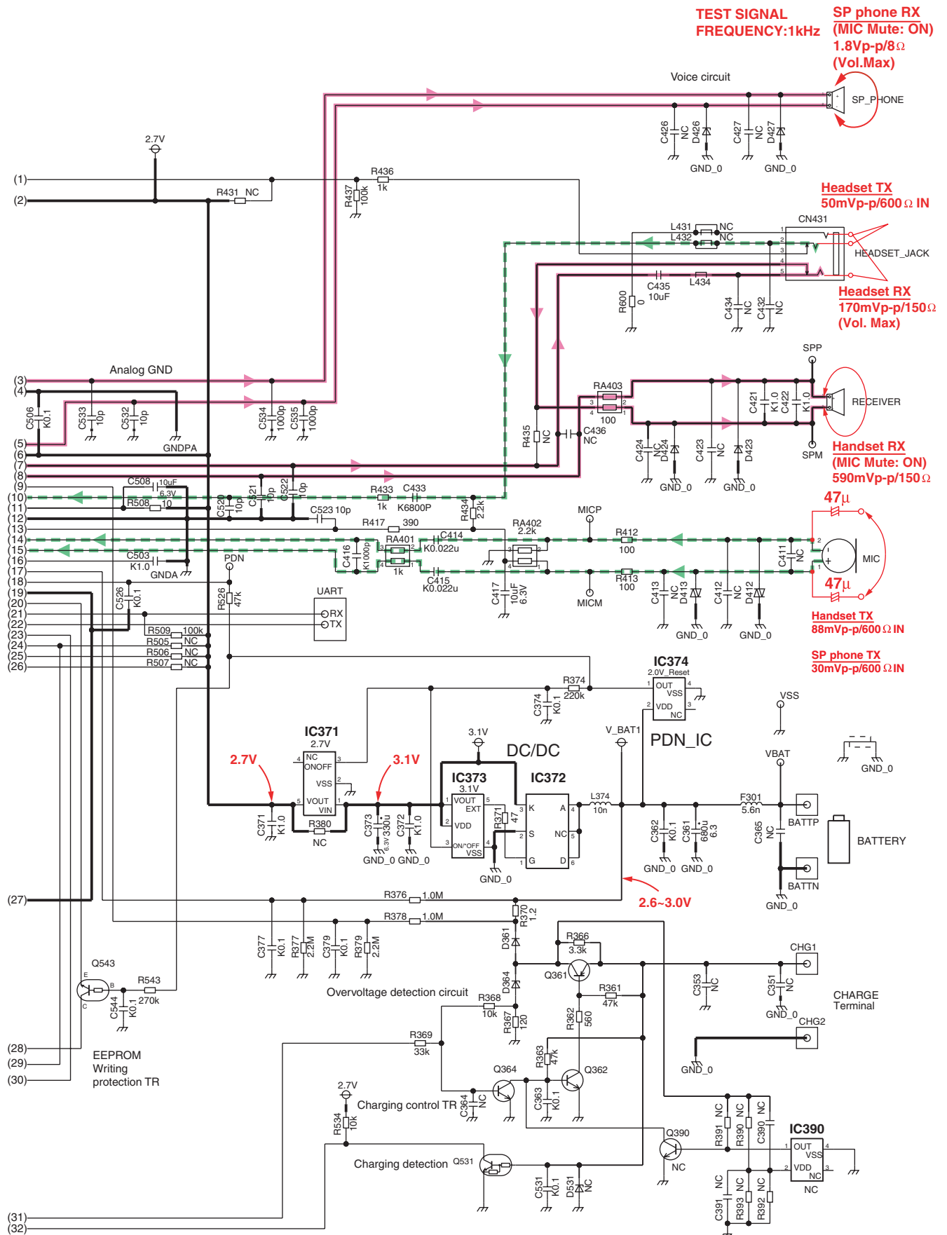
KX-TGA641 SCHEMATIC DIAGRAM (Handset_Main)
