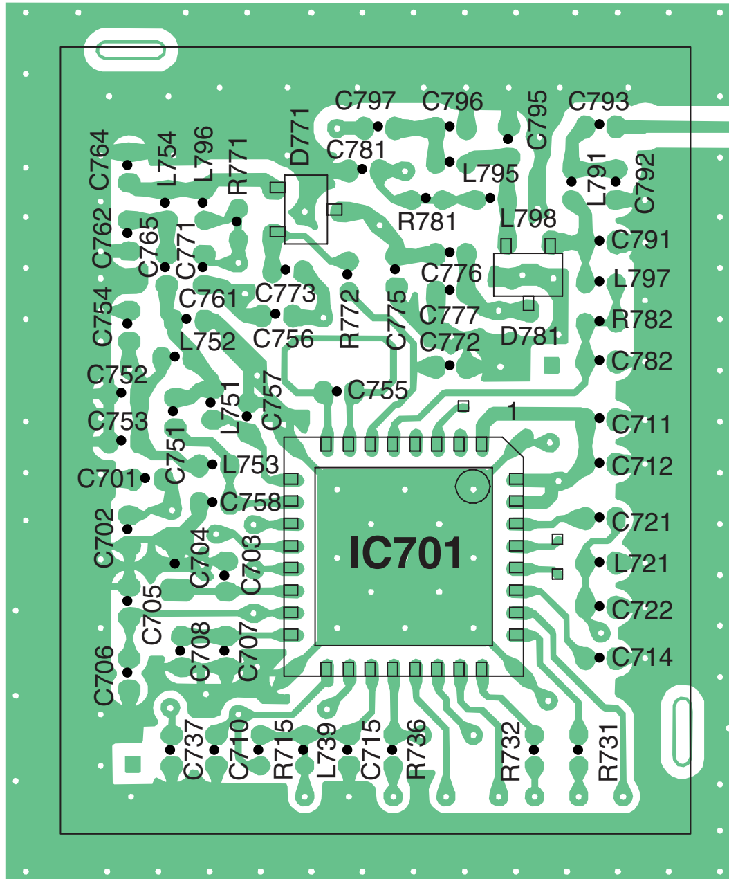
KX-TG6441/6442/6443/6444/6445 CIRCUIT BOARD (Base Unit_RF Part (Component View))
