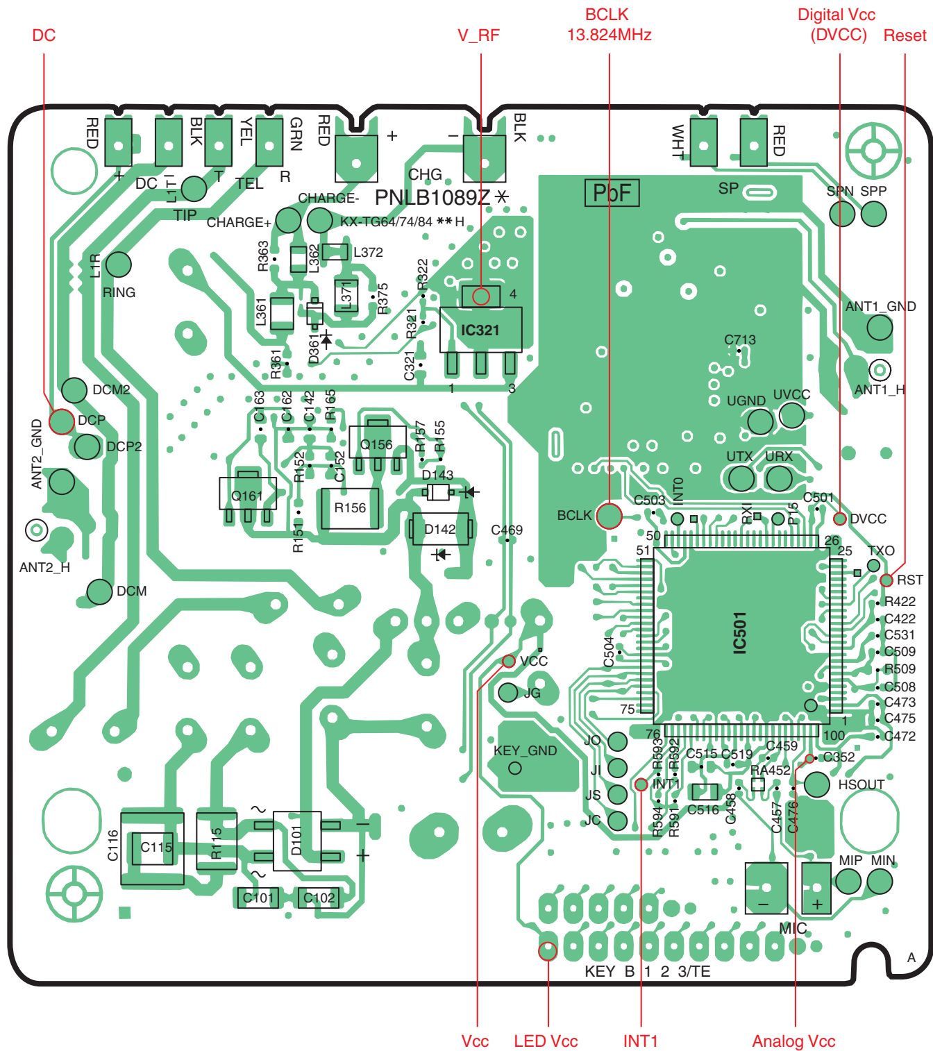
KX-TG6441/6442/6443/6444/6445 CIRCUIT BOARD (Base Unit_Main (Bottom View))
