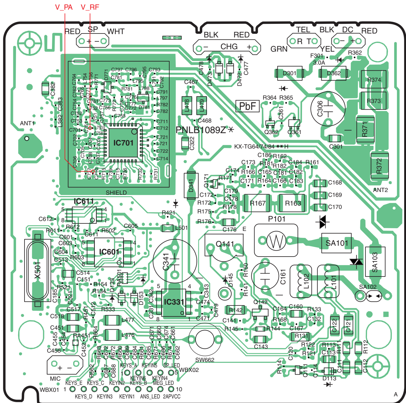
KX-TG6441/6442/6443/6444/6445 CIRCUIT BOARD (Base Unit_Main (Component View))
