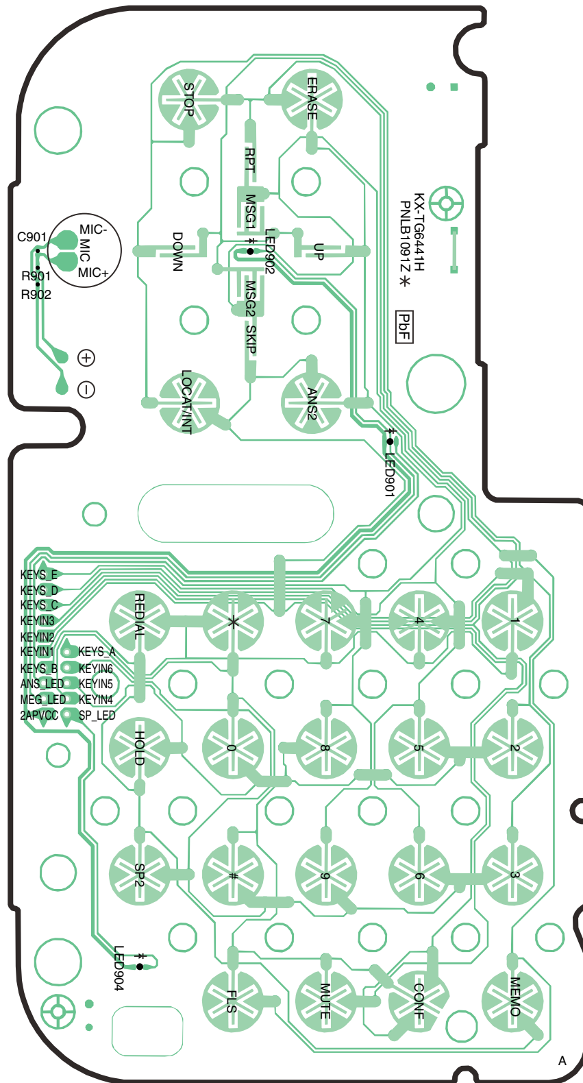
KX-TG6441/6442/6443/6444/6445 CIRCUIT BOARD (Base Unit_Operation (Component View))
