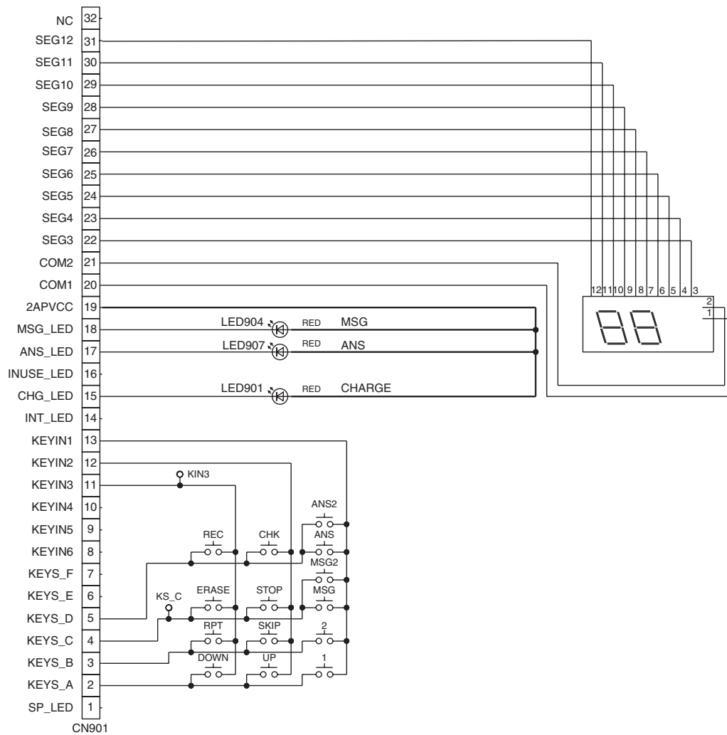
KX-TG5631/5632/5633 SCHEMATIC DIAGRAM (Base Unit_Operation)
