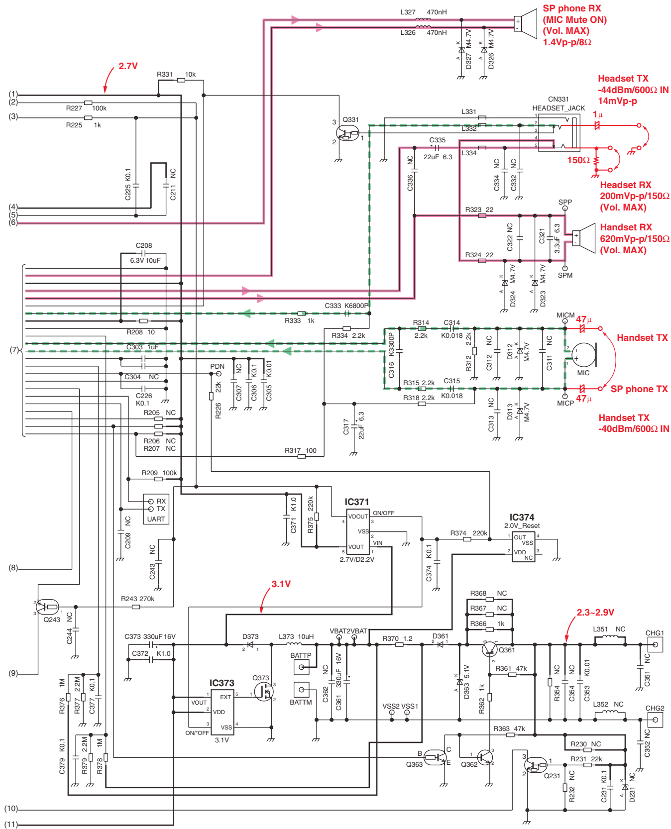
KX-TGA670 SCHEMATIC DIAGRAM (Handset_Main)
