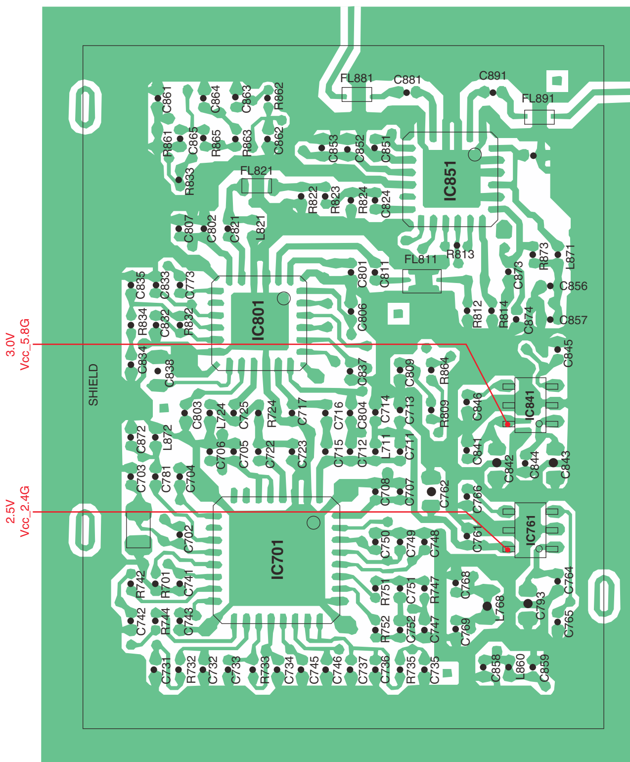
KX-TG6700 CIRCUIT BOARD (Base Unit_RF Part (Component View))
