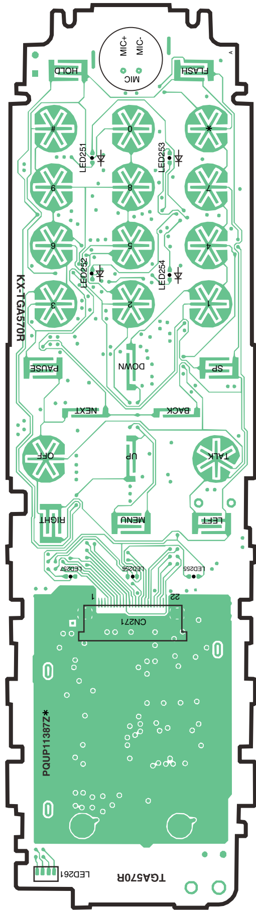
KX-TGA670 CIRCUIT BOARD (Handset_Main (Flow Solder Side View))
