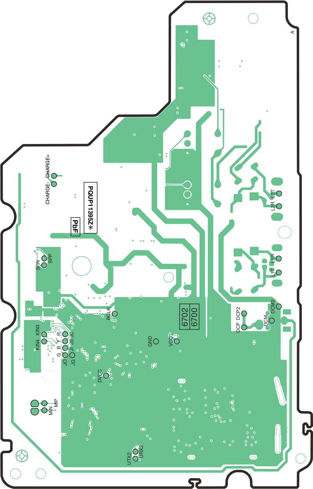
KX-TG6700 CIRCUIT BOARD (Base Unit (Flow Solder Side View))
