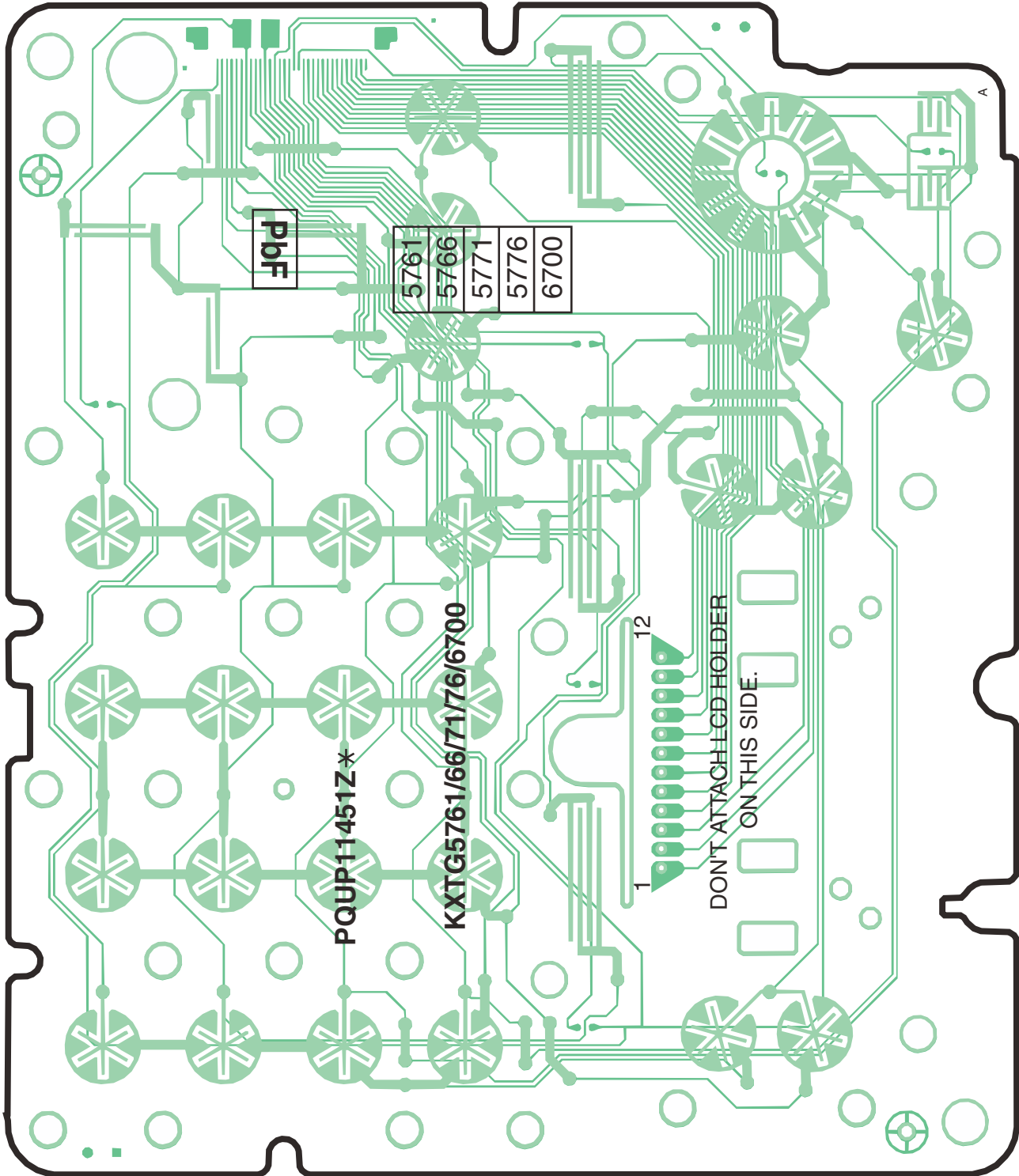
KX-TG6700 CIRCUIT BOARD (Base Unit_Operation (Flow Solder Side View))
