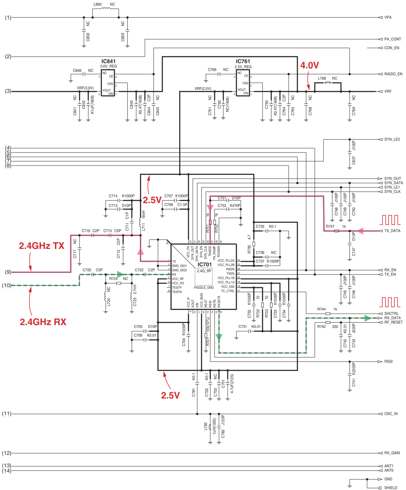
KX-TG6700 SCHEMATIC DIAGRAM (Base Unit_RF Part)
