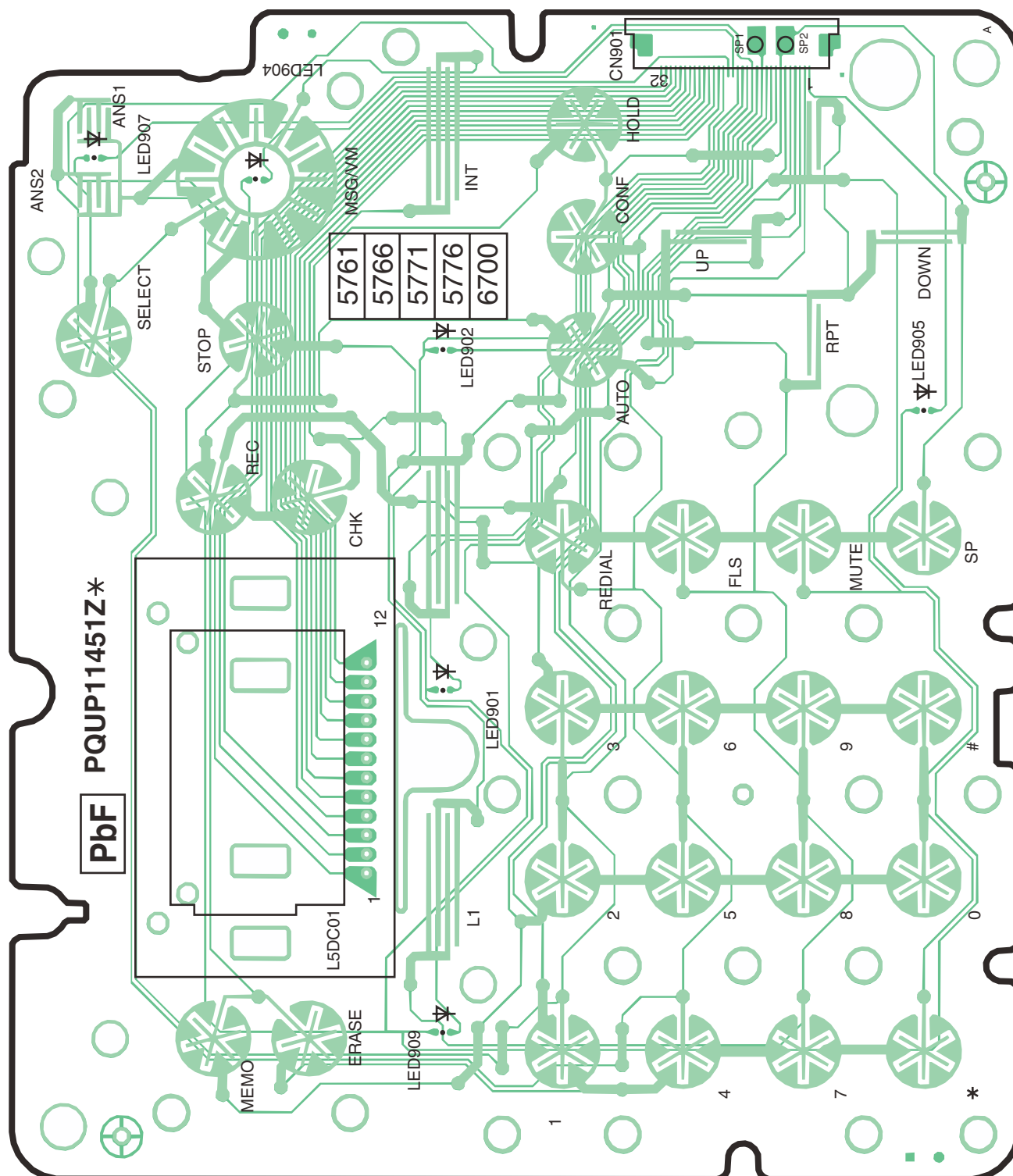
KX-TG6700 CIRCUIT BOARD (Base Unit_Operation (Component View))
