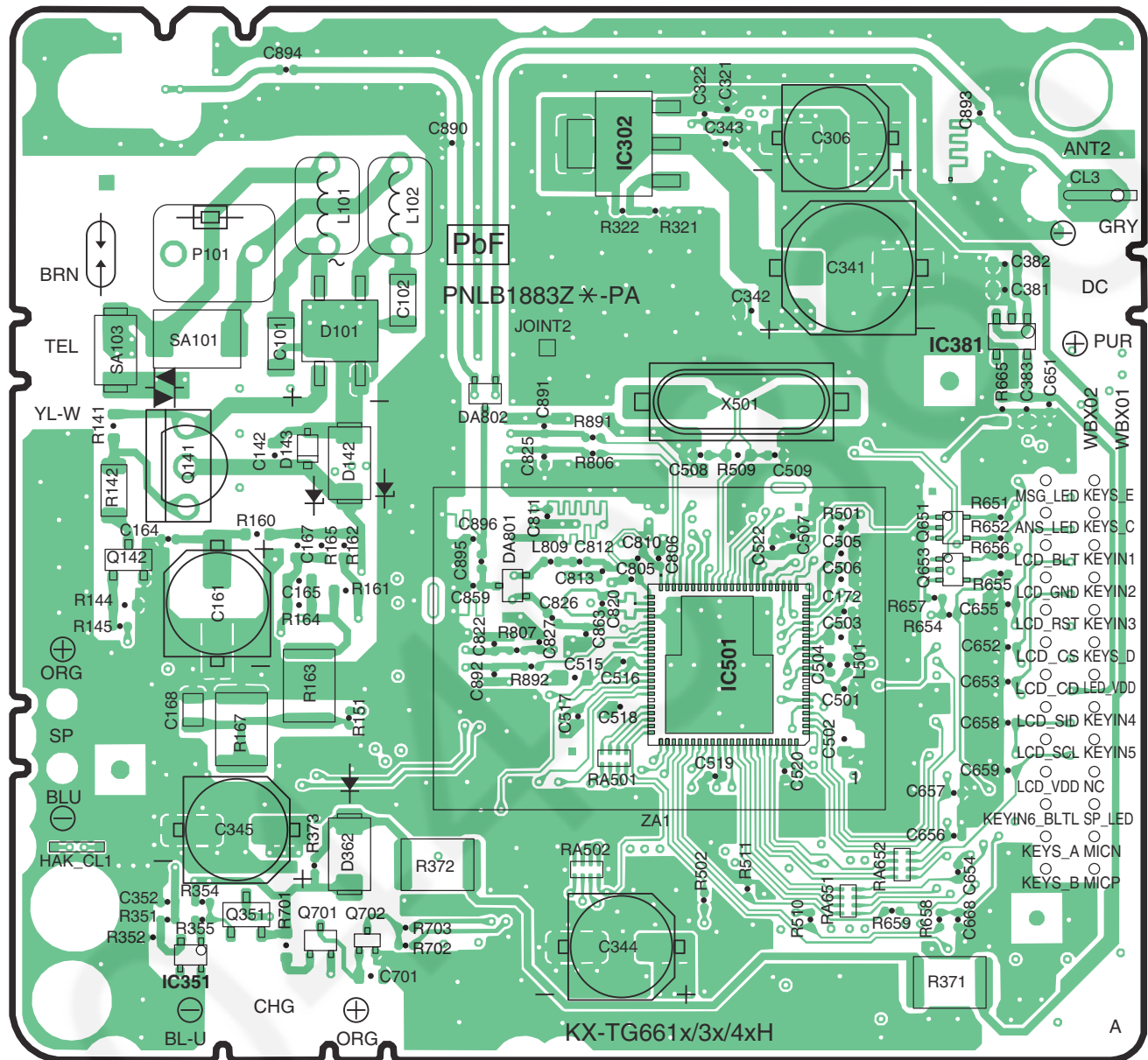
KX-TG6641/6643/6644/6645 CIRCUIT BOARD (Base Unit_Main (Component View))
