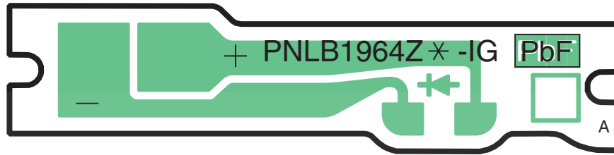
KX-TGA660 CIRCUIT BOARD (Handset_LED (Component View))
