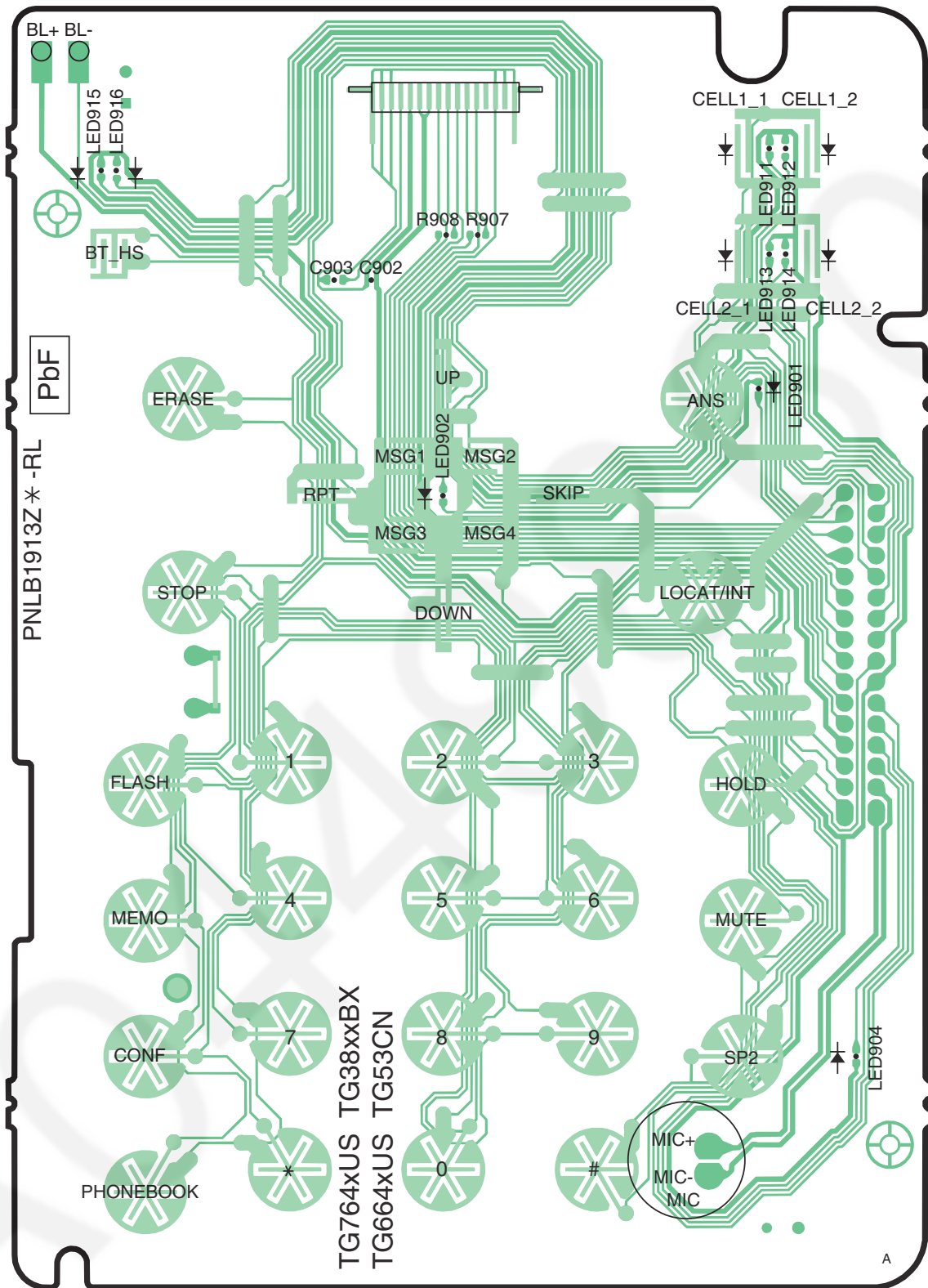
KX-TG6641/6643/6644/6645 CIRCUIT BOARD (Base Unit_Operation (Component View))
