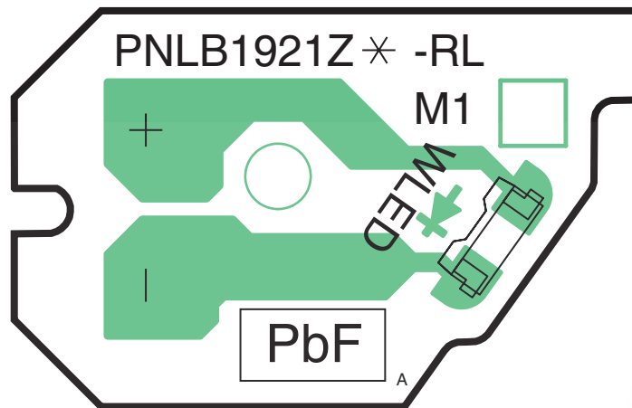
KX-TG6641/6643/6644/6645 CIRCUIT BOARD (Base Unit_LED (Component View))
