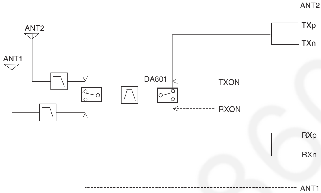
KX-TG6641/6643/6644/6645 BLOCK DIAGRAM (Base Unit_RF Part)
