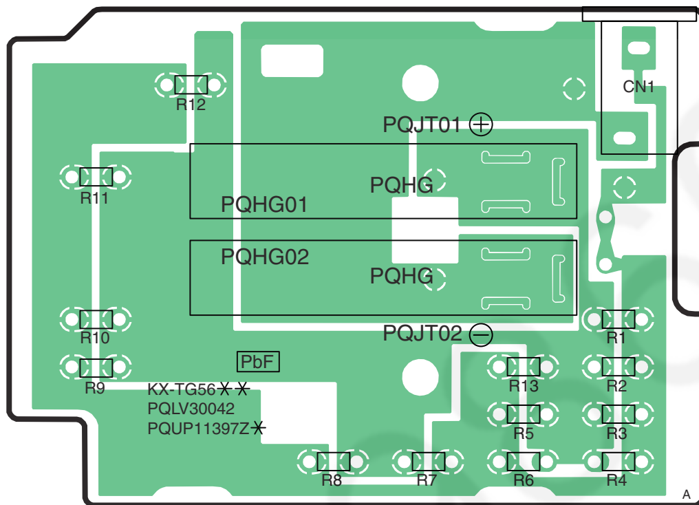
CIRCUIT BOARD (Charger Unit (Component View))
