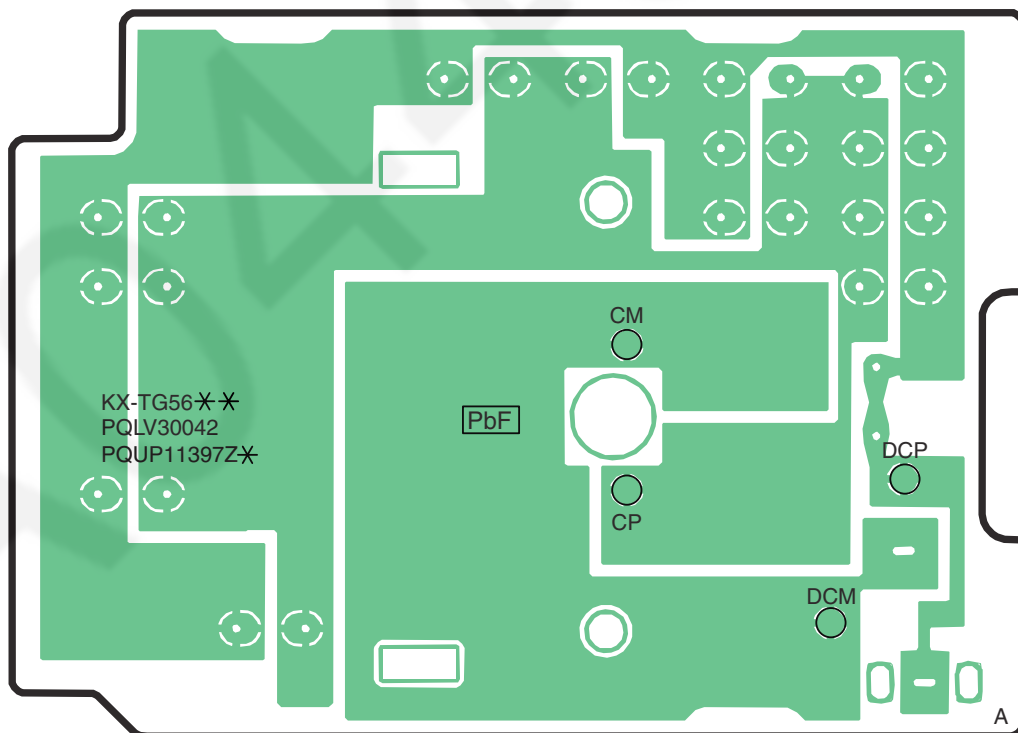
CIRCUIT BOARD (Charger Unit (Flow Solder Side View))
