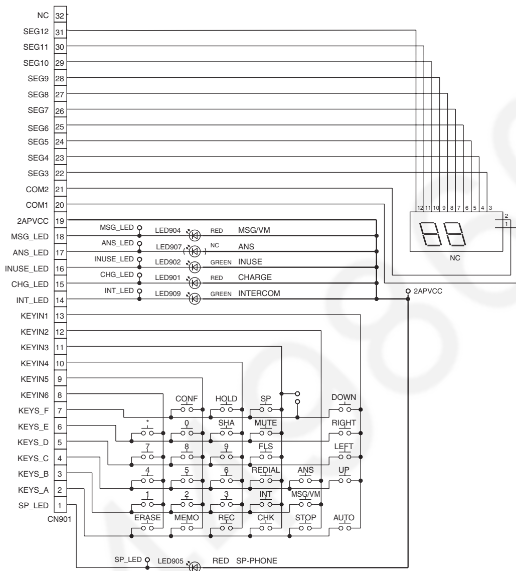
KX-TG5671/5672/5673 SCHEMATIC DIAGRAM (Base Unit_Operation)
