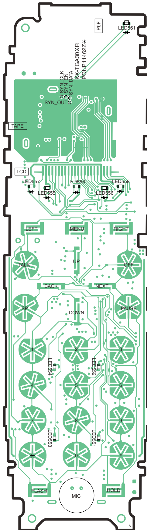
KX-TGA351 CIRCUIT BOARD (Handset (Flow Solder Side View))
