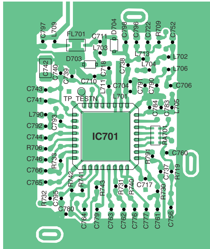
KX-TG3521/3522 CIRCUIT BOARD (Base Unit_RF Part (Component View))
