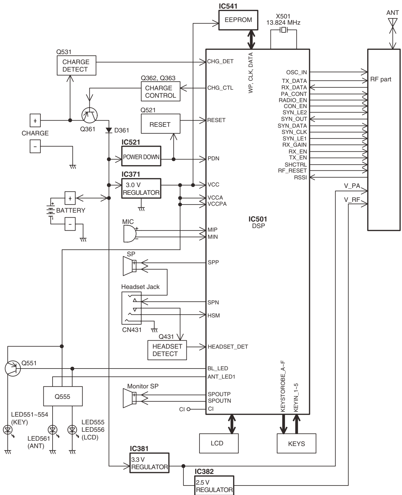
KX-TGA351 BLOCK DIAGRAM (Handset)
