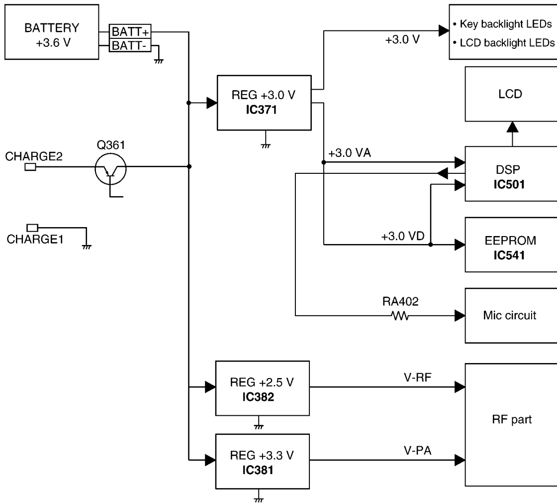
Block Diagram (Handset Power)
