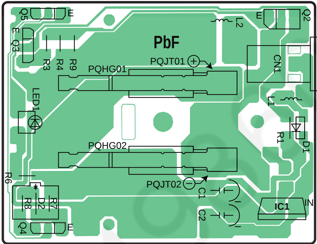
KX-TG2361JXB CIRCUIT BOARD (Component View (Charger Unit))
