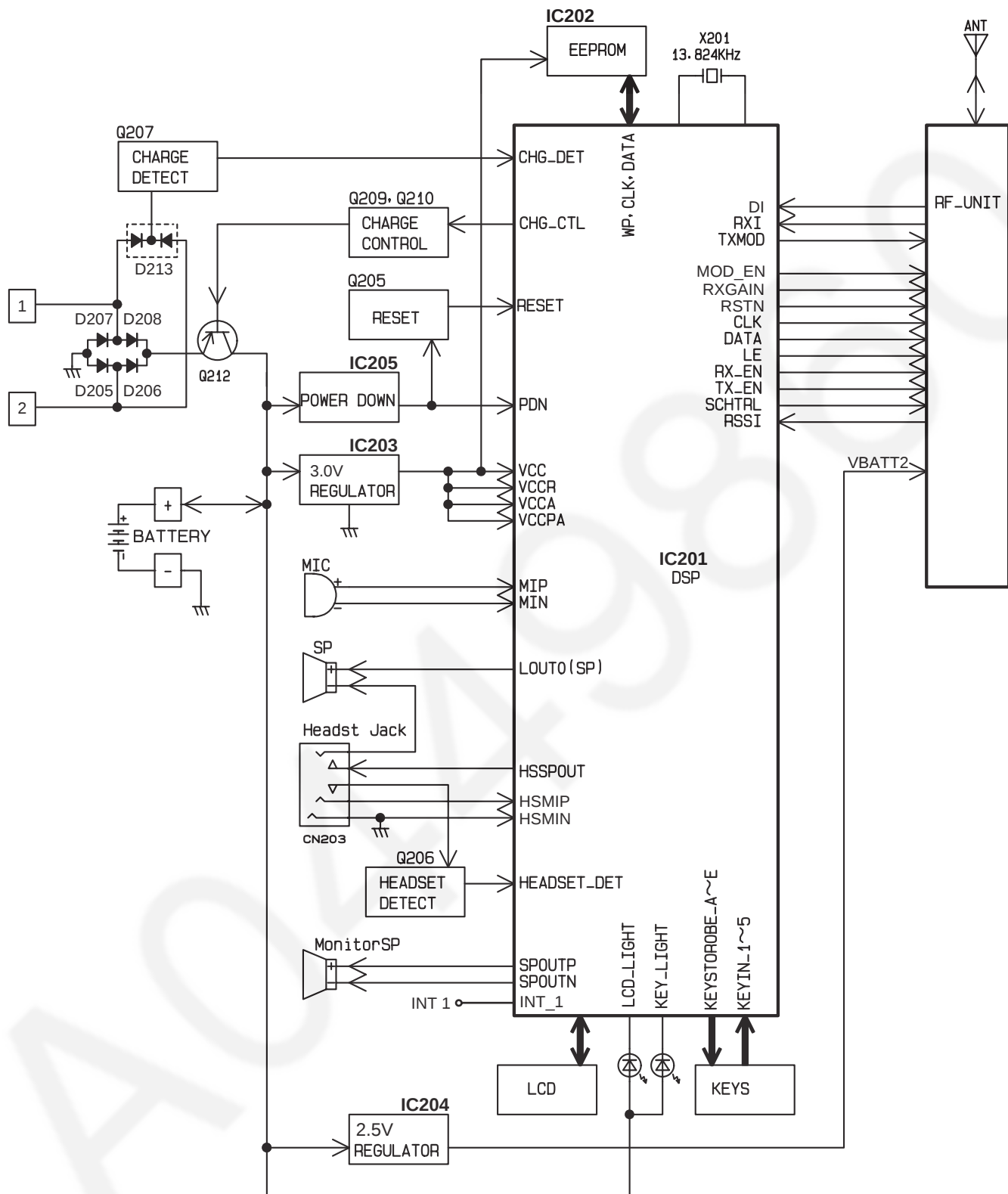
KX-TG2361JXB BLOCK DIAGRAM (Handset)
