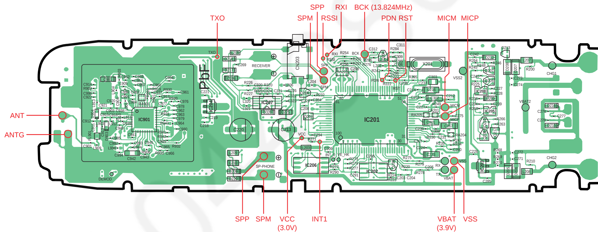
KX-TG2361JXB CIRCUIT BOARD (Component View (Handset))
