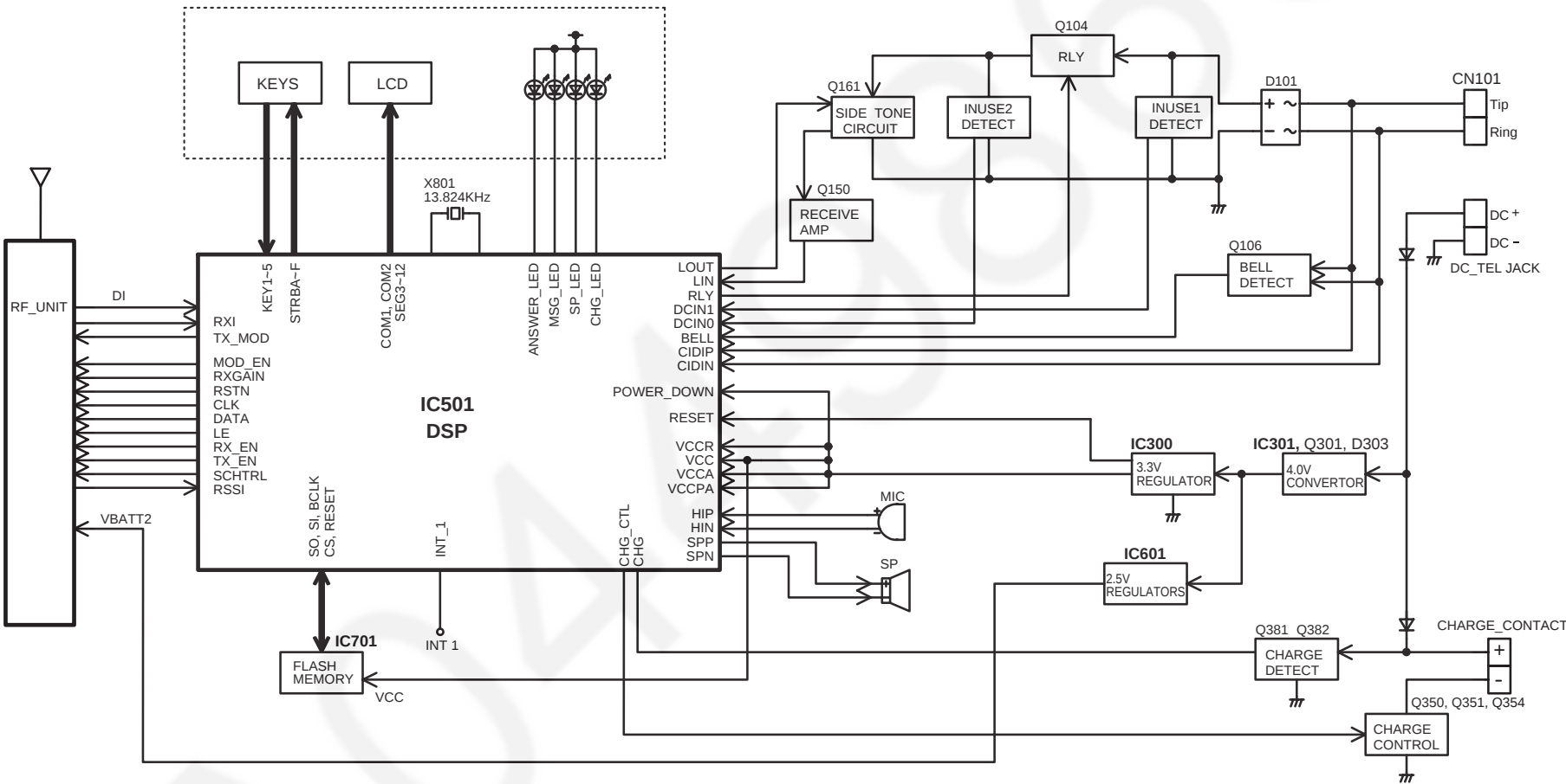
KX-TG2361JXB BLOCK DIAGRAM (Base Unit)
