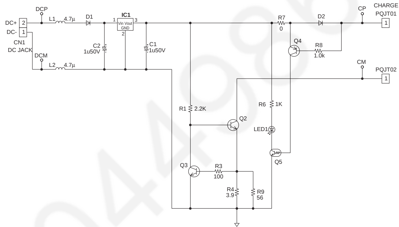
KX-TG2361JXB SCHEMATIC DIAGRAM (Charger Unit)
