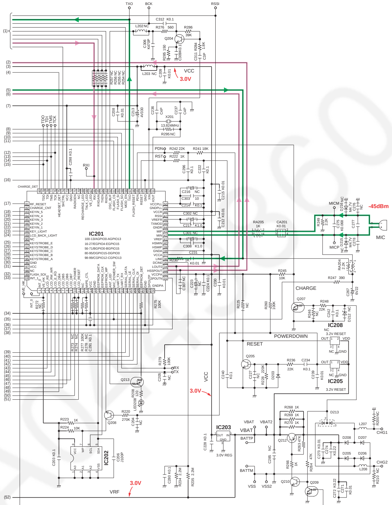
KX-TG2361JXB SCHEMATIC DIAGRAM (Handset)
