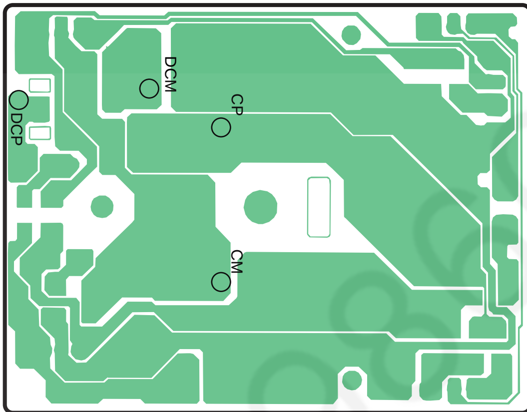
KX-TG2359BXB CIRCUIT BOARD (Flow Solder Side View (Charger Unit))
