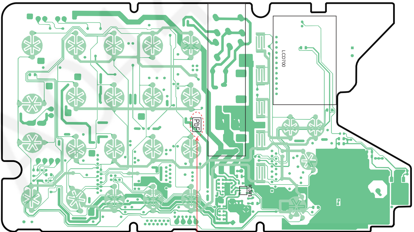
(Flow Solder Side View)
