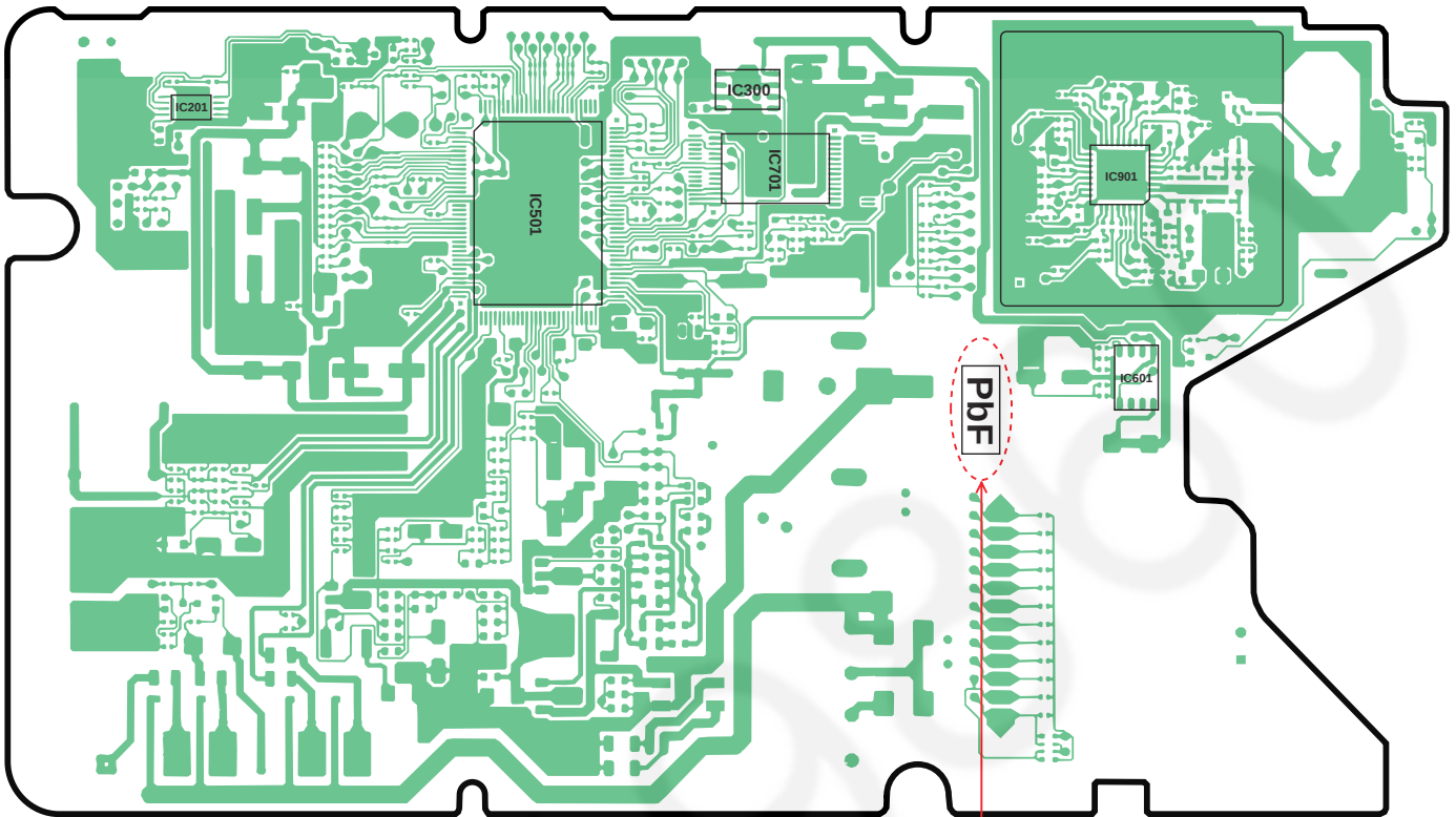
(Component View)
