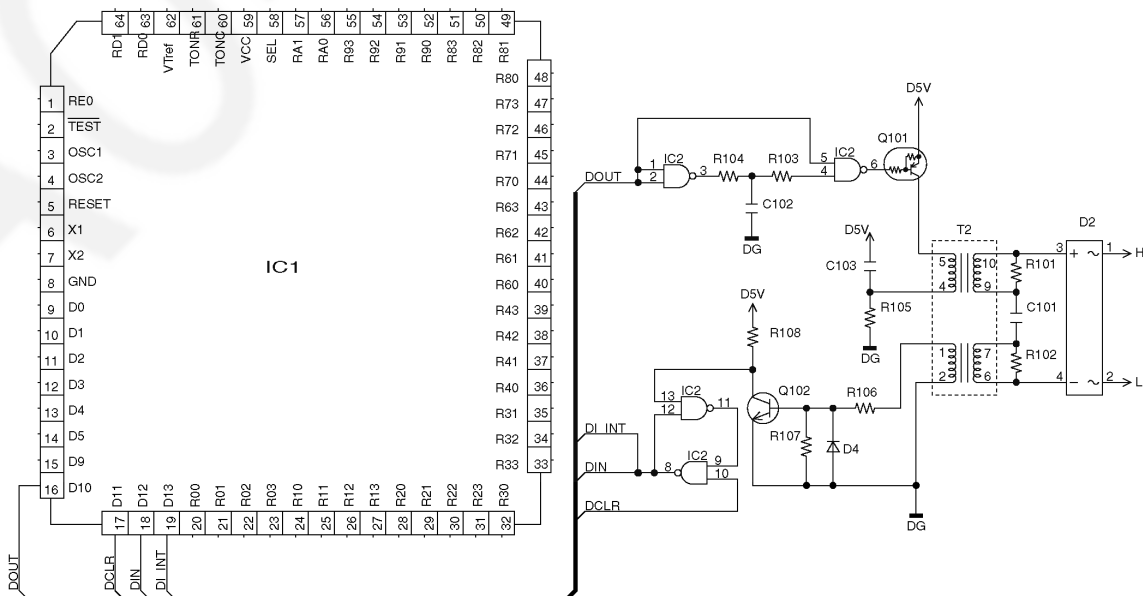
Circuit Diagram
