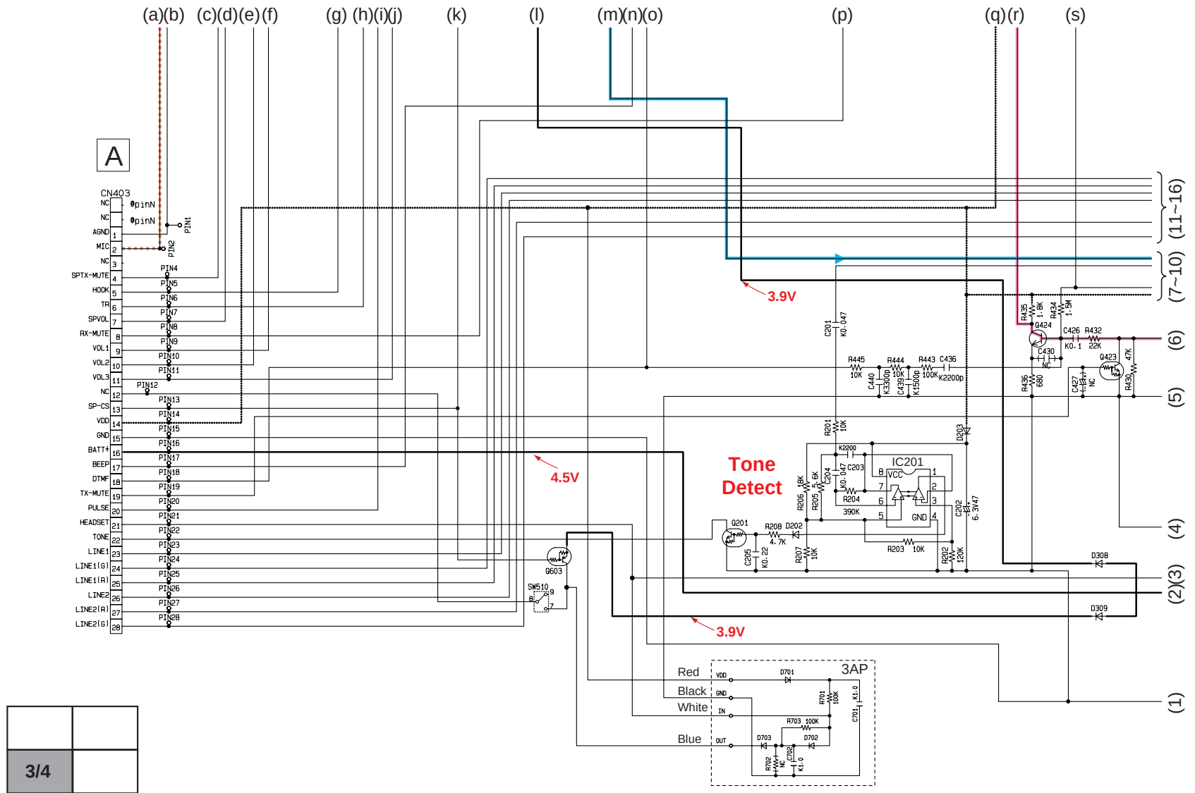
KX-T2378JXW SCHEMATIC DIAGRAM (Main (Suffix A)) 3/4
