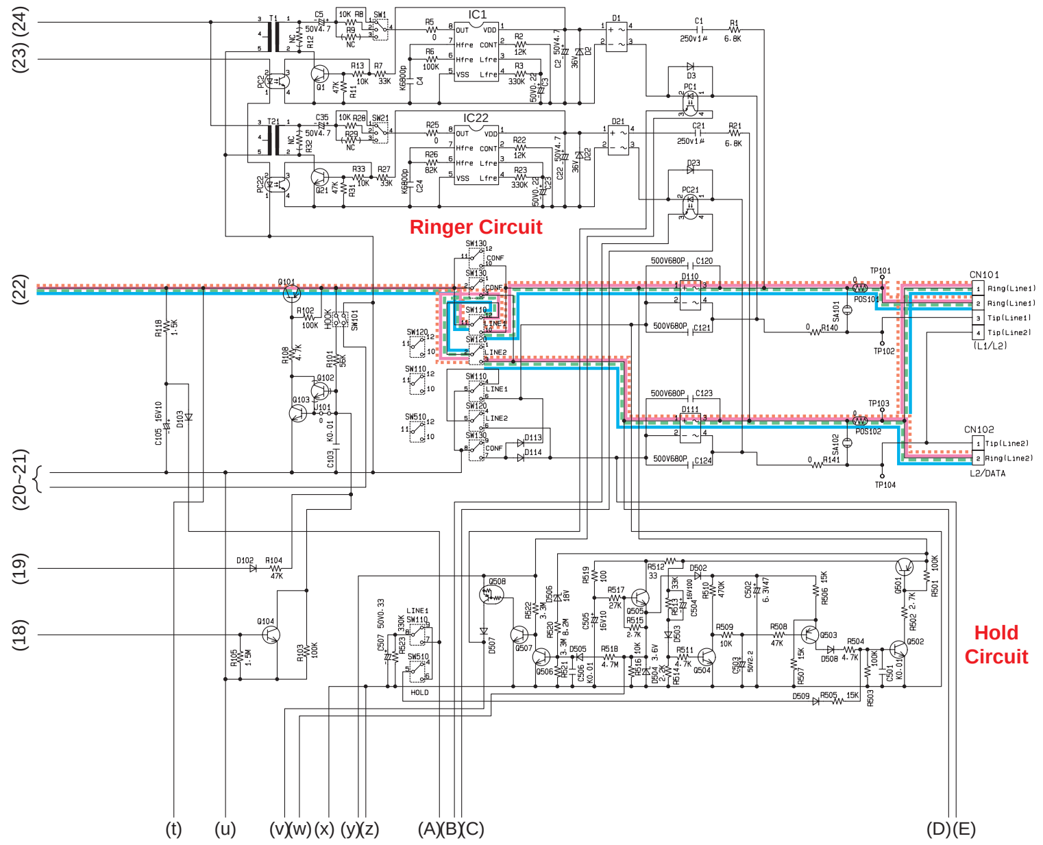
KX-T2378JXW SCHEMATIC DIAGRAM (Main (Suffix B)) 2/4
