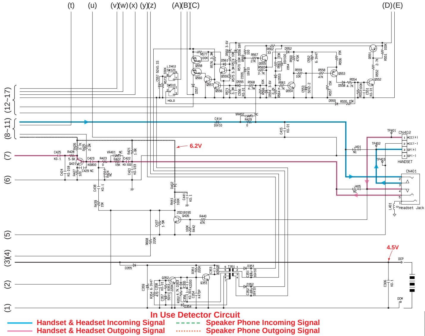
KX-T2378JXW SCHEMATIC DIAGRAM (Main (Suffix B)) 4/4
