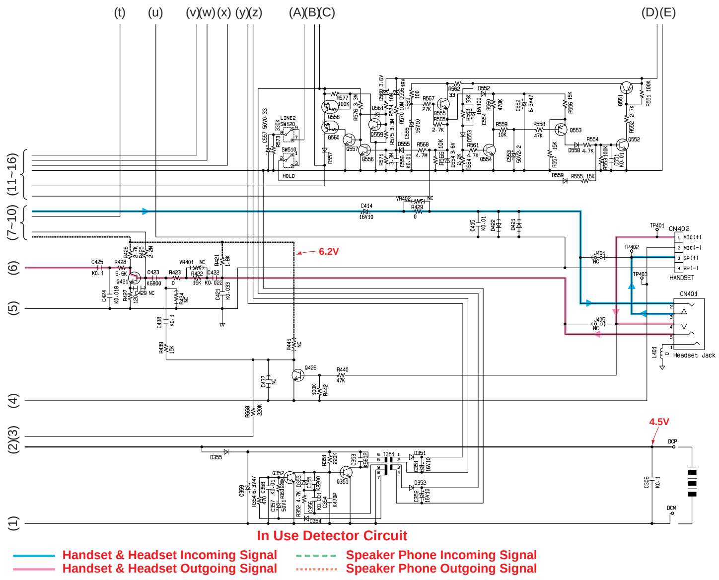
KX-T2378JXW SCHEMATIC DIAGRAM (Main (Suffix A)) 4/4
