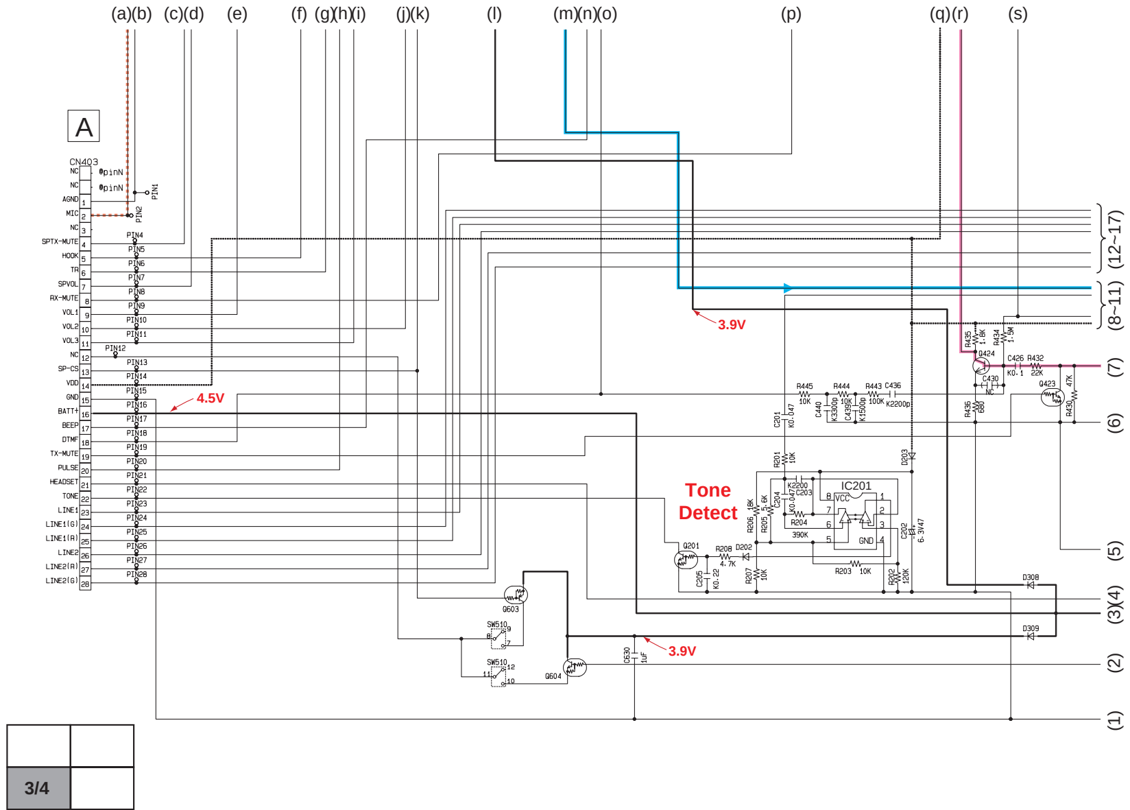
KX-T2378JXW SCHEMATIC DIAGRAM (Main (Suffix B)) 3/4
