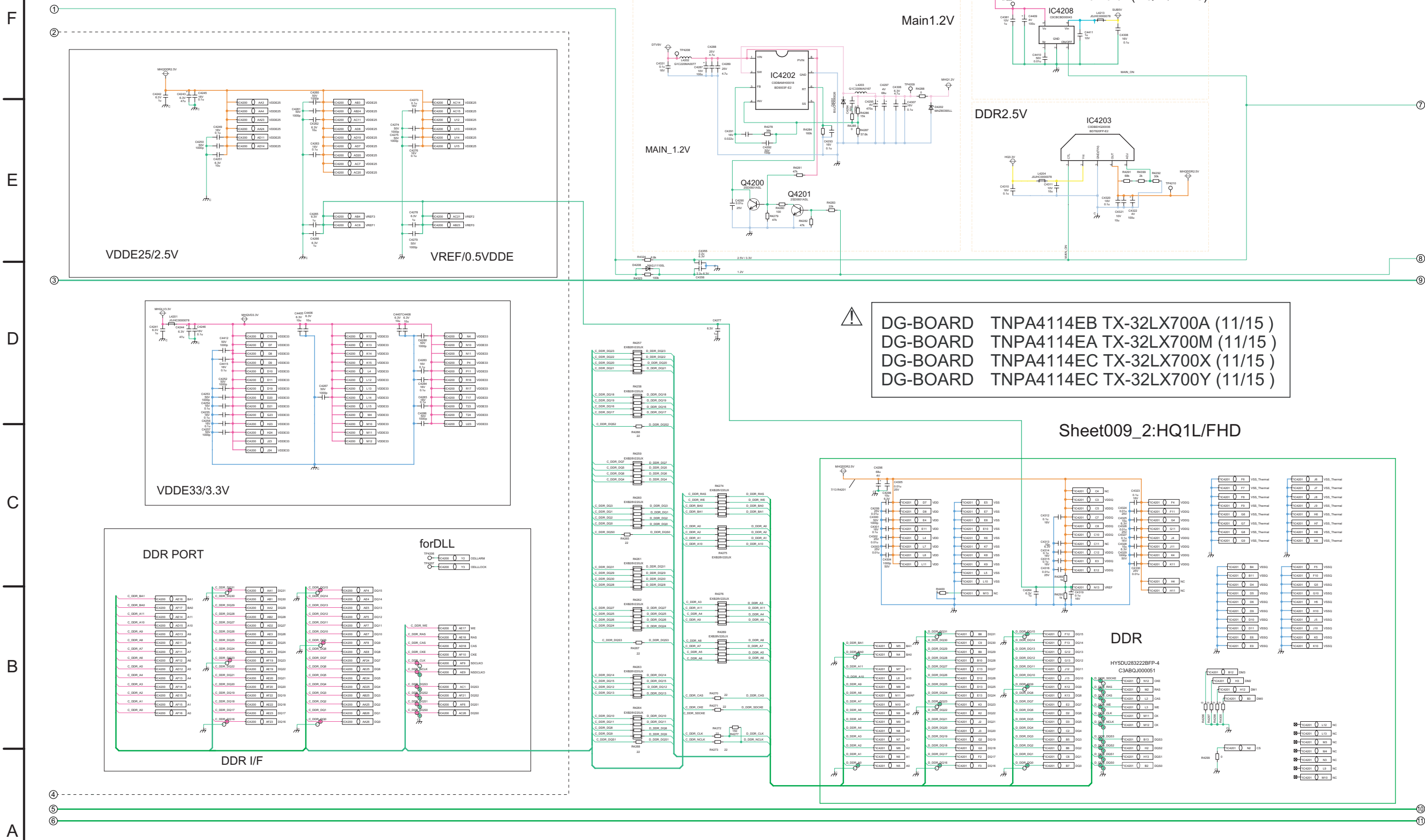
TX-32LX700A/M/X/Y DG-BOARD (11/15) Schematic Diagram
