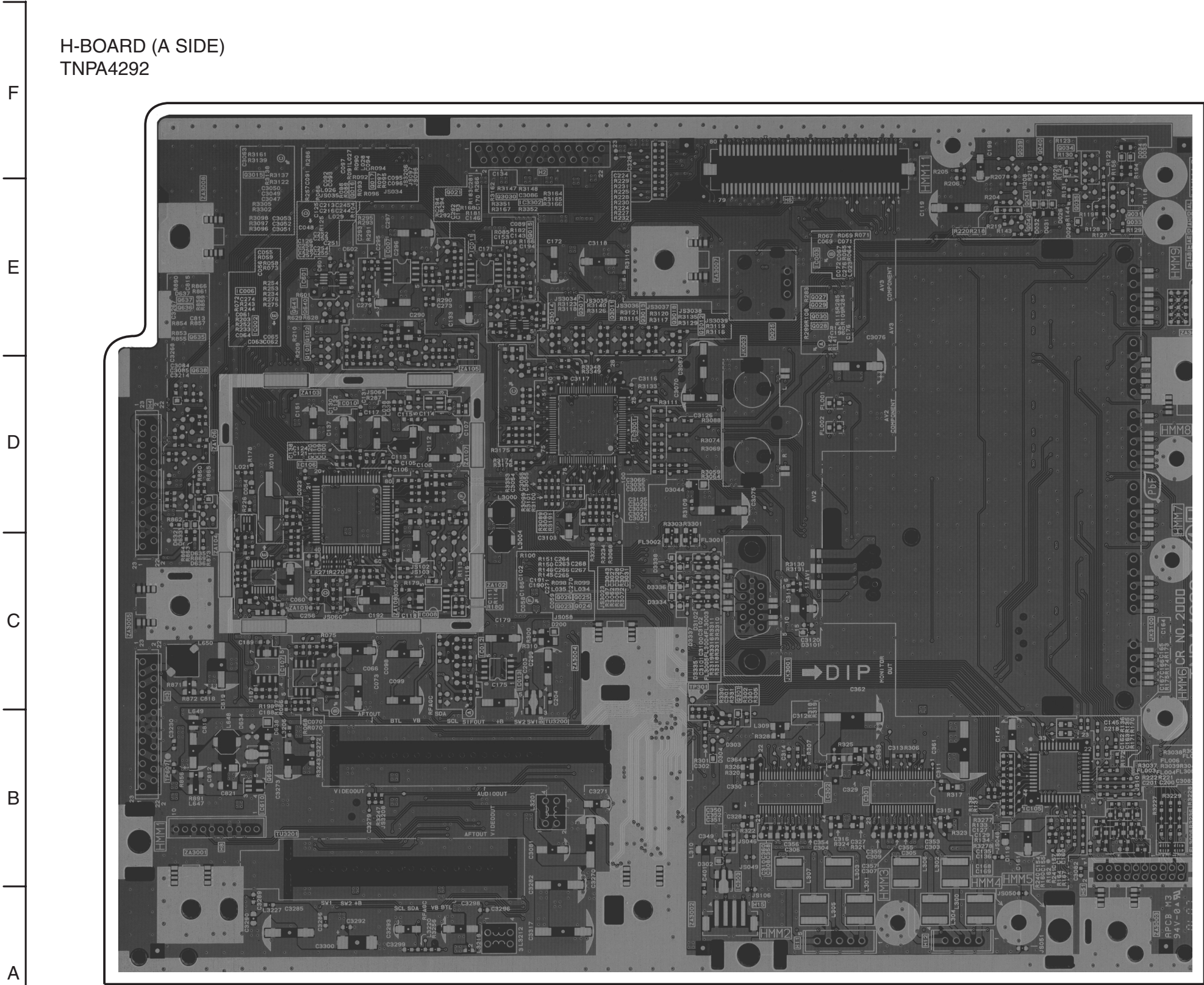
TX-32LX700A/M/X/Y H-BOARD TNPA4292
