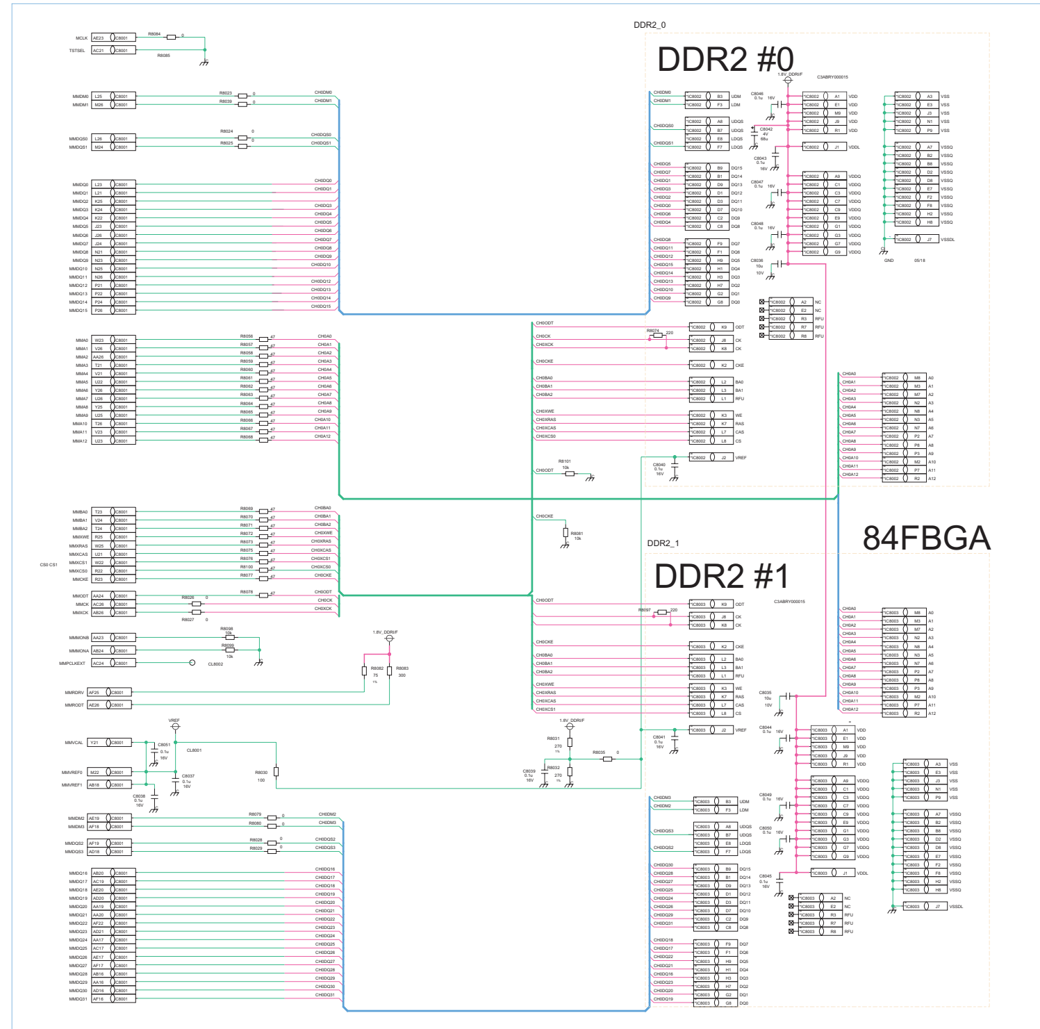
TX-32LX700A/M/X/Y DG-BOARD (3/15) Schematic Diagram
