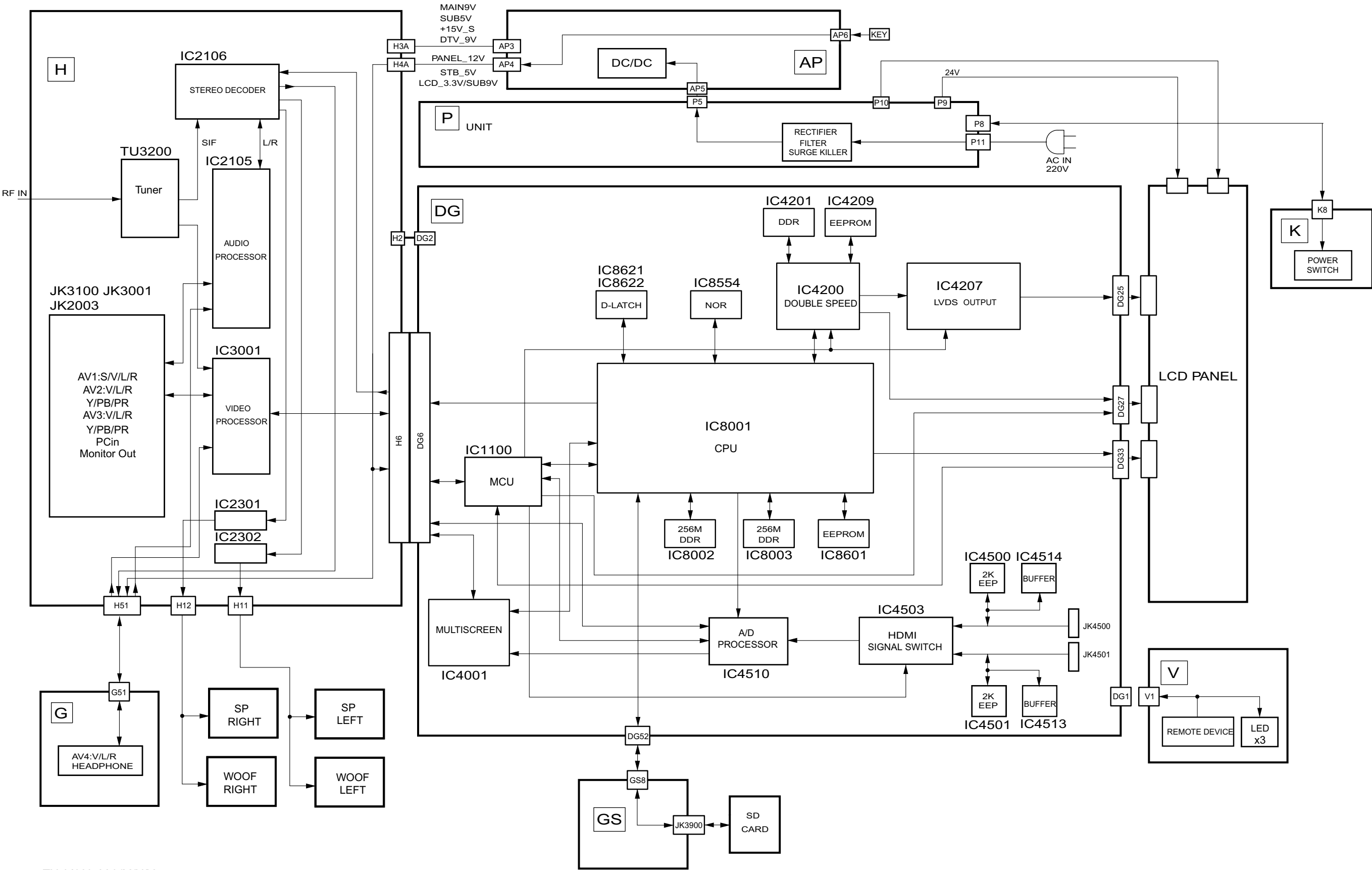
TX-32LX700A/M/X/Y Main Block Diagram
