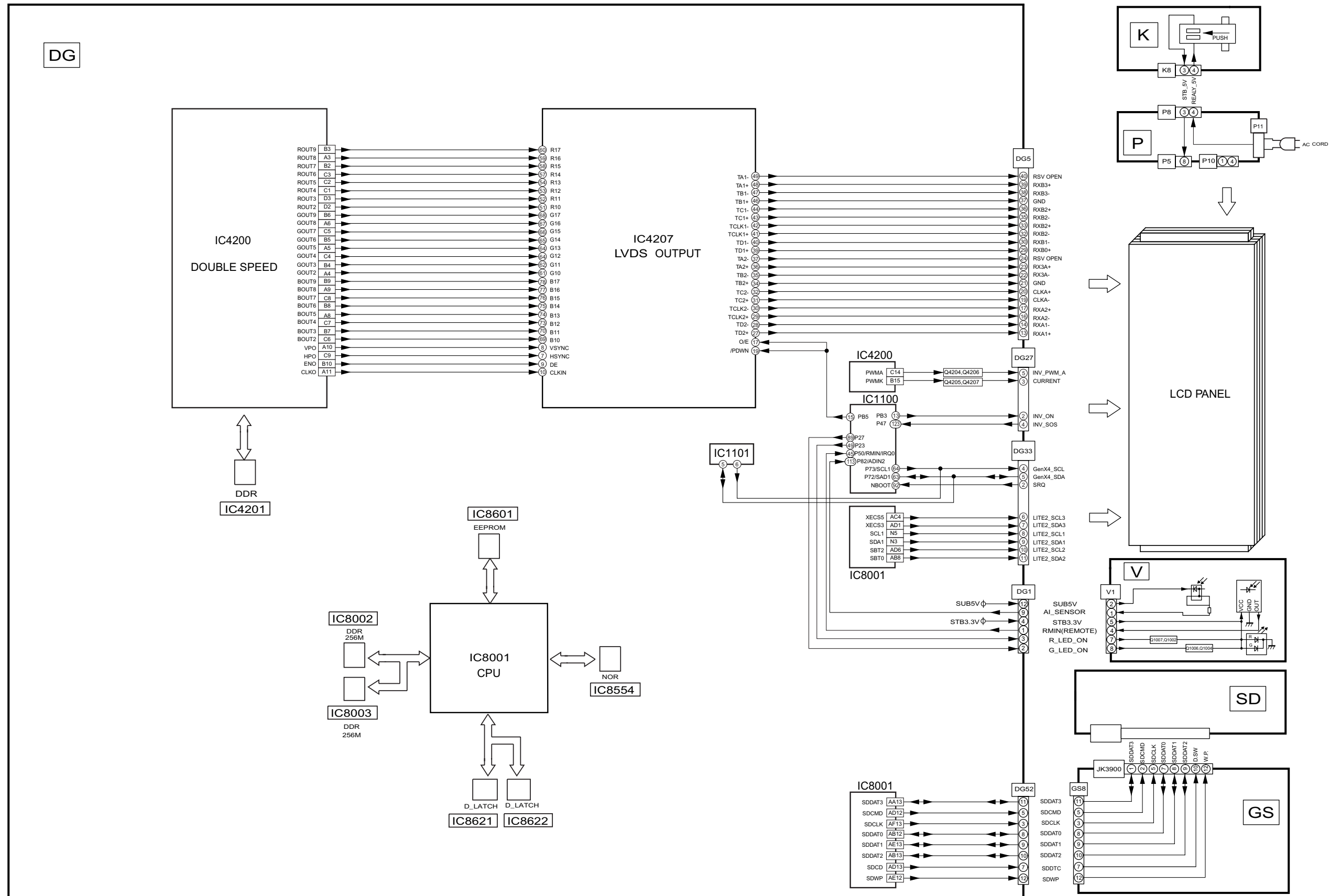
TX-32LX700A/M/X/Y Signal Block Diagram( 3/3 )
