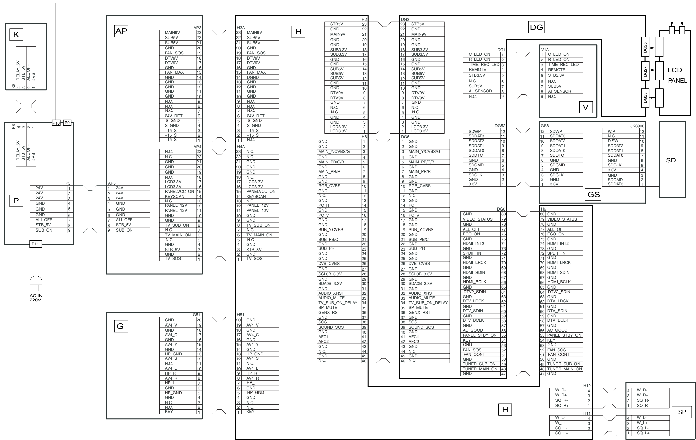
TX-32LX700A/M/X/Y Interconnection Schematic Diagram
