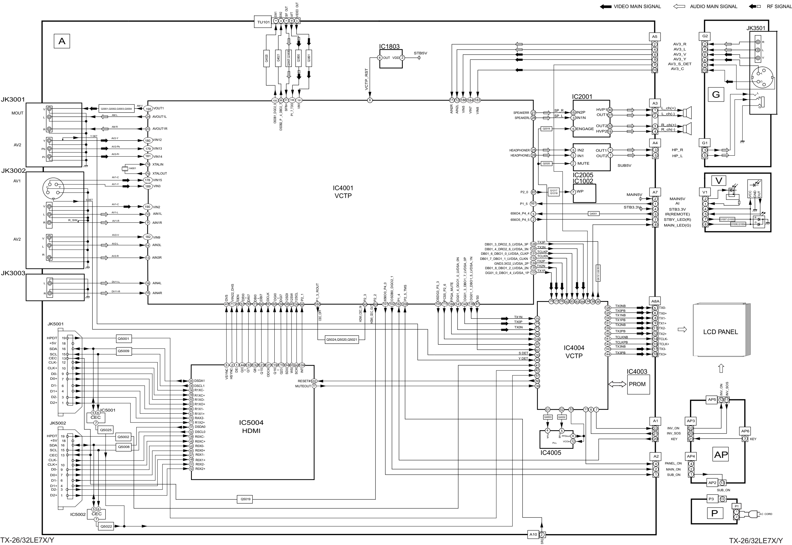
TX-26/32LE7X/Y TX-26/32LX70A/X/Y Signal Block Diagram
