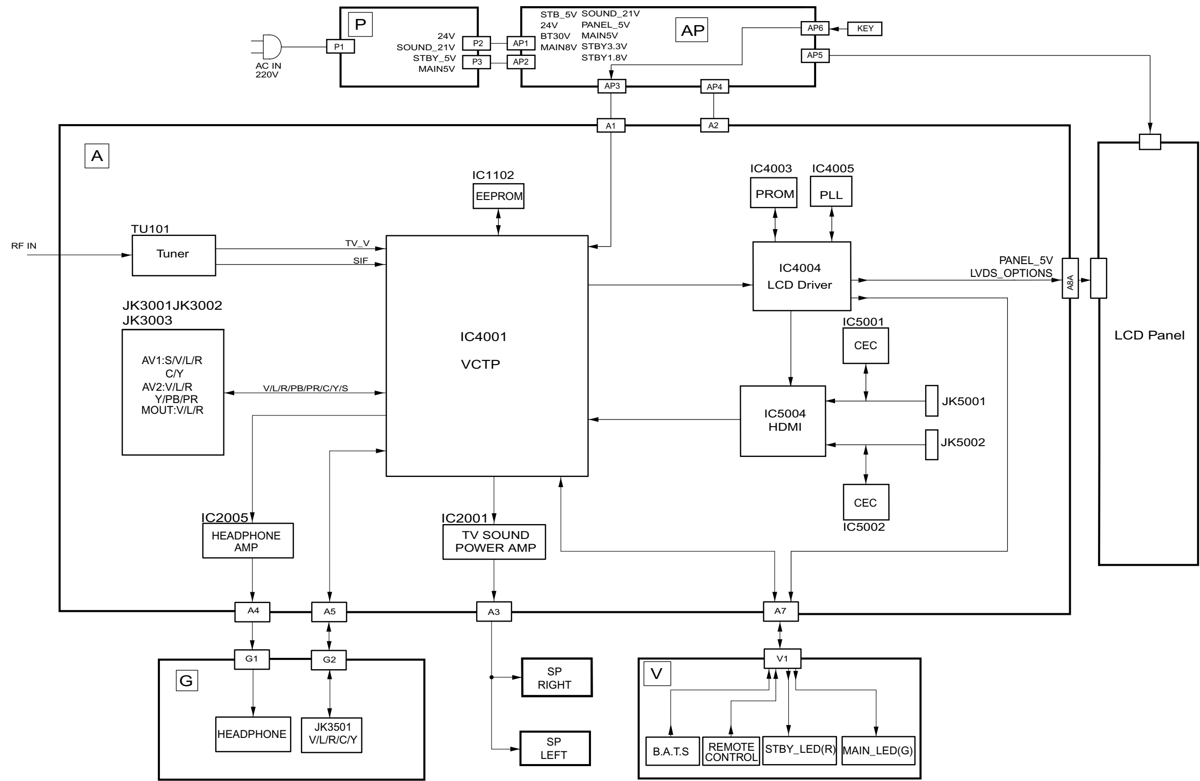
TX-26/32LE7X/Y TX-26/32LX70A/X/Y Main Block Diagram
