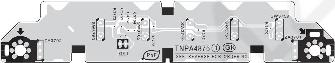
GK-BOARD (FOIL SIDE) TXNGK1EQUC
