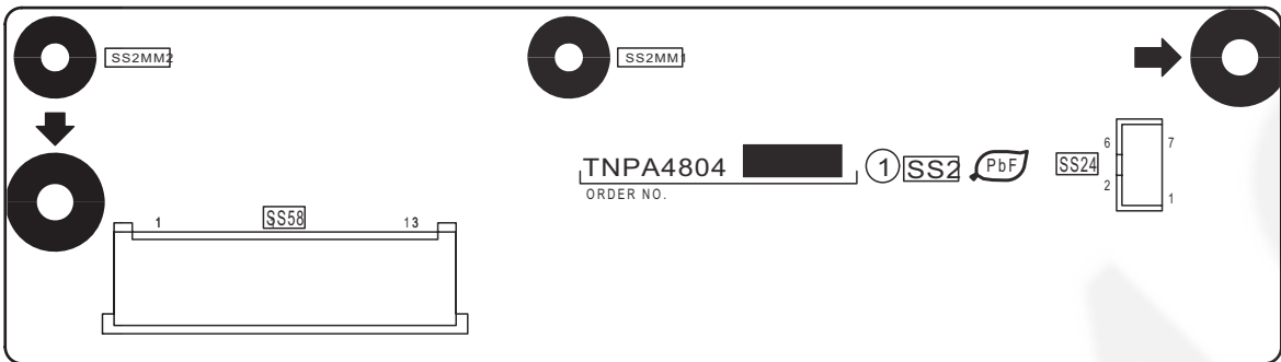
SS2-BOARD (COMPONENT SIDE) TNPA4804
