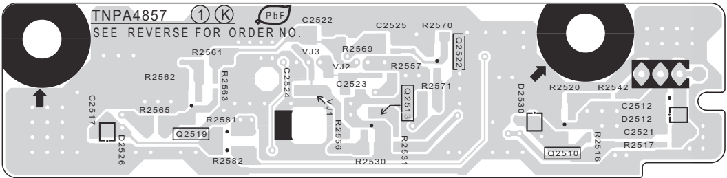
K-BOARD (COMPONENT SIDE) TXN/K1EQUC
