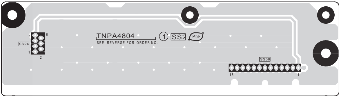
SS2-BOARD (FOIL SIDE) TNPA4804
