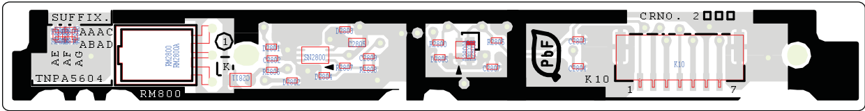
K-BOARD (TOP COMPONENT SIDE) TNPA5604
