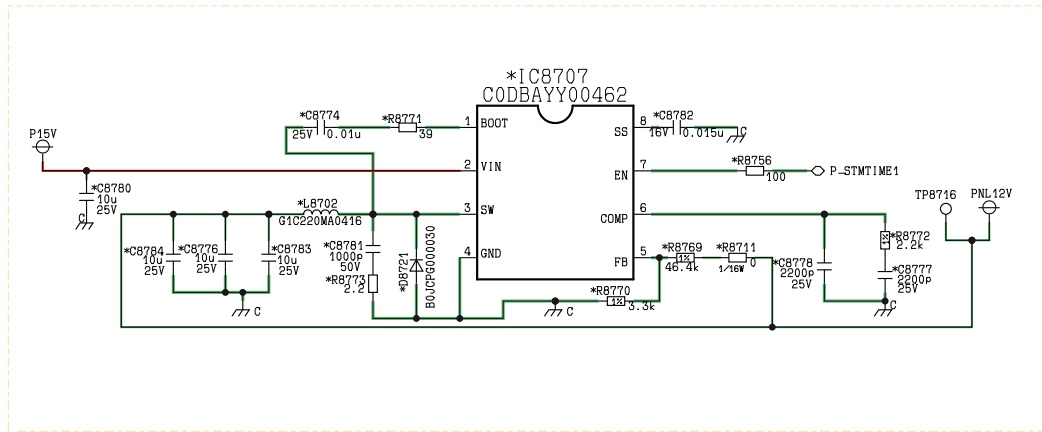
PANEL_DCDC
