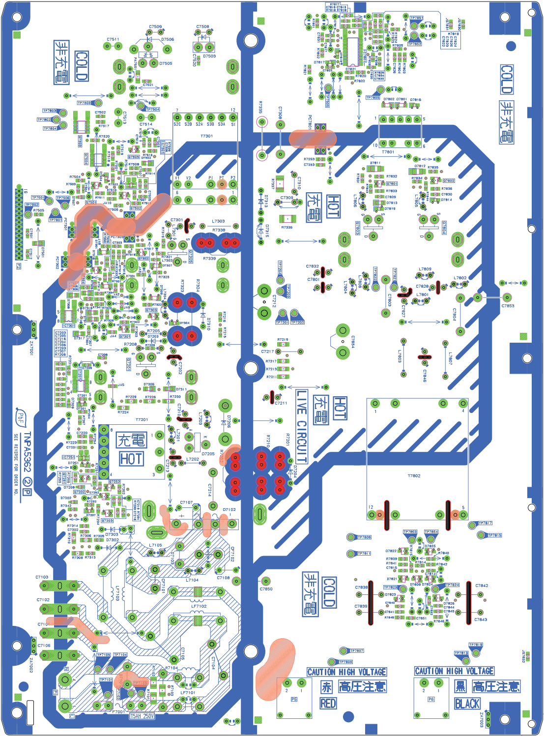
P-BOARD (BOTTOM COMPONENT SIDE) TNPA5362
