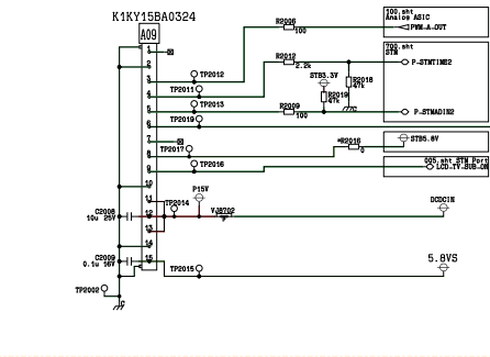
POWER-CONNECTOR
