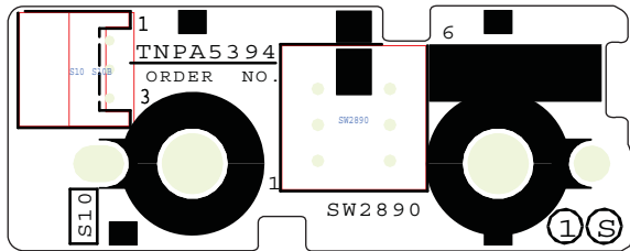
S-BOARD (TOP COMPONENT SIDE) TNPA5394
