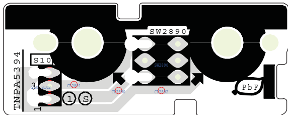
S-BOARD (BOTTOM COMPONENT SIDE) TNPA5394
