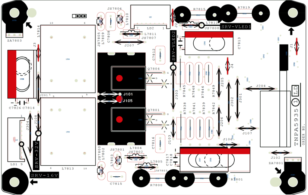
(COMPONENT SIDE)
