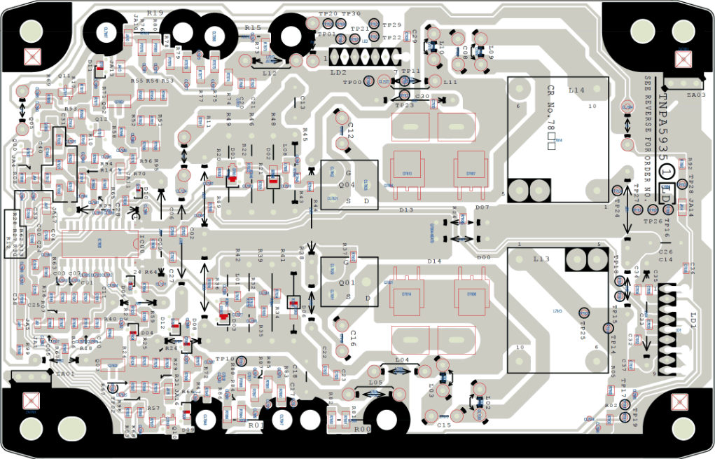
(FOIL SIDE)
