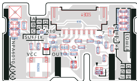
(FOIL SIDE)
