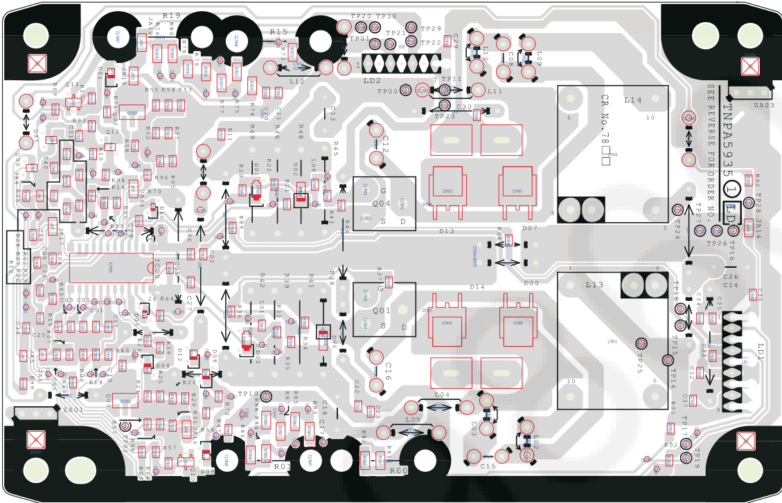
(FOIL SIDE)
