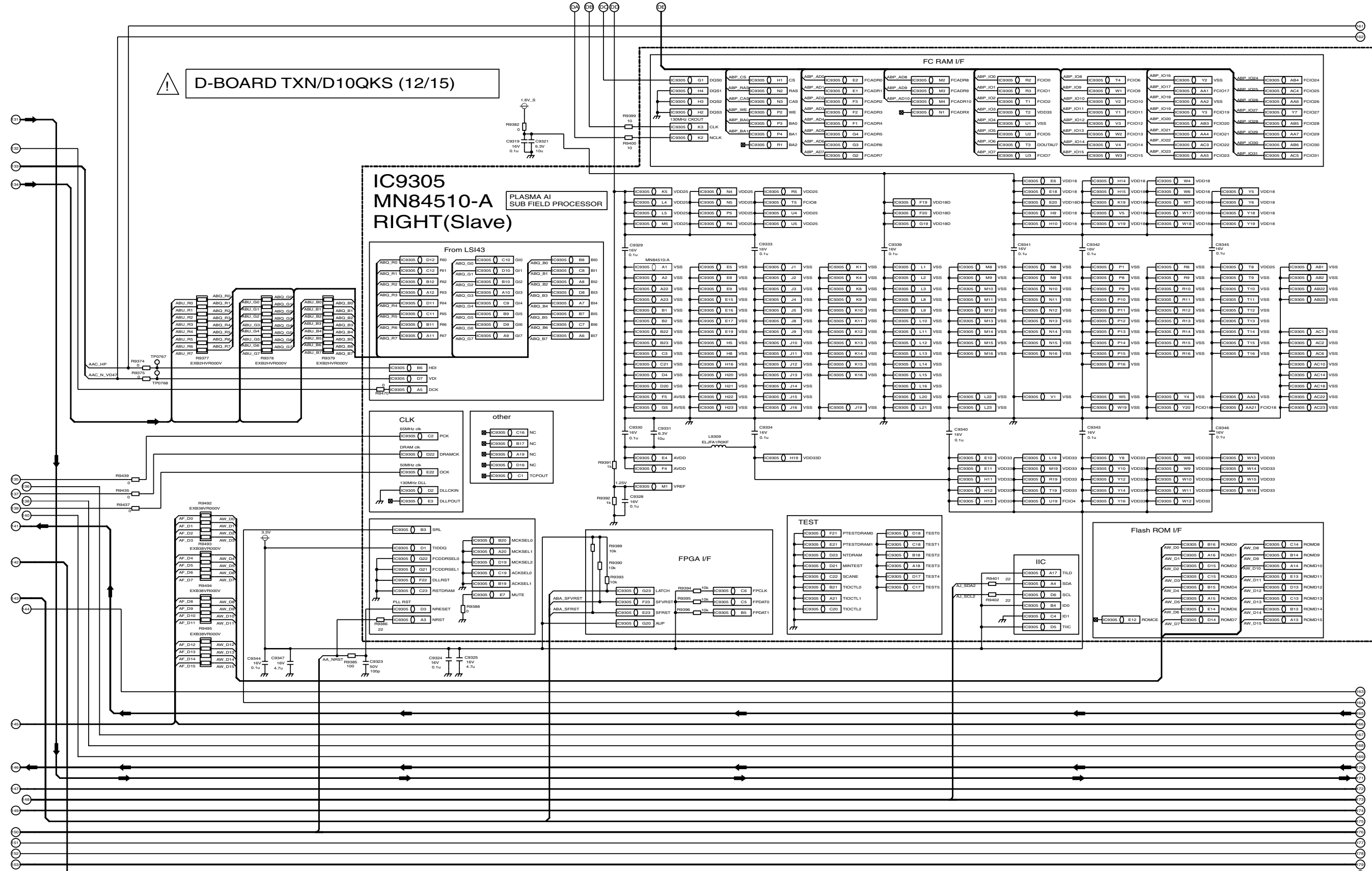
TH-42PX20U-P D-BOARD (12 of 15) Schematic Diagram
