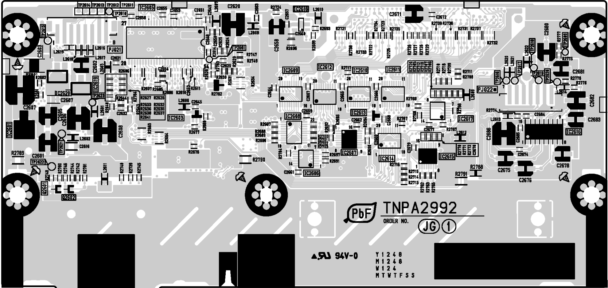
JG-BOARD(COMPONENT SIDE) TNPA2992
