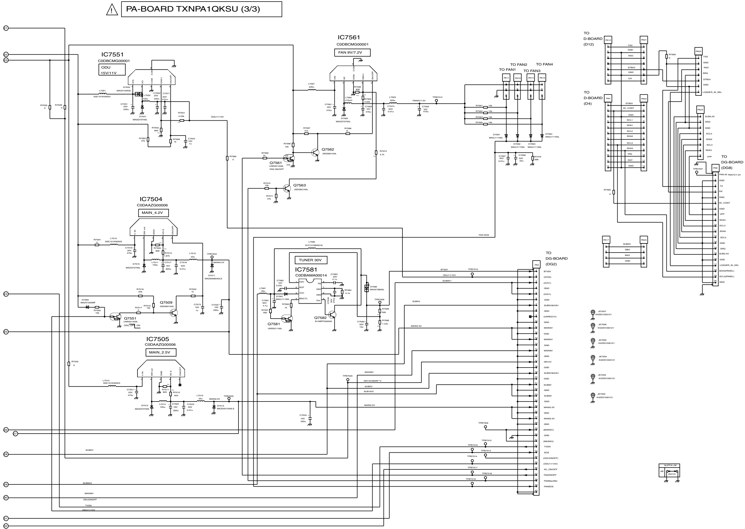
TH-42PX20U-P PA-BOARD (3 of 3) Schematic Diagram
