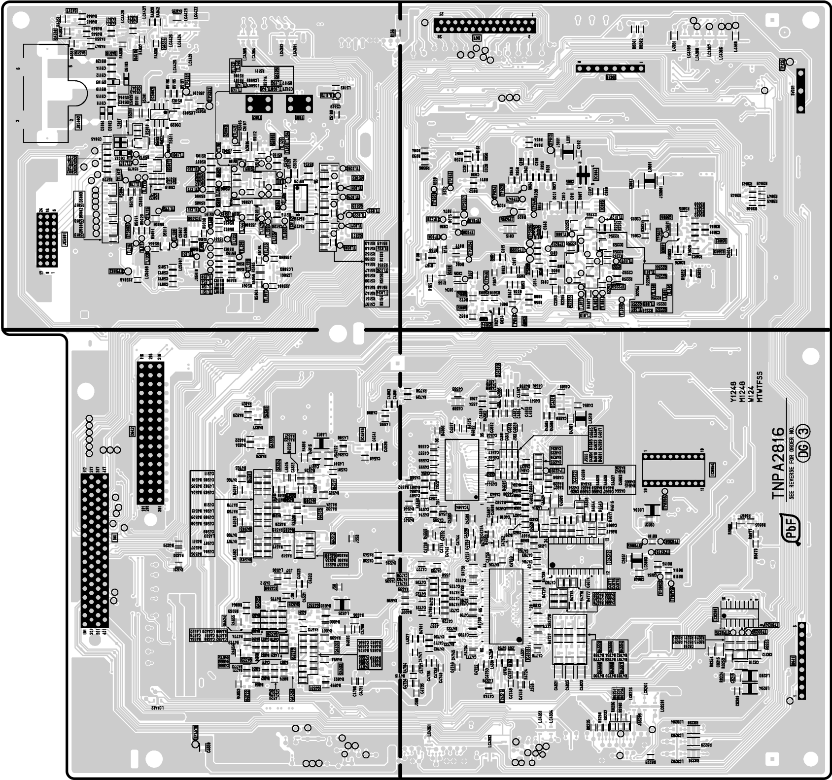
TH-42PX20U-P DG-BOARD TNPA2816AB
