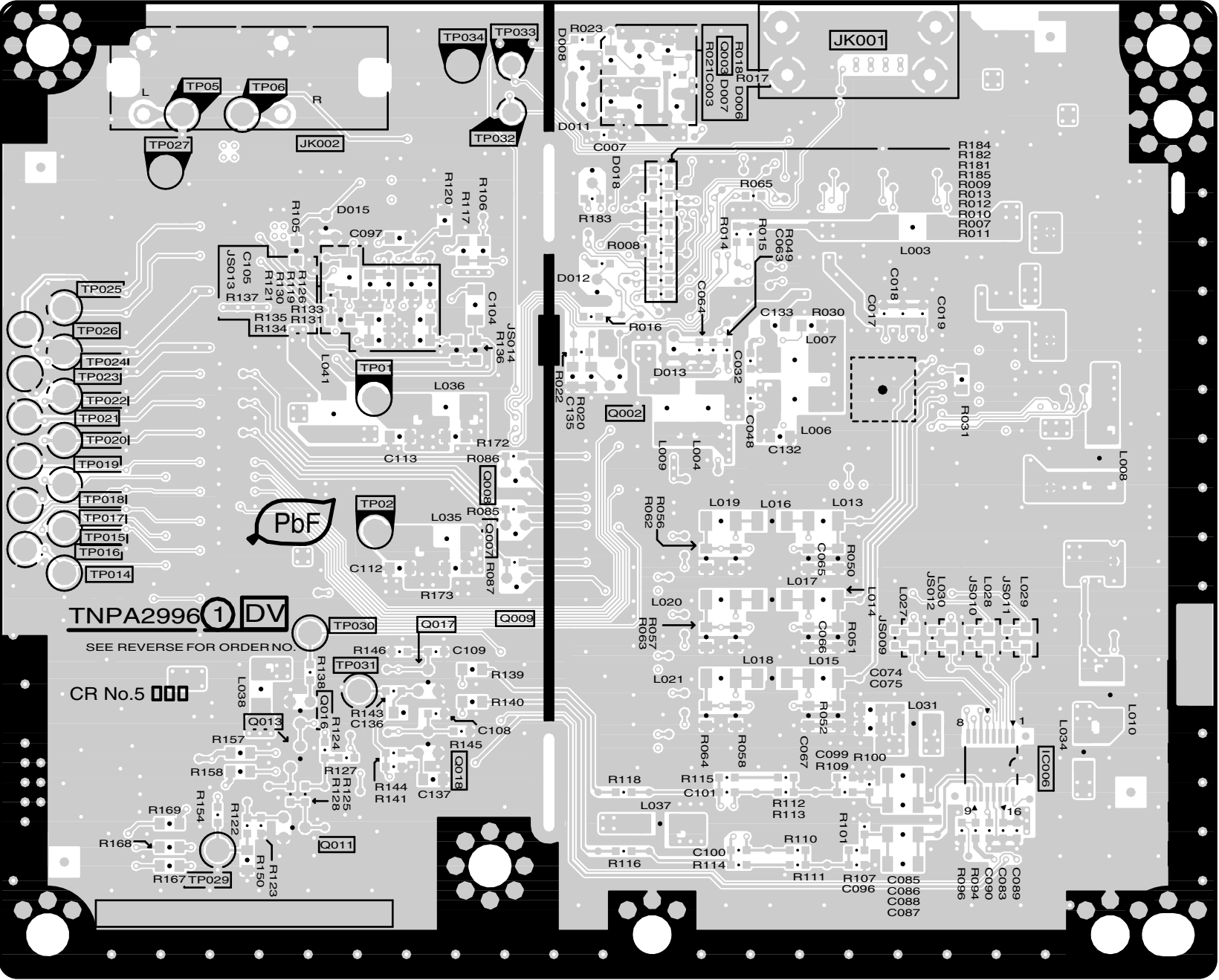
DV-BOARD(FOIL SIDE) TNPA2996AC
