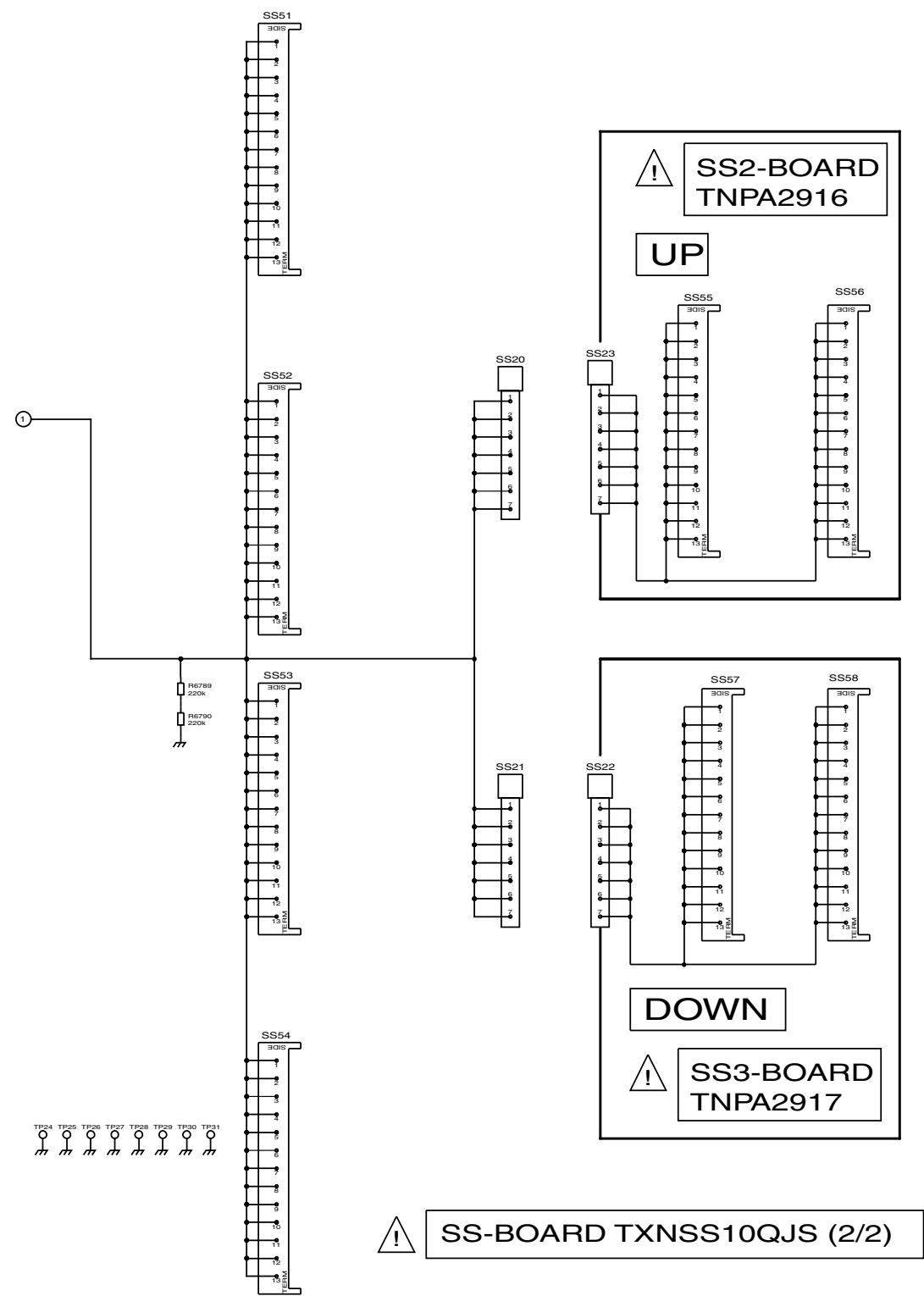
TH-42PX20U-P SS (2 of 2), SS2, and SS3-BOARD Schematic Diagram
