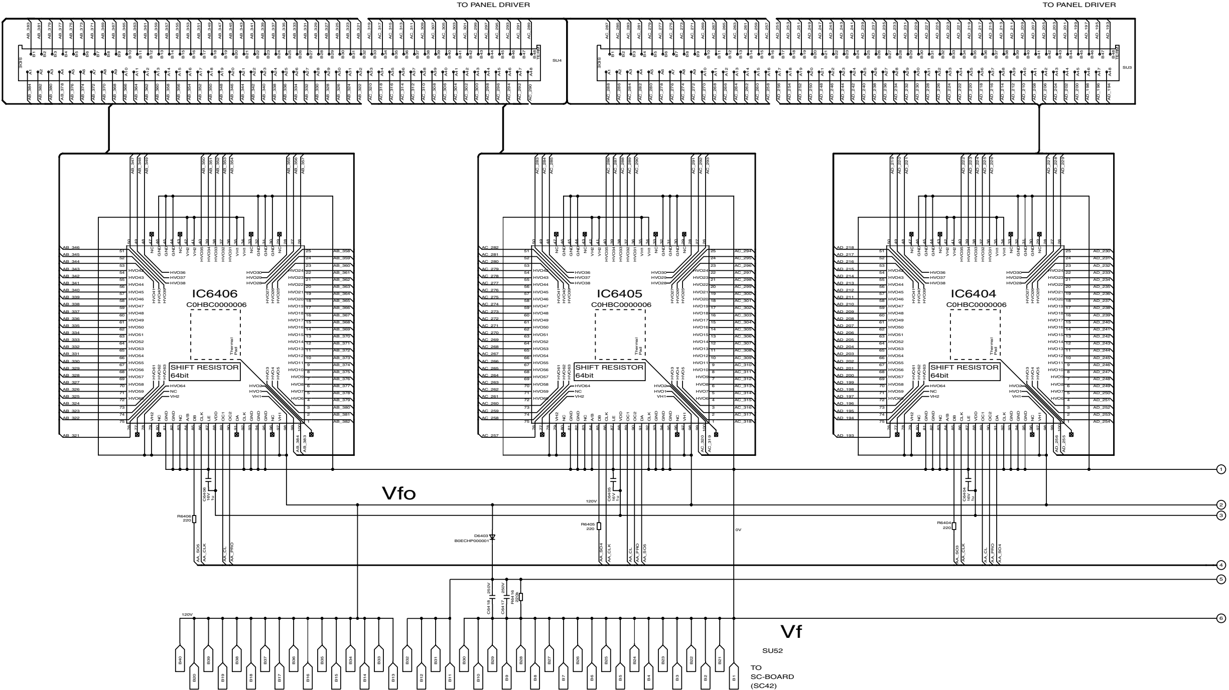
TH-42PX20U-P SU-BOARD (1 of 2) Schematic Diagram
