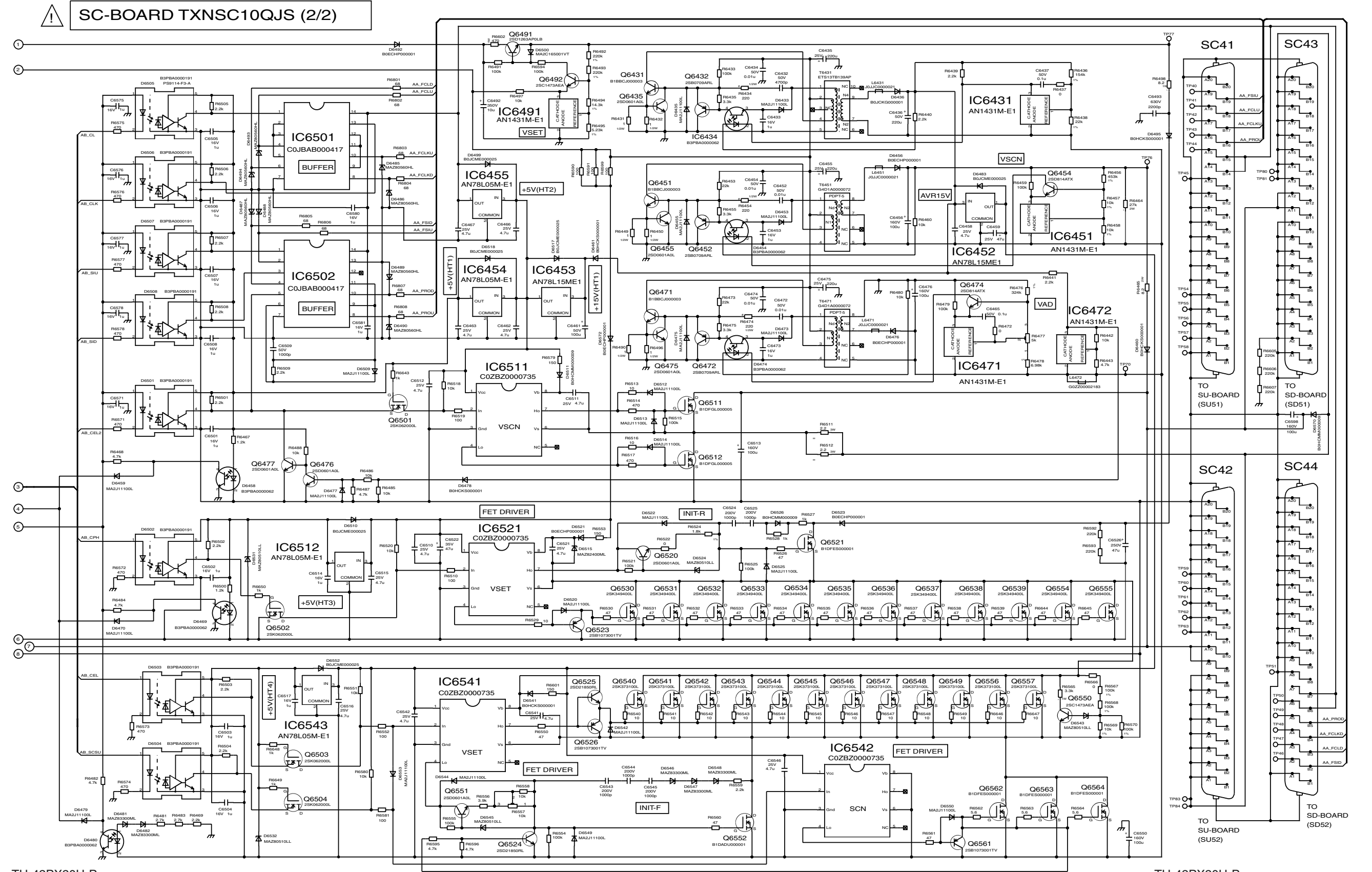
TH-42PX20U-P SC-BOARD (2 of 2) Schematic Diagram
