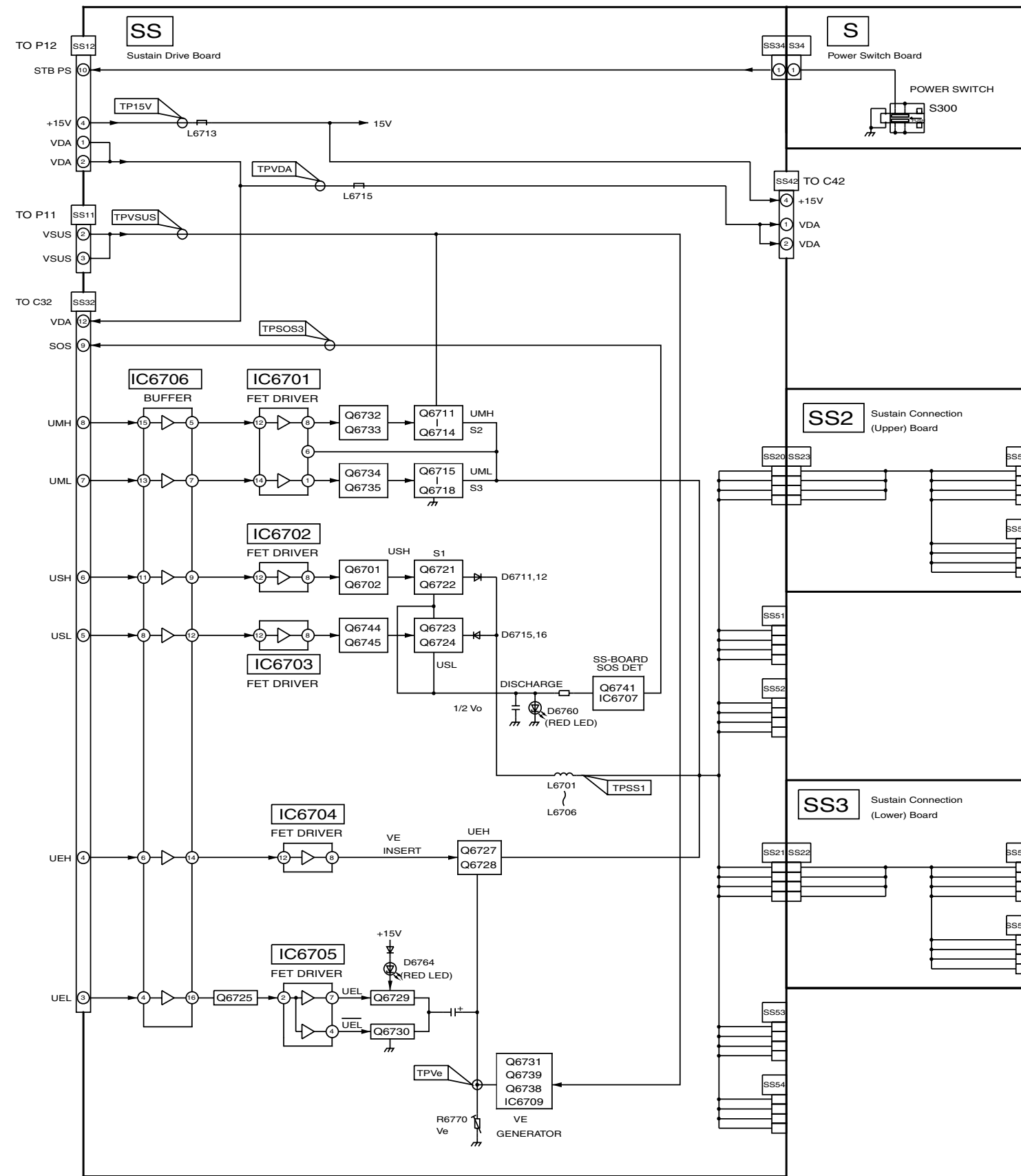
TH-42PX20U-P SS, S, SS2 and SS3-BOARD BLOCK Diagram
