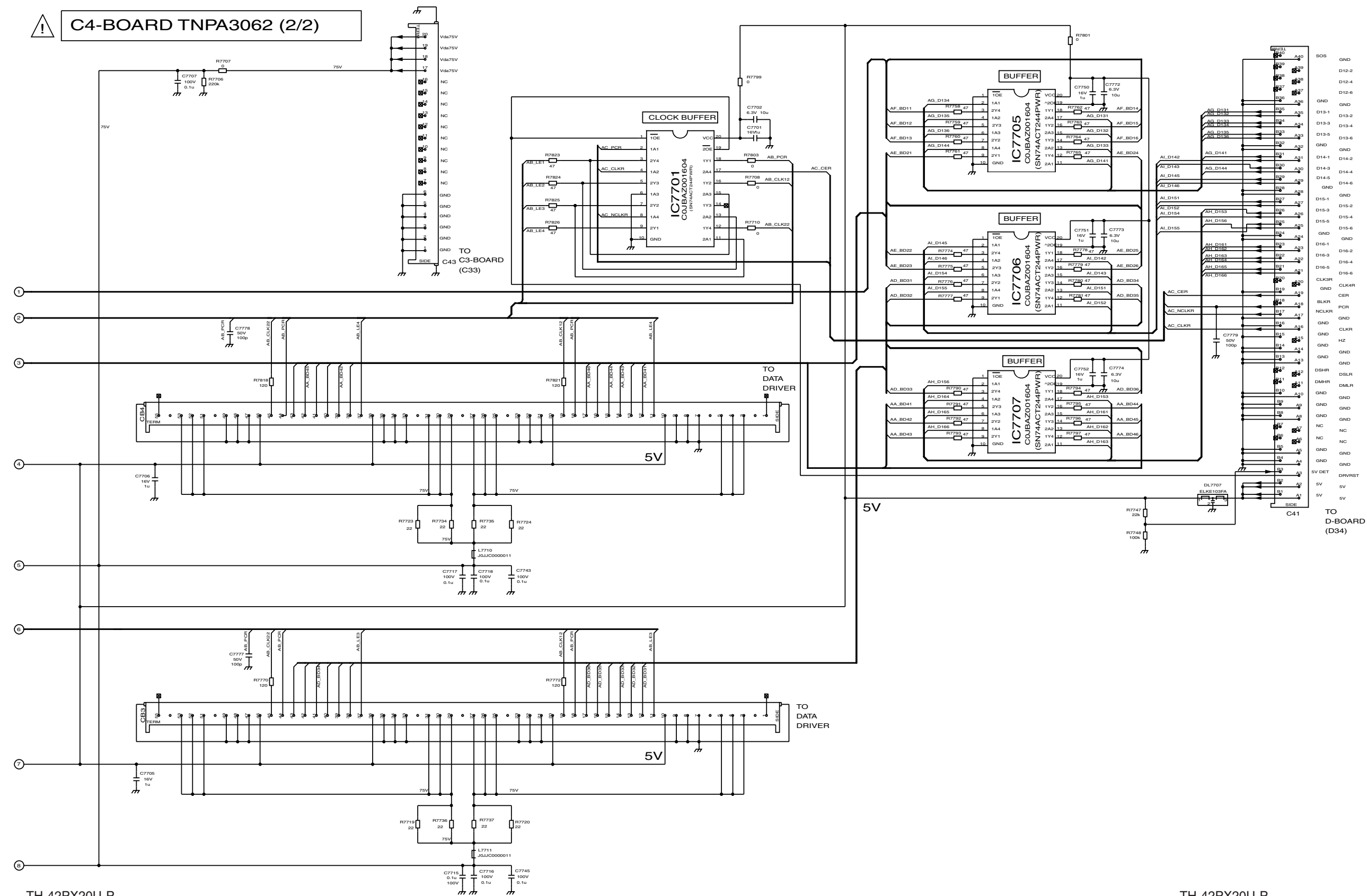
TH-42PX20U-P C4-BOARD (2 of 2) Schematic Diagram
