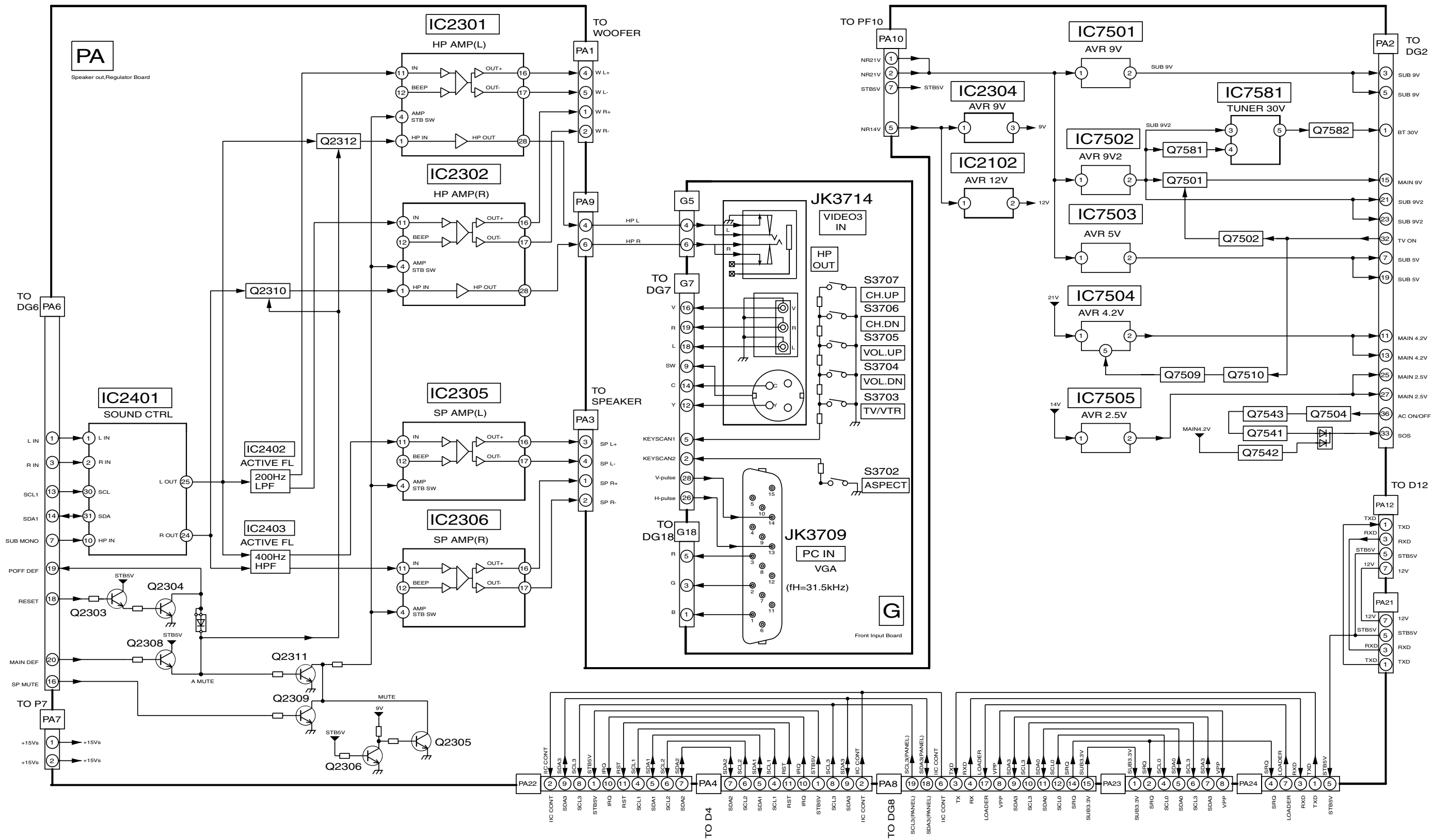
TH-42PX20U-P PA and G-BOARD BLOCK Diagram
