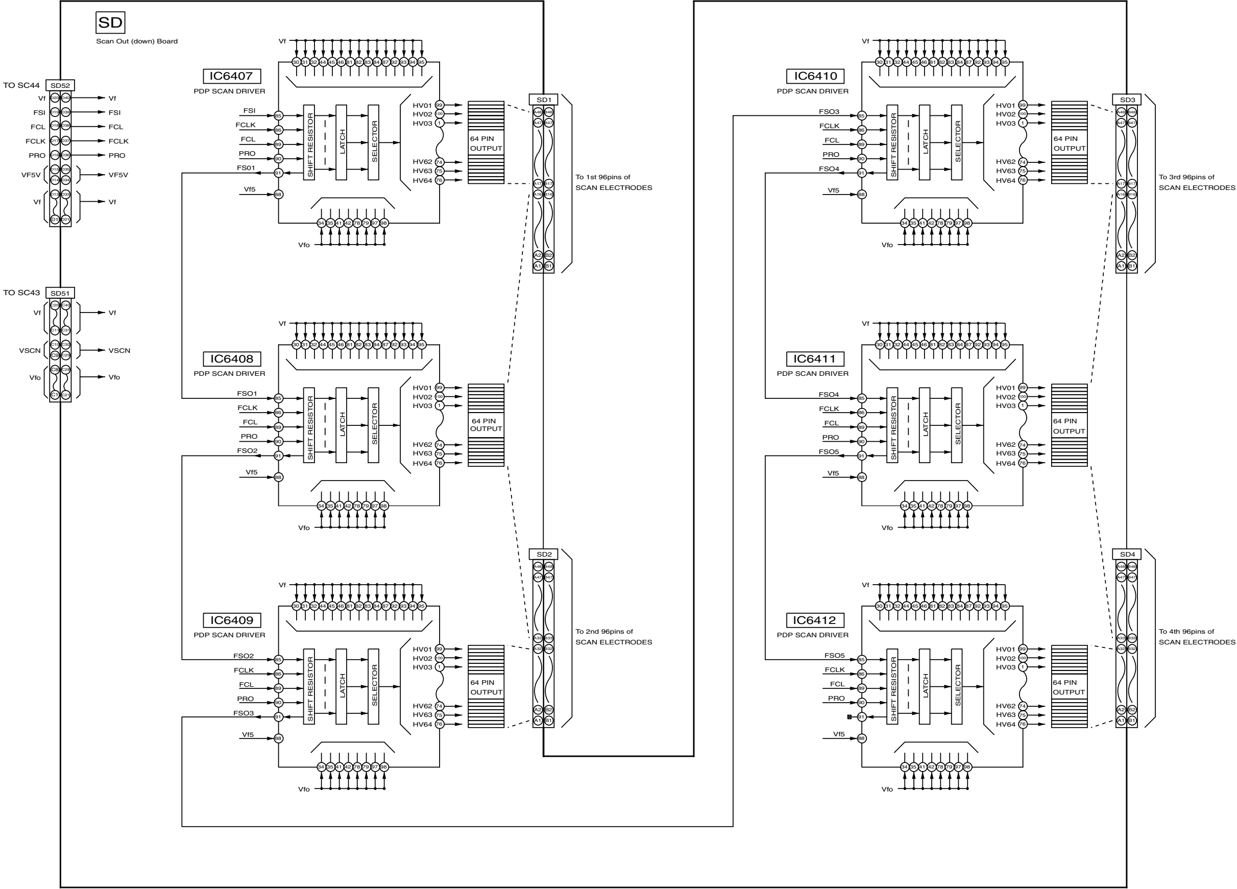
TH-42PX20U-P SD-BOARD BLOCK Diagram
