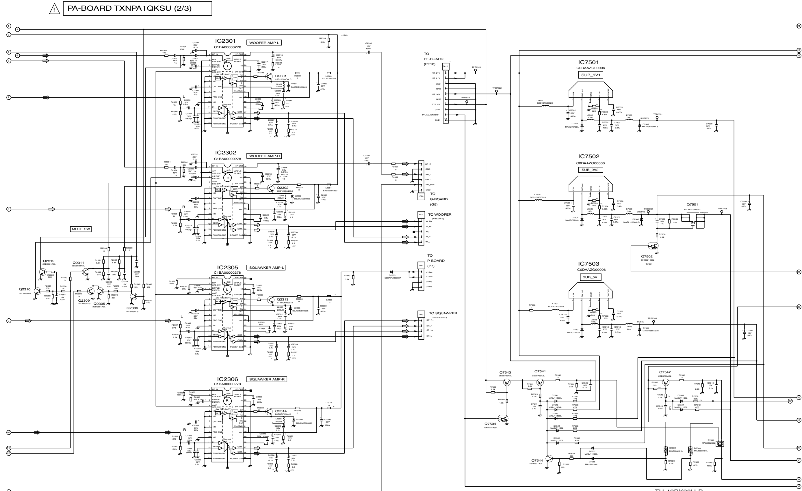
TH-42PX20U-P PA-BOARD (2 of 3) Schematic Diagram
