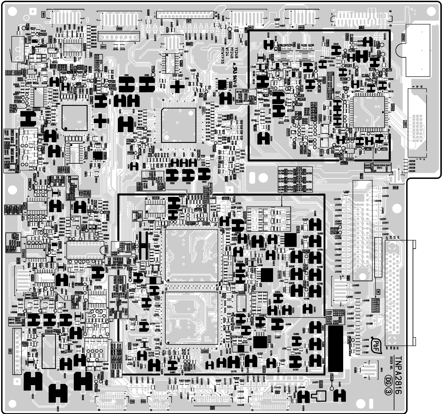
TH-42PX20U-P DG-BD(BOARD) TNPA2816AB
