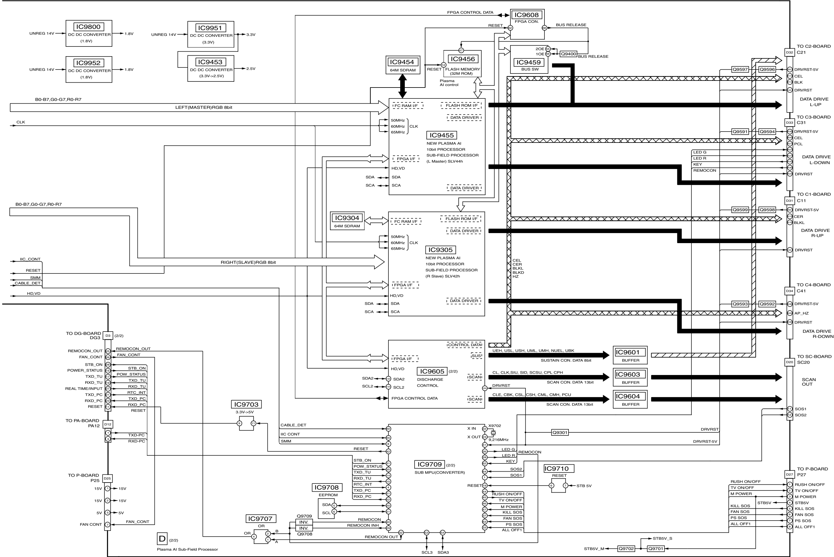
TH-42PX20U-P D-BOARD (2 of 2) BLOCK Diagram
