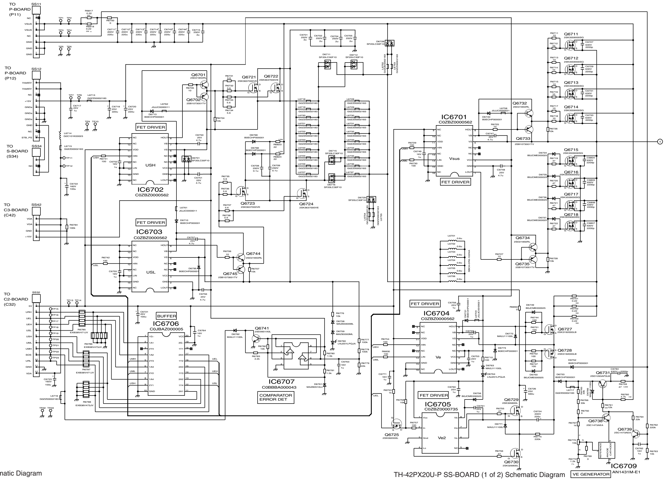
TH-42PX20U-P SS-BOARD (1 of 2) Schematic Diagram
