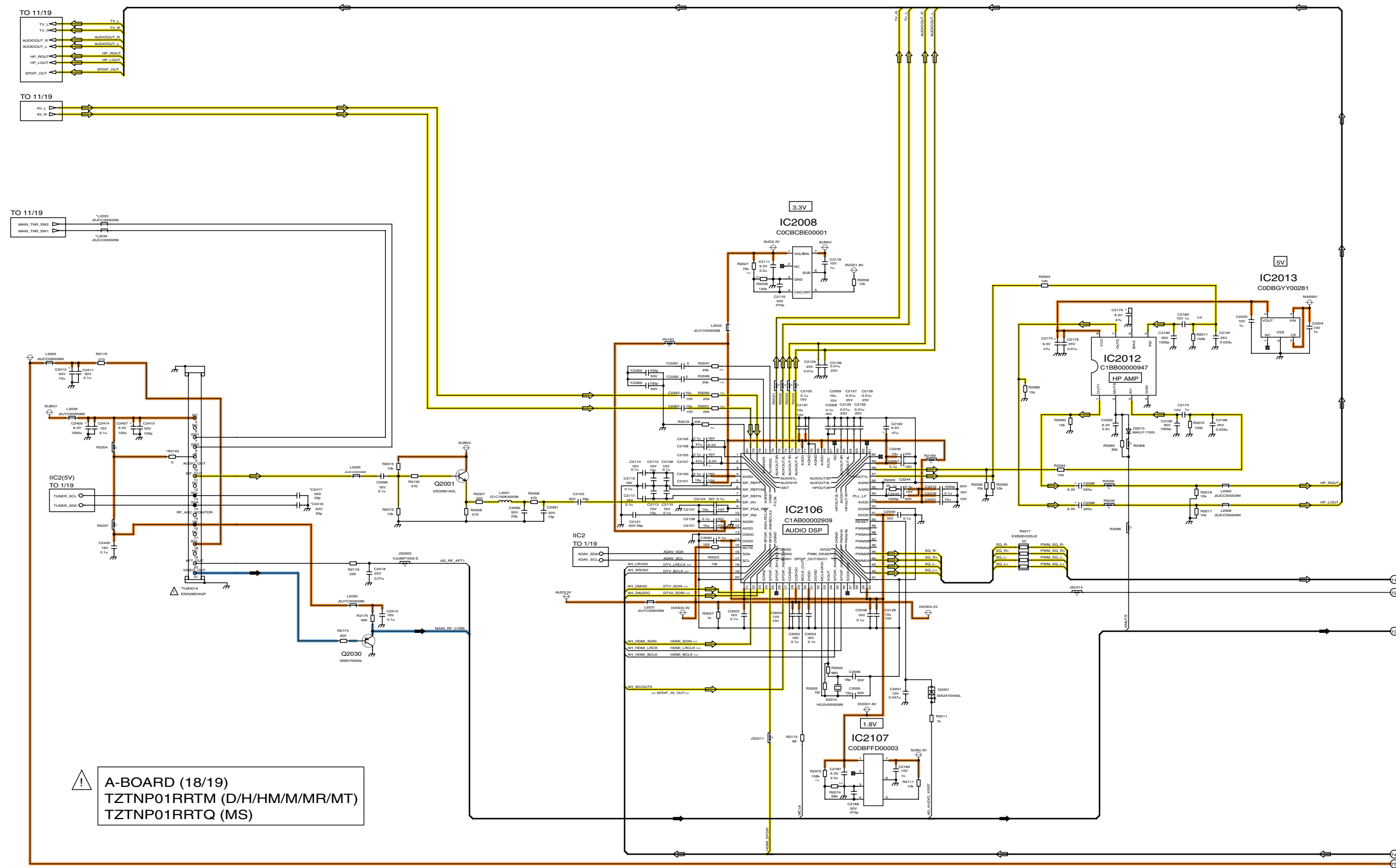
TH-42PV80D/H/HM/M/MR/MS/MT A-Board (18/19) Schematic Diagram
