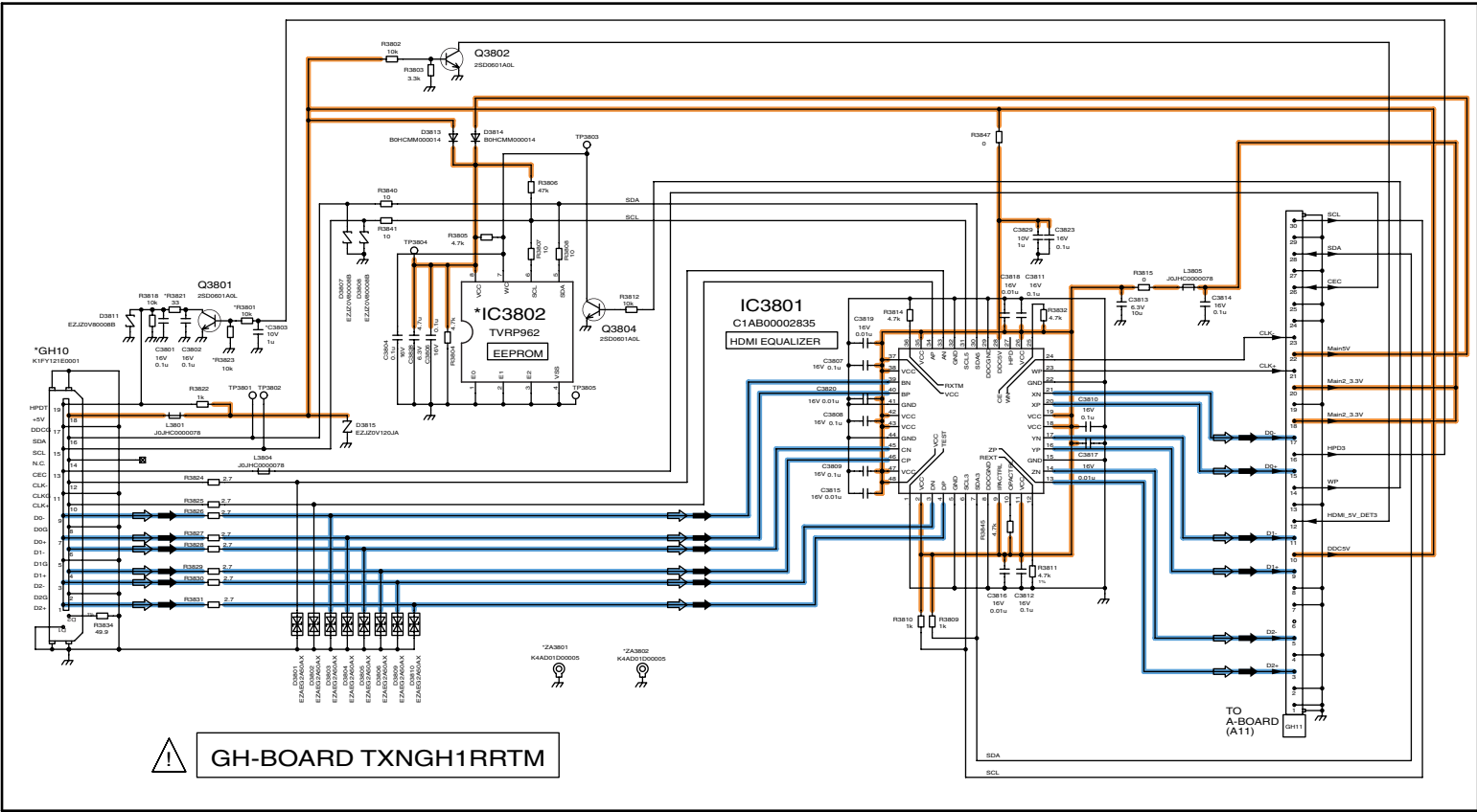
TH-42PV80D/H/HM/M/MR/MS/MT G, GH, GS, and K-Board Schematic Diagram
