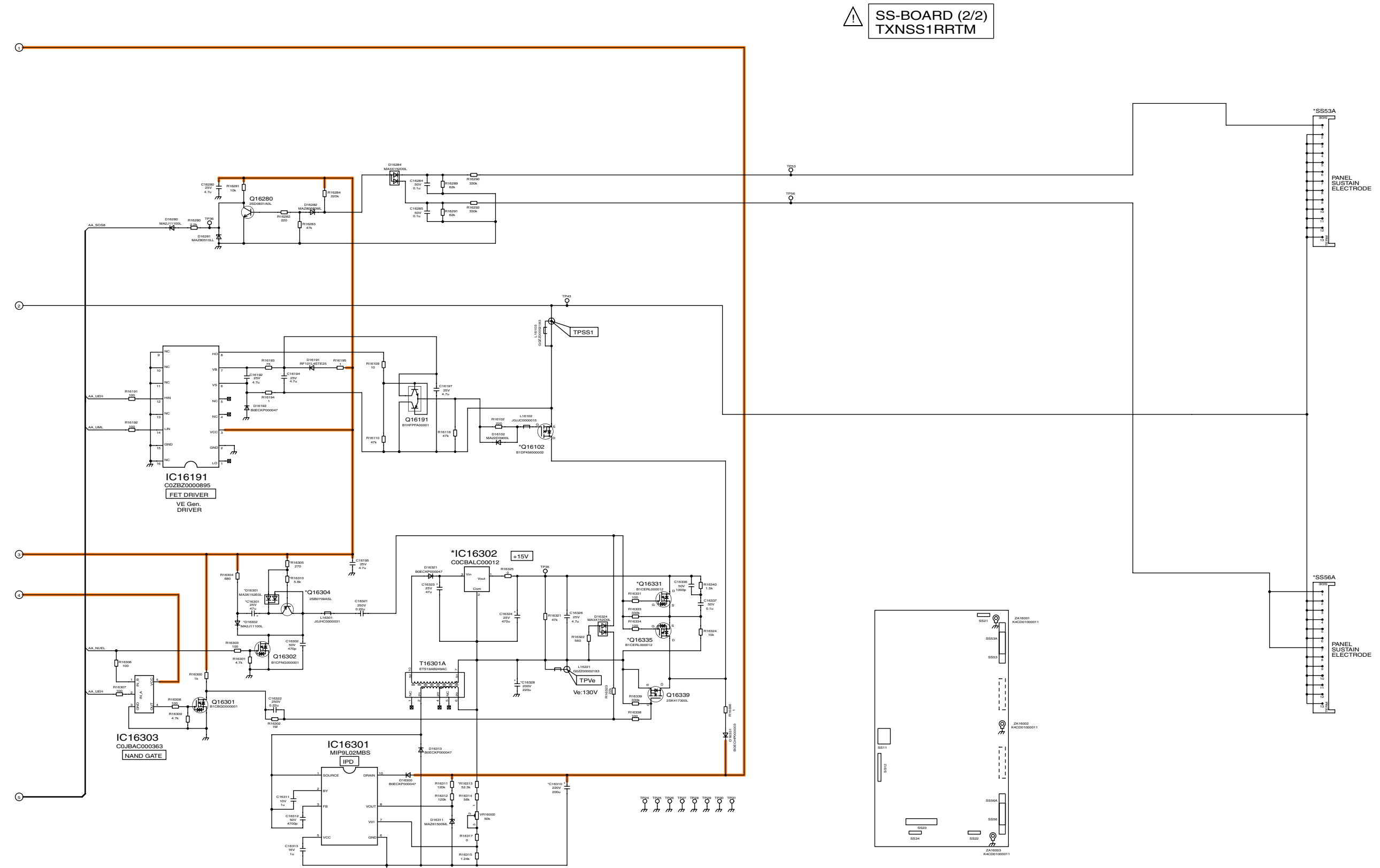
TH-42PV80D/H/HM/M/MR/MS/MT SS-Board (2/2) Schematic Diagram
