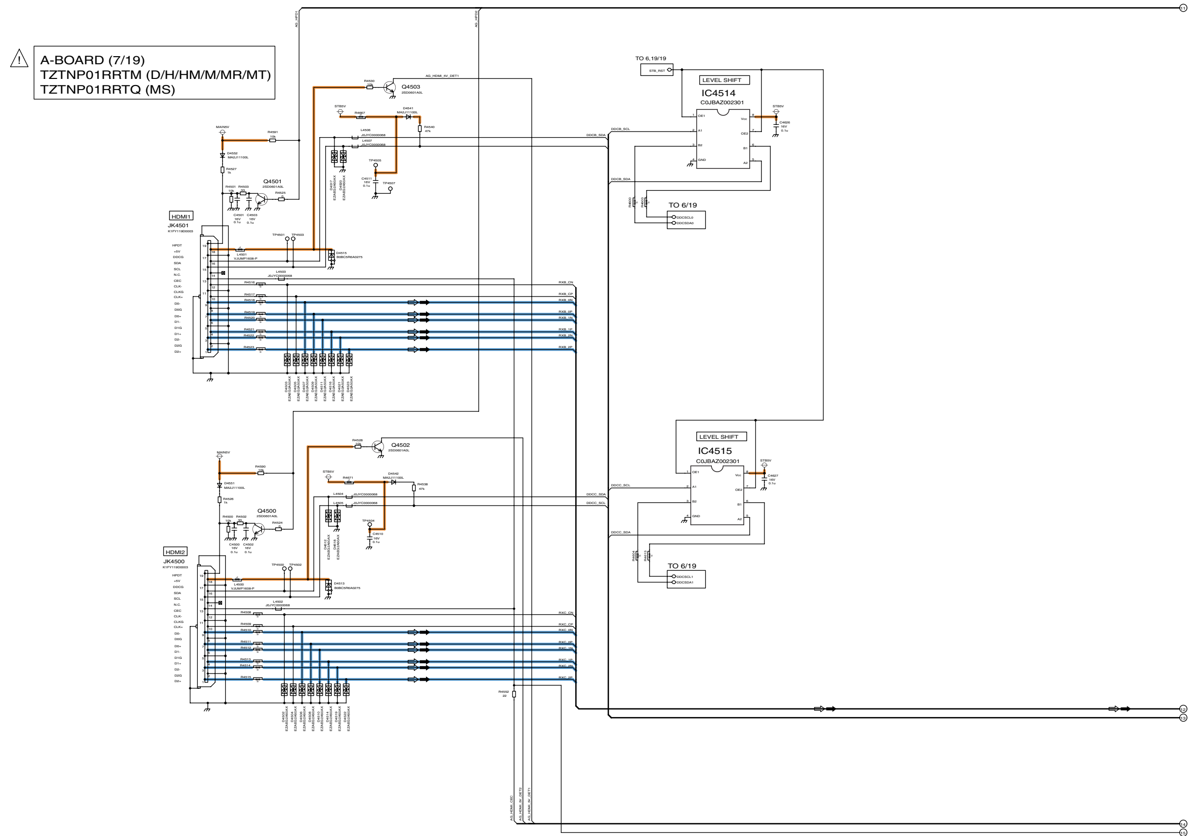
TH-42PV80D/H/HM/M/MR/MS/MT A-Board (7/19) Schematic Diagram
