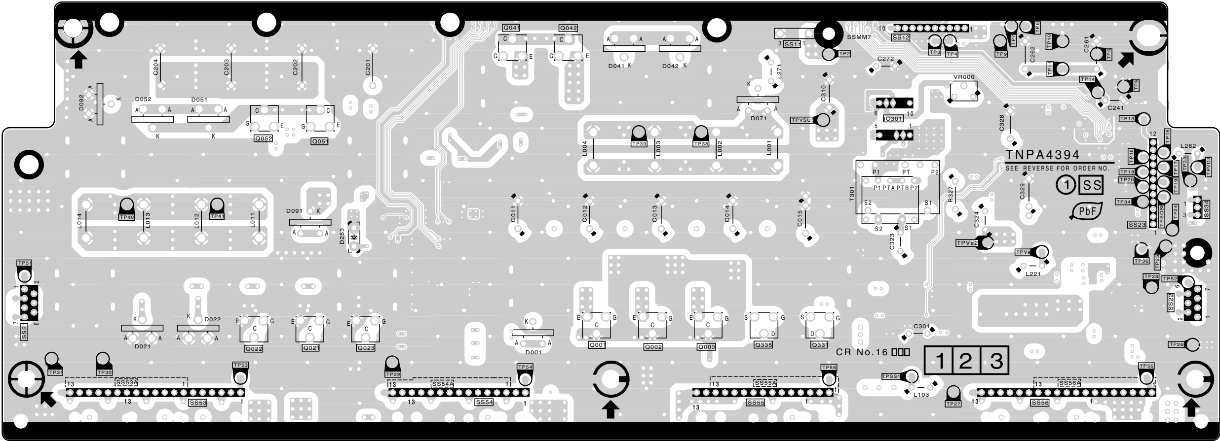
TH-42PV80D/H/HM/M/MR/MS/MT SS-BOARD TXNSS1RRTM
