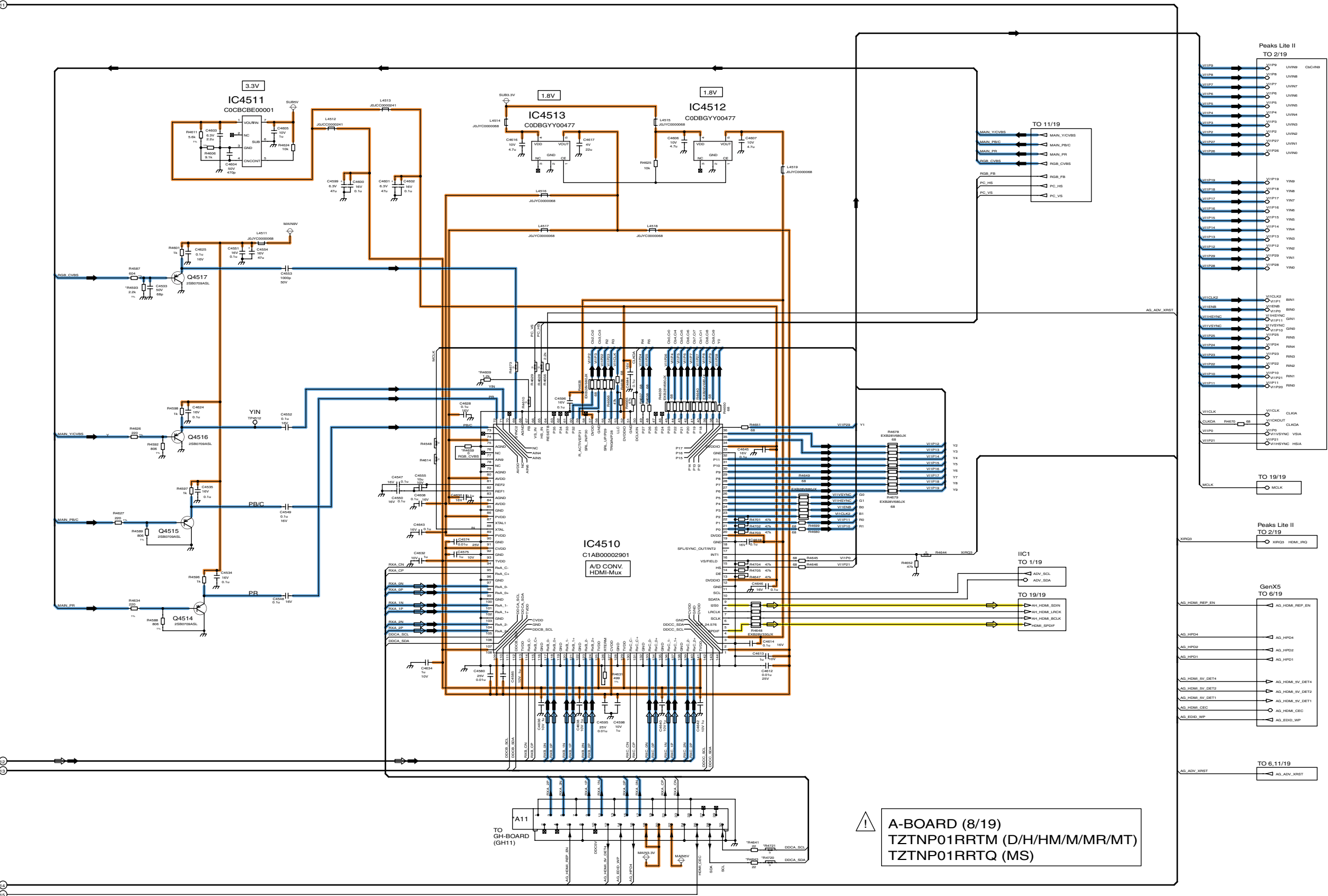
TH-42PV80D/H/HM/M/MR/MS/MT A-Board (8/19) Schematic Diagram
