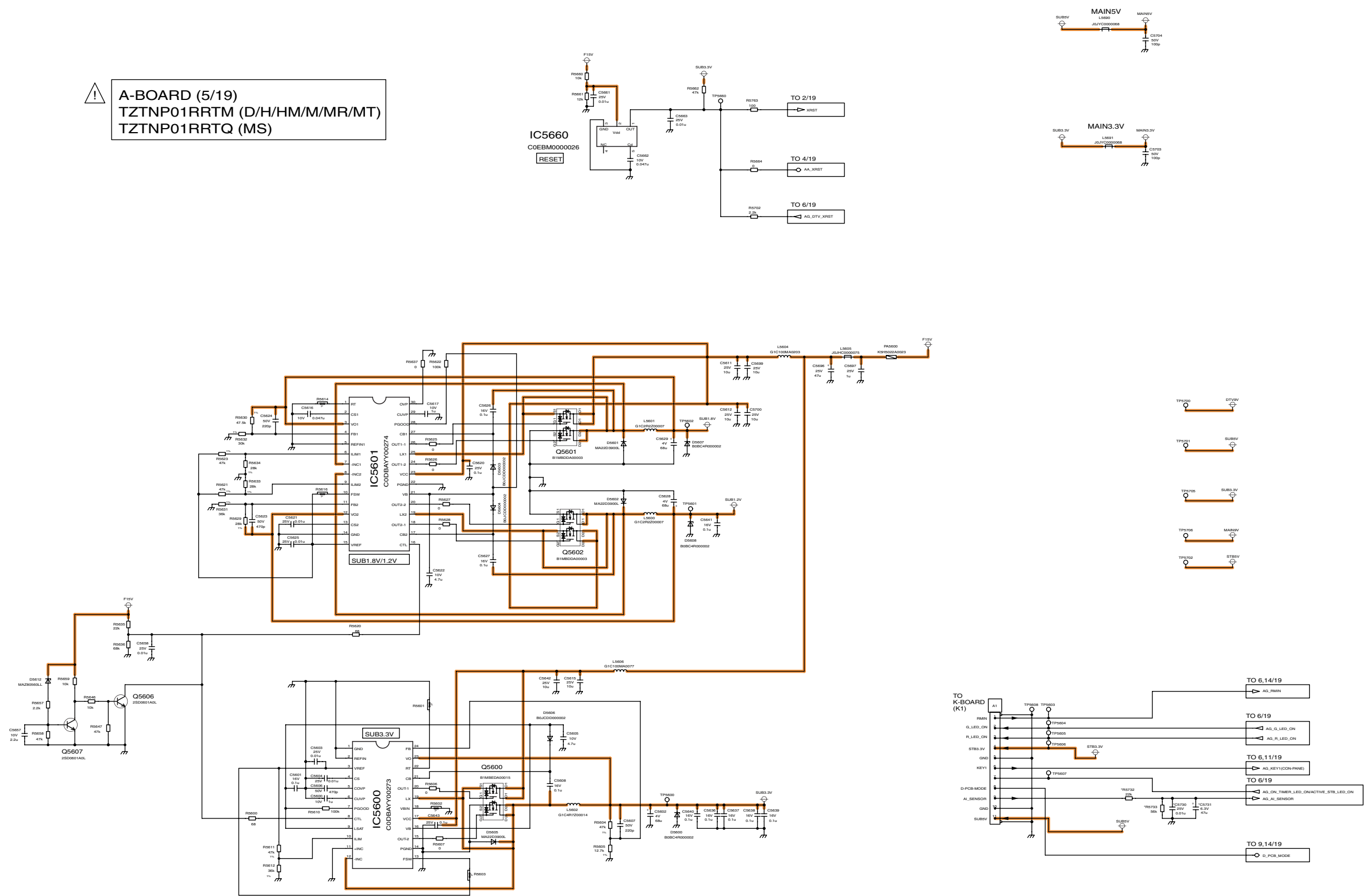
TH-42PV80D/H/HM/M/MR/MS/MT A-Board (5/19) Schematic Diagram
