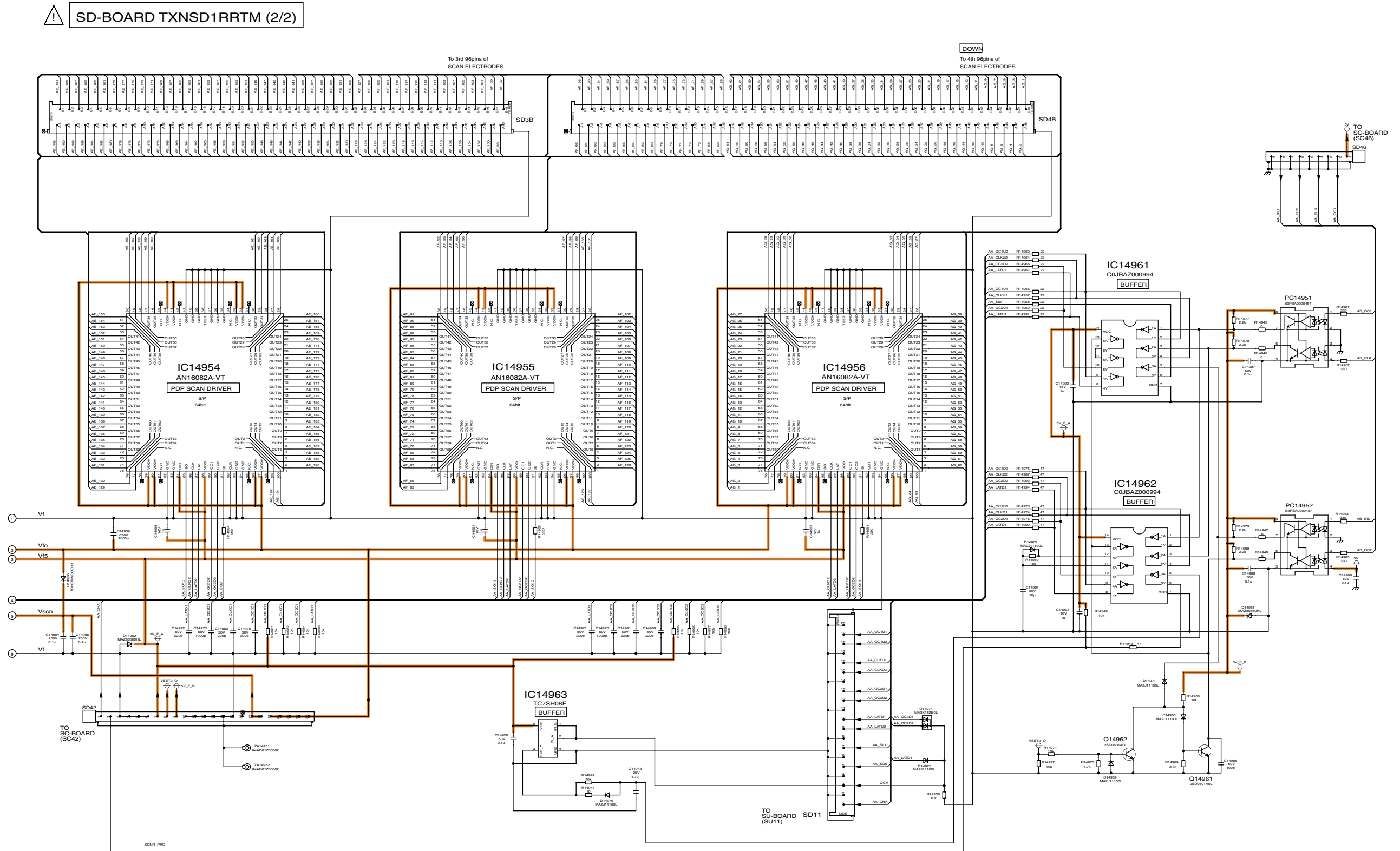
TH-42PV80D/H/HM/M/MR/MS/MT SD-Board (2/2) Schematic Diagram
