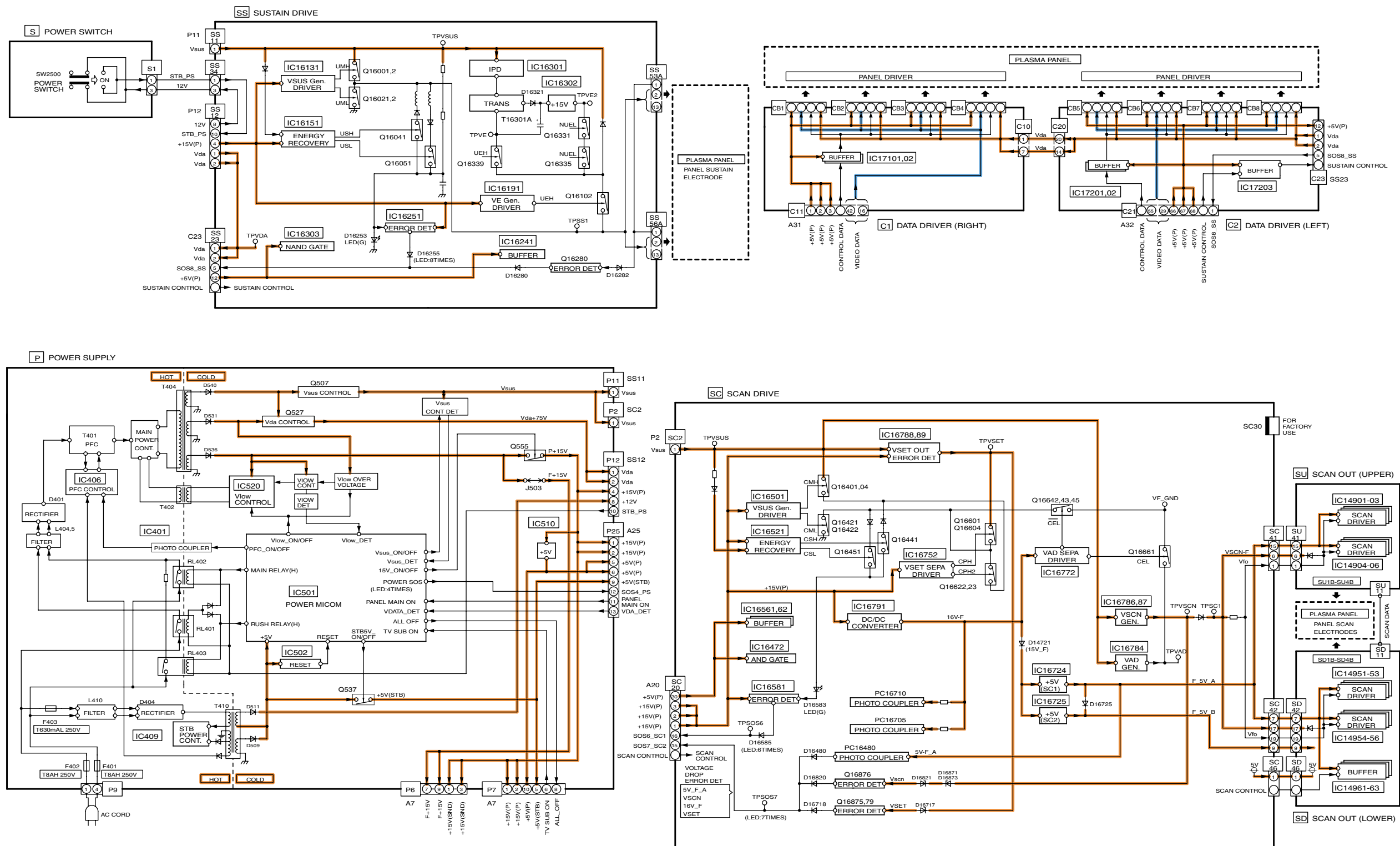
TH-42PV80D/H/HM/M/MR/MS/MT Block (5/5) Diagram
