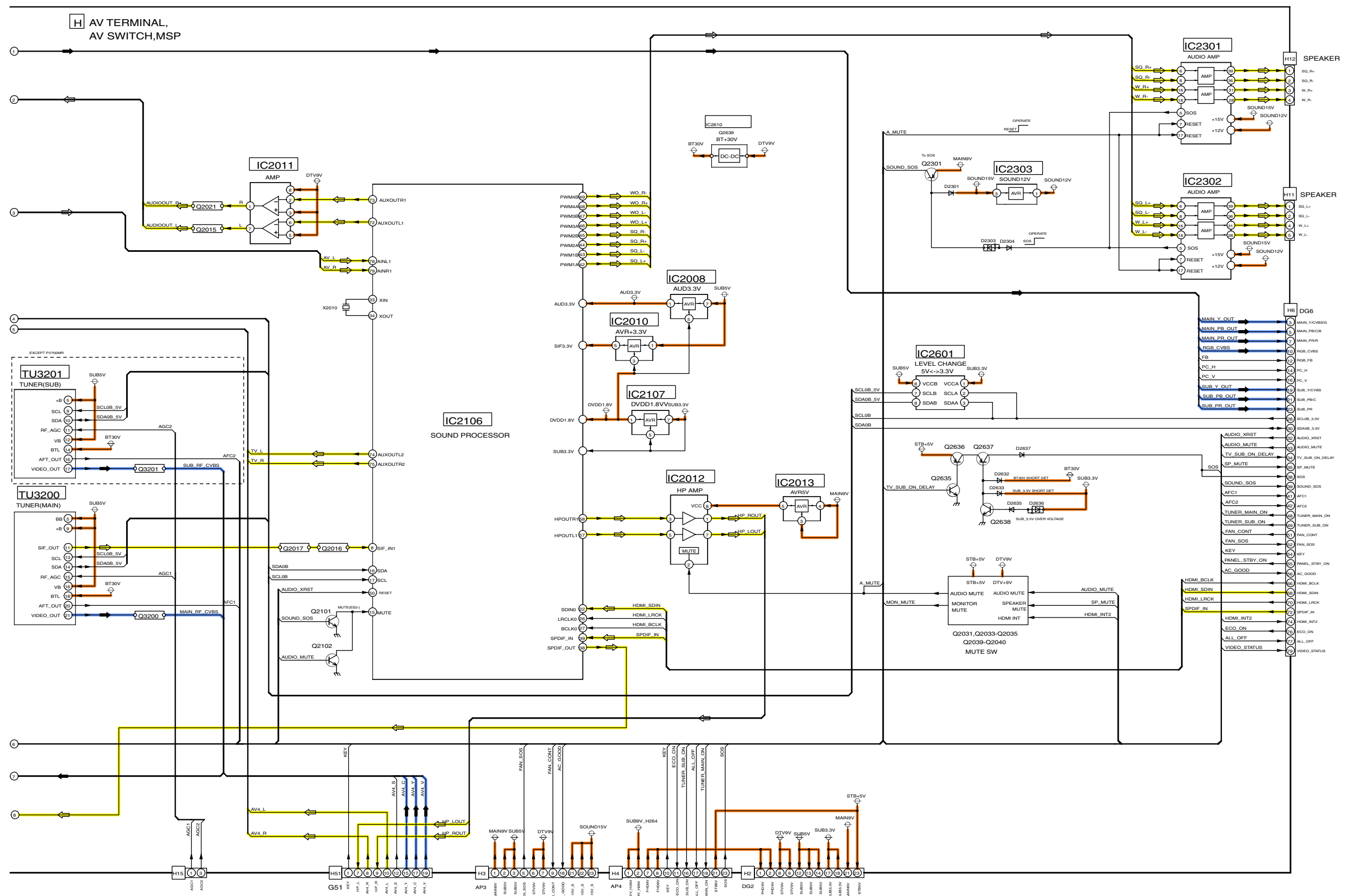
TH-42PV700AZ/H/M/MR/MT H-Board (2 of 2) Block Diagram
