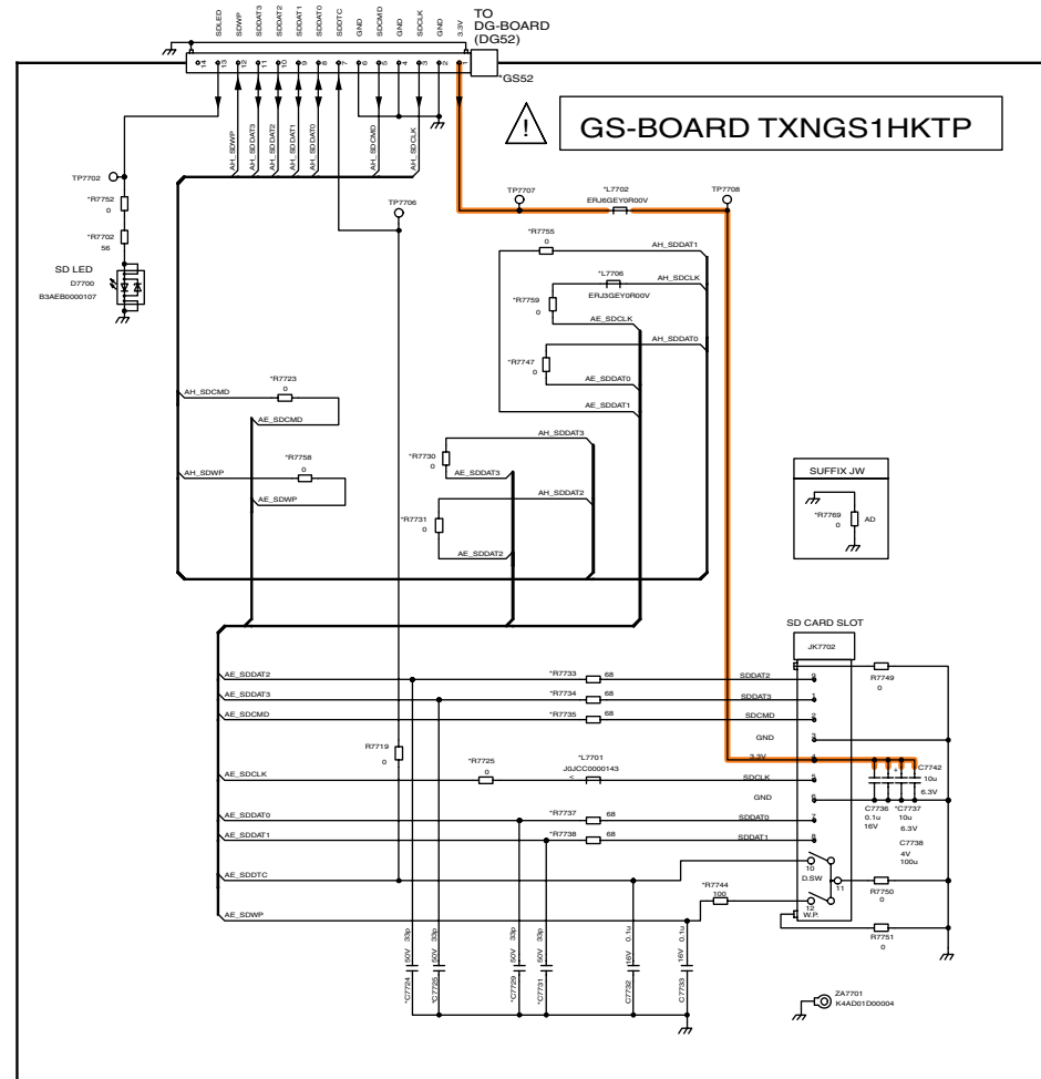
TH-42PV700AZ/H/M/MR/MT G and GS-Board Schematic Diagram
