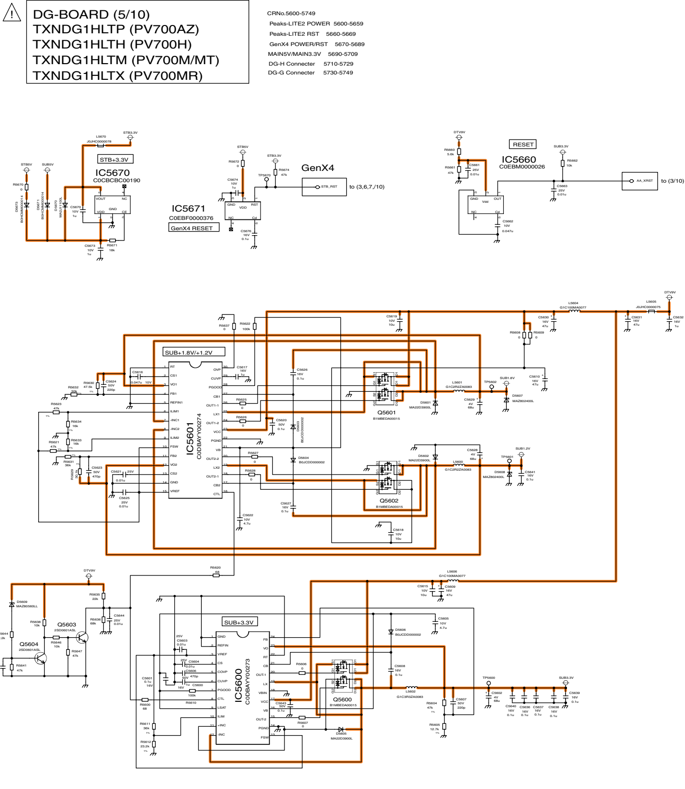
TH-42PV700AZ/H/M/MR/MT DG-Board (5 of 10) Schematic Diagram
