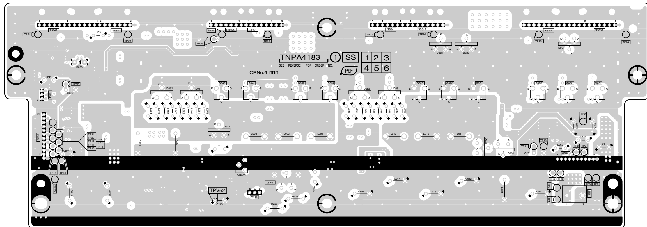
SS-BOARD (FOIL SIDE) TNPA4183
