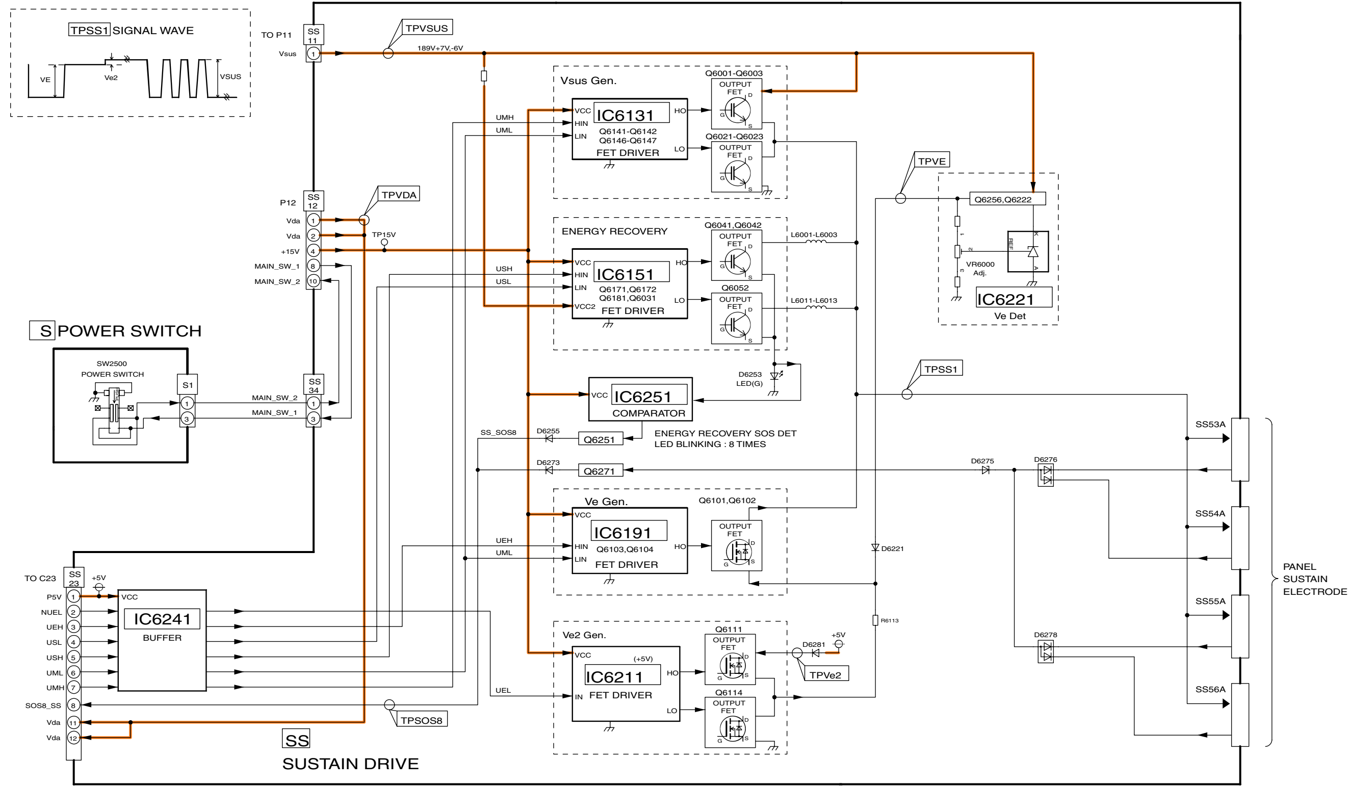
TH-42PV700AZ/H/M/MR/MT SS-Board Block Diagram
