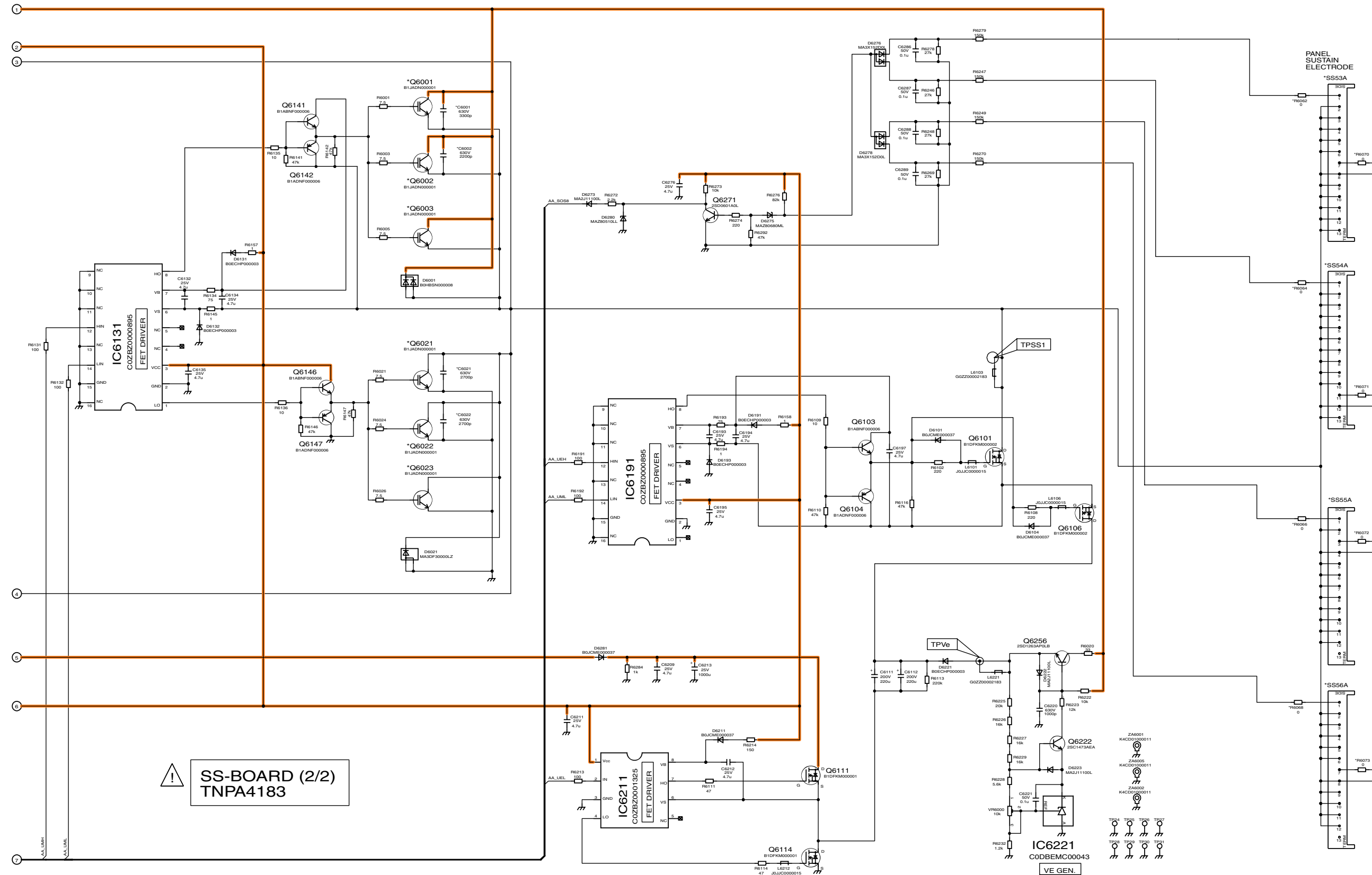
TH-42PV700AZ/H/M/MR/MT SS-Board (2 of 2) Schematic Diagram
