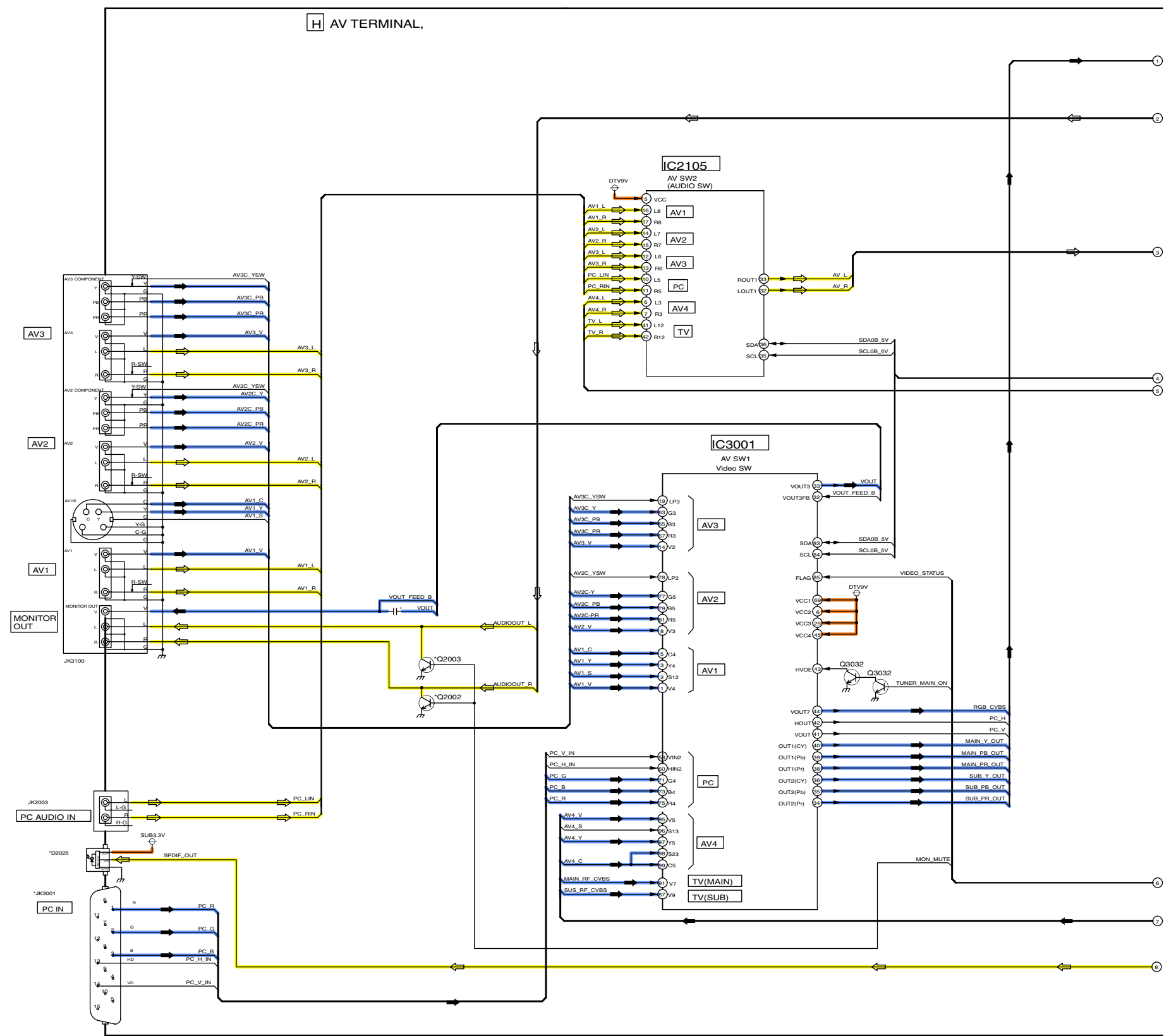
TH-42PV700AZ/H/M/MR/MT H-Board (1 of 2) Block Diagram
