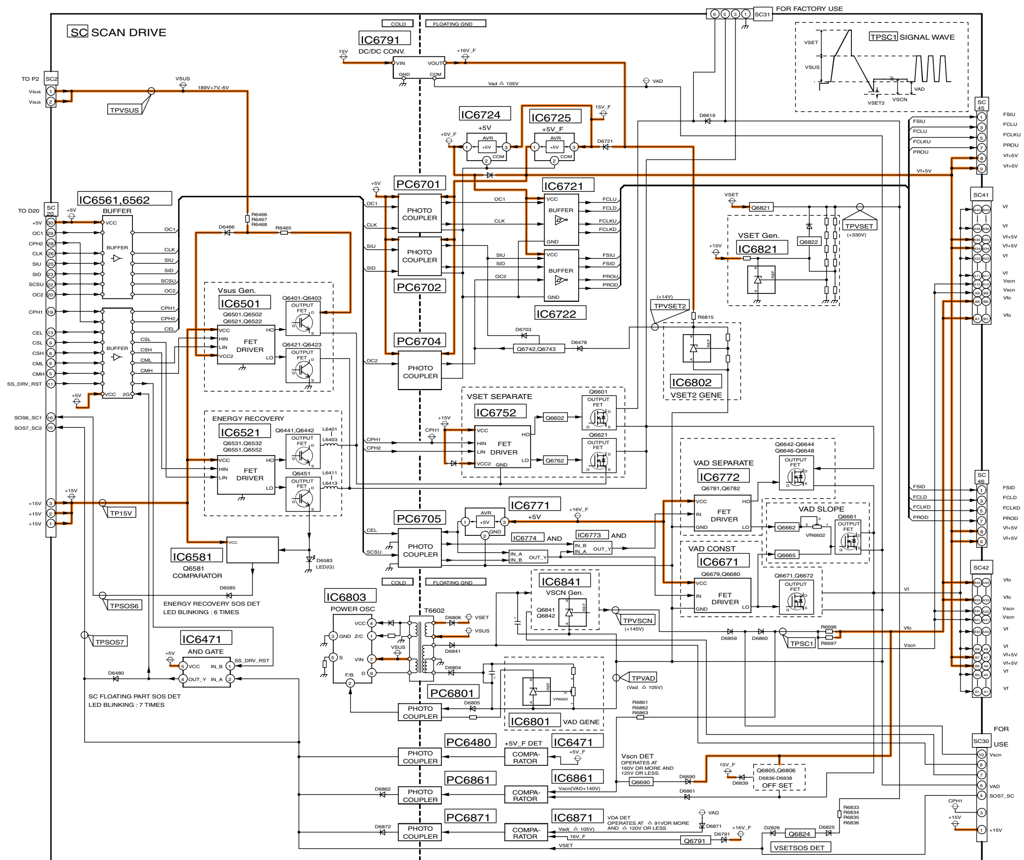
TH-42PV700AZ/H/M/MR/MT SC-Board Block Diagram
