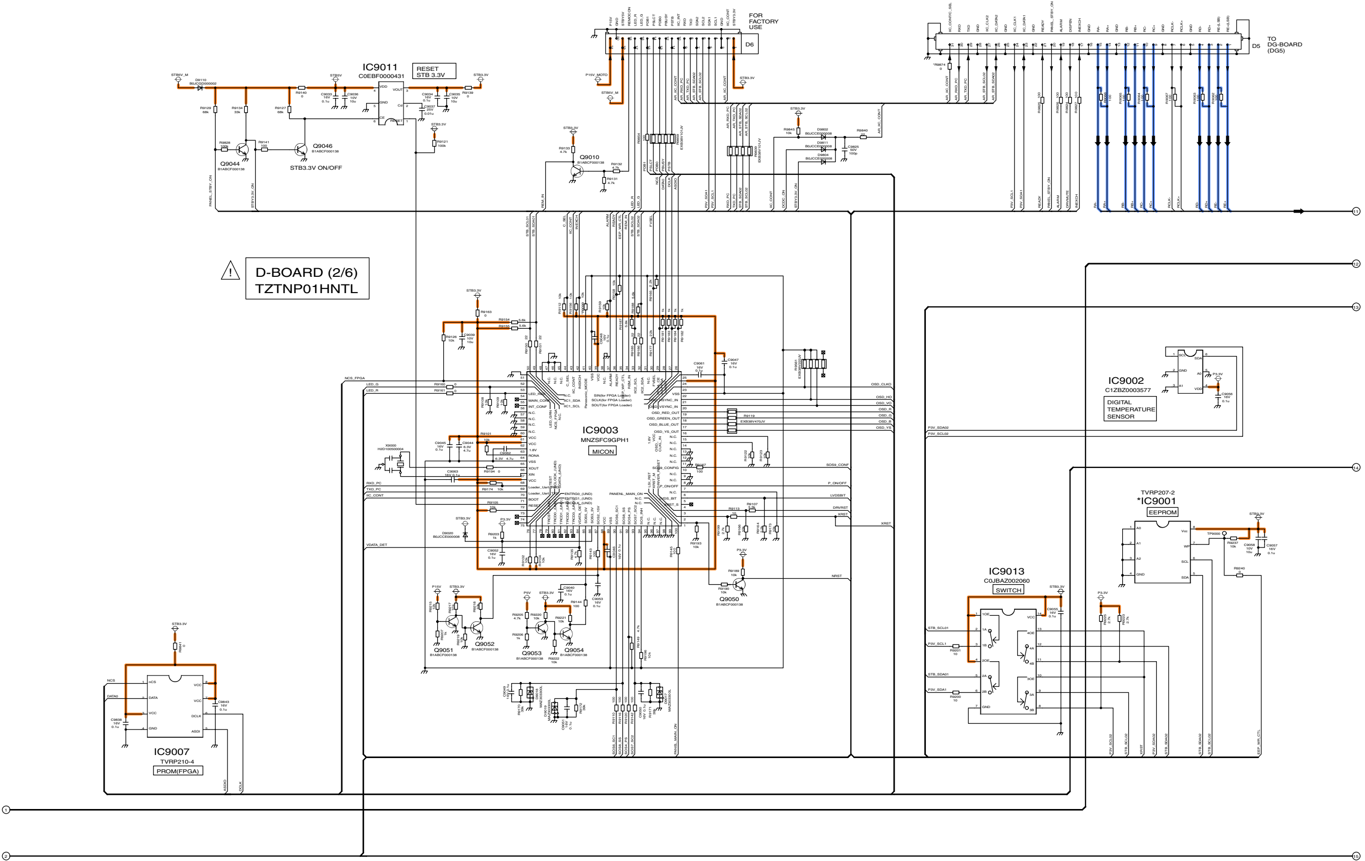
TH-42PV700AZ/H/M/MR/MT D-Board (2 of 6) Schematic Diagram
