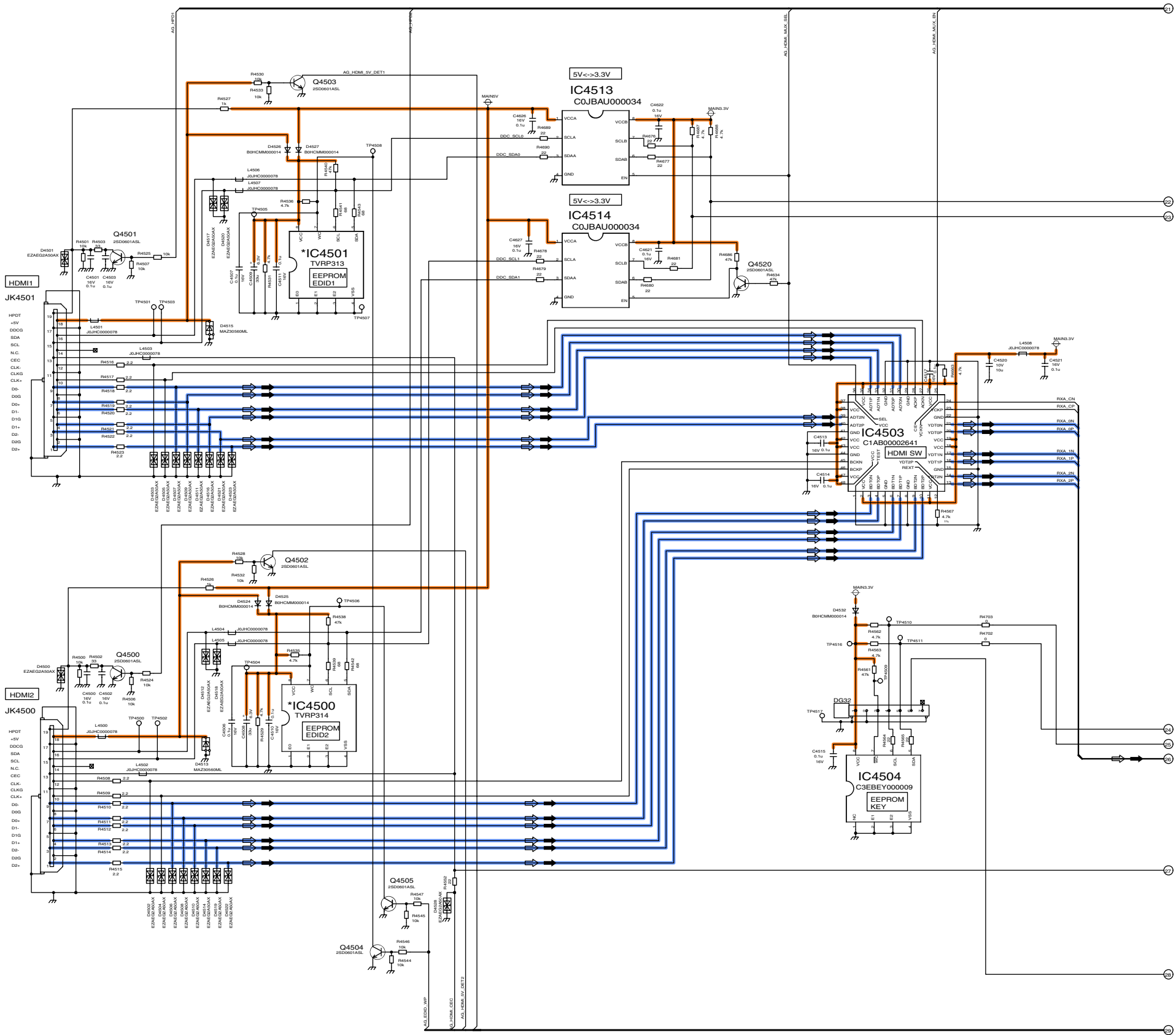
TH-42PV700AZ/H/M/MR/MT DG-Board (8 of 10) Schematic Diagram
