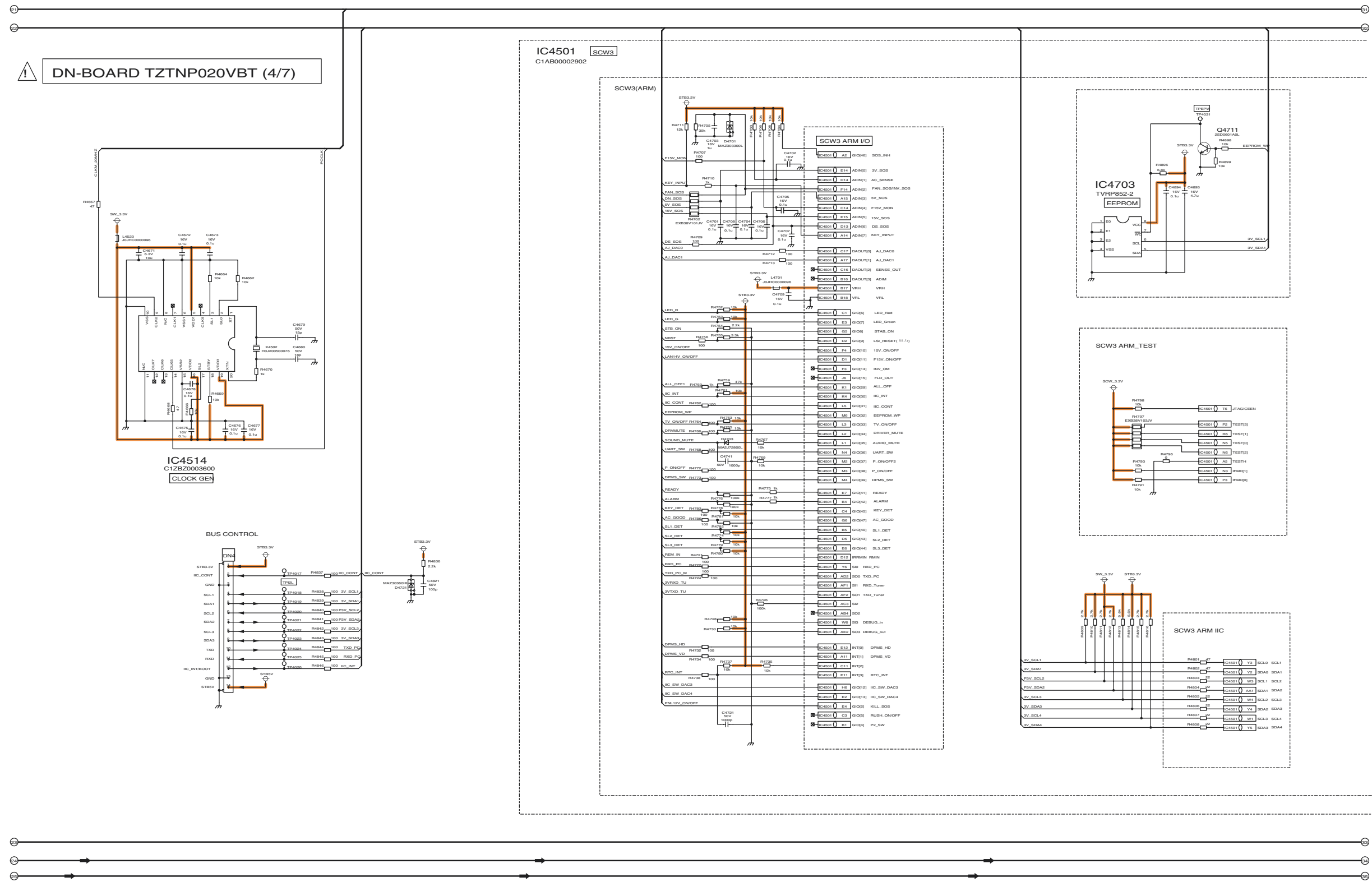
TH-42PH11GK/MK/MS DN-Board (4 of 7) Schematic Diagram
