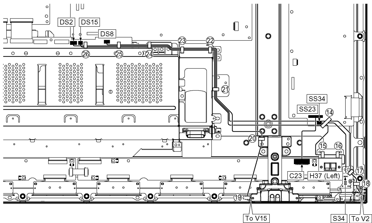
Clamp position
