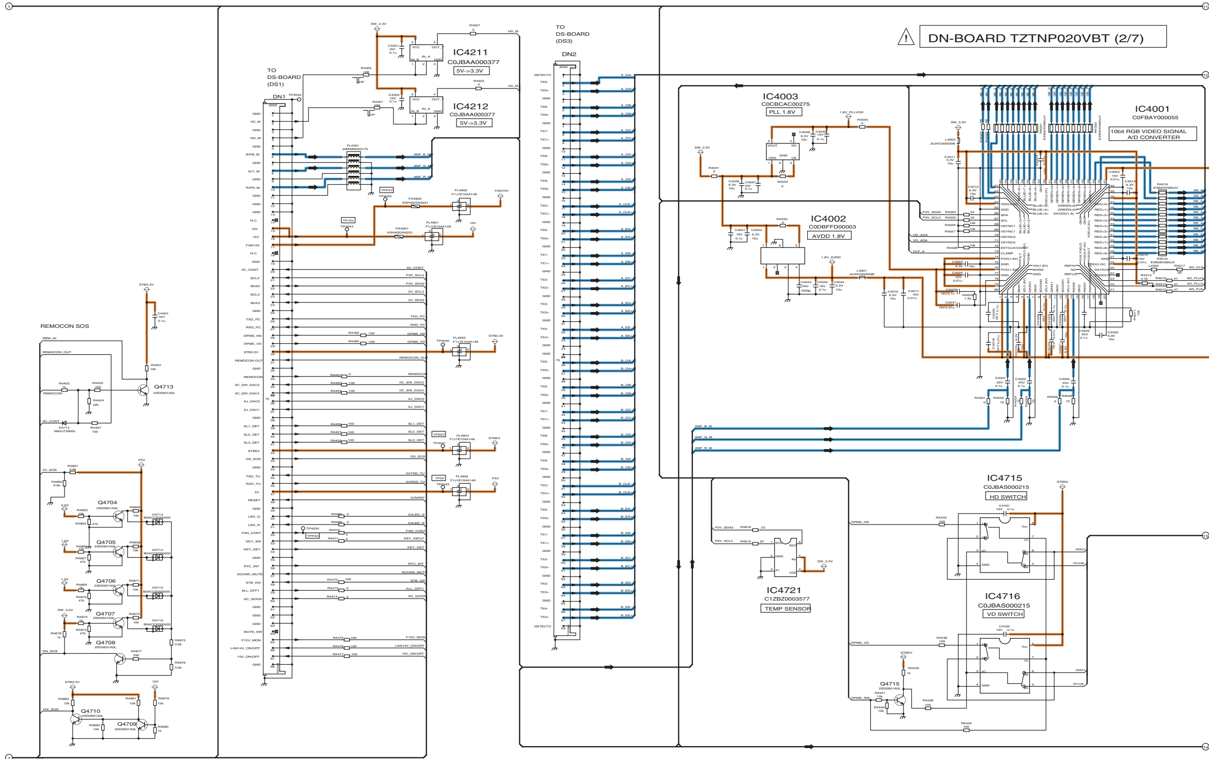
TH-42PH11GK/MK/MS DN-Board (2 of 7) Schematic Diagram
