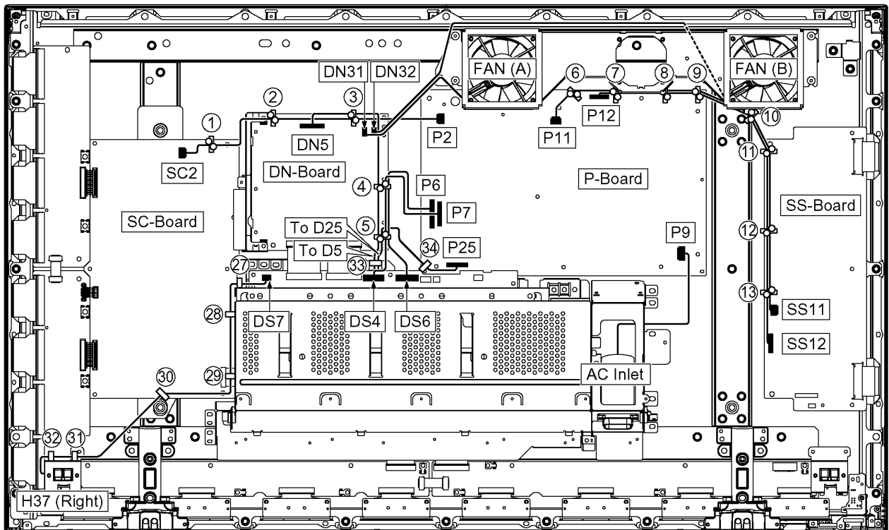
Clamp position
