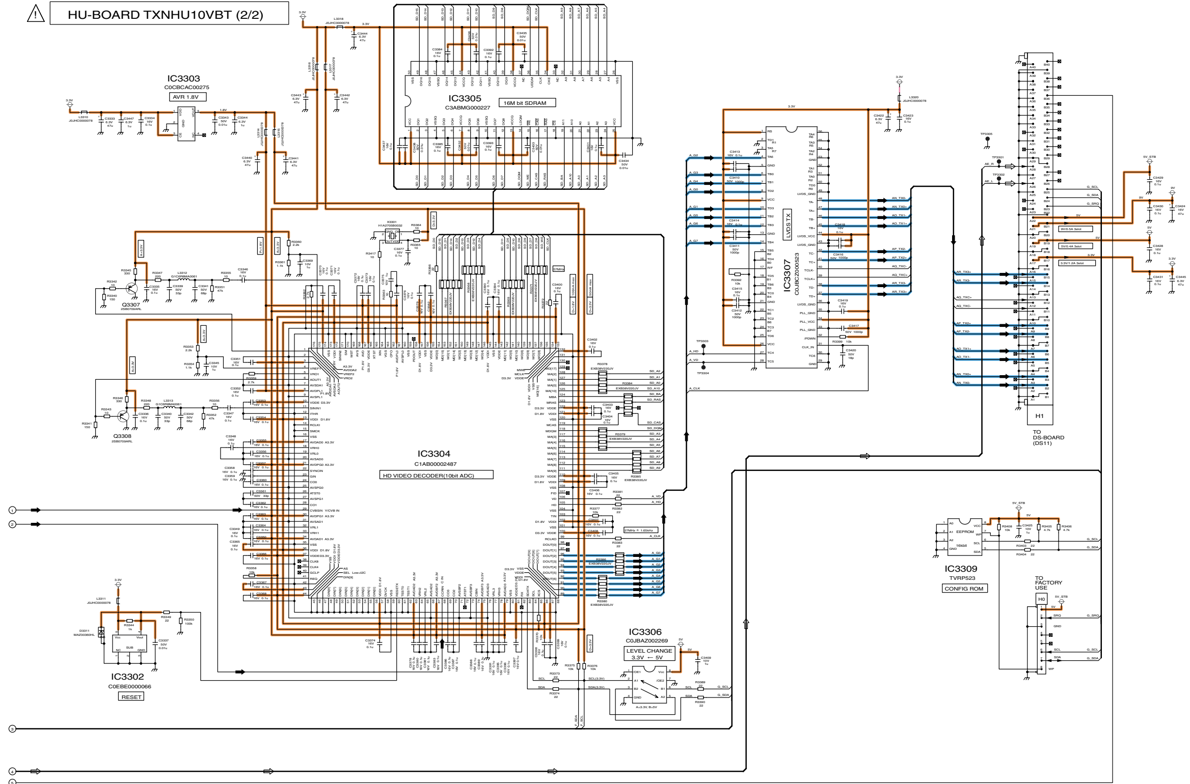
TH-42PH11GK/MK/MS HU-Board (2 of 2) Schematic Diagram
