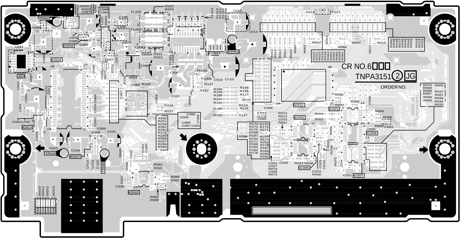
JG-BOARD(COMPONENT SIDE) TNPA3151AD
