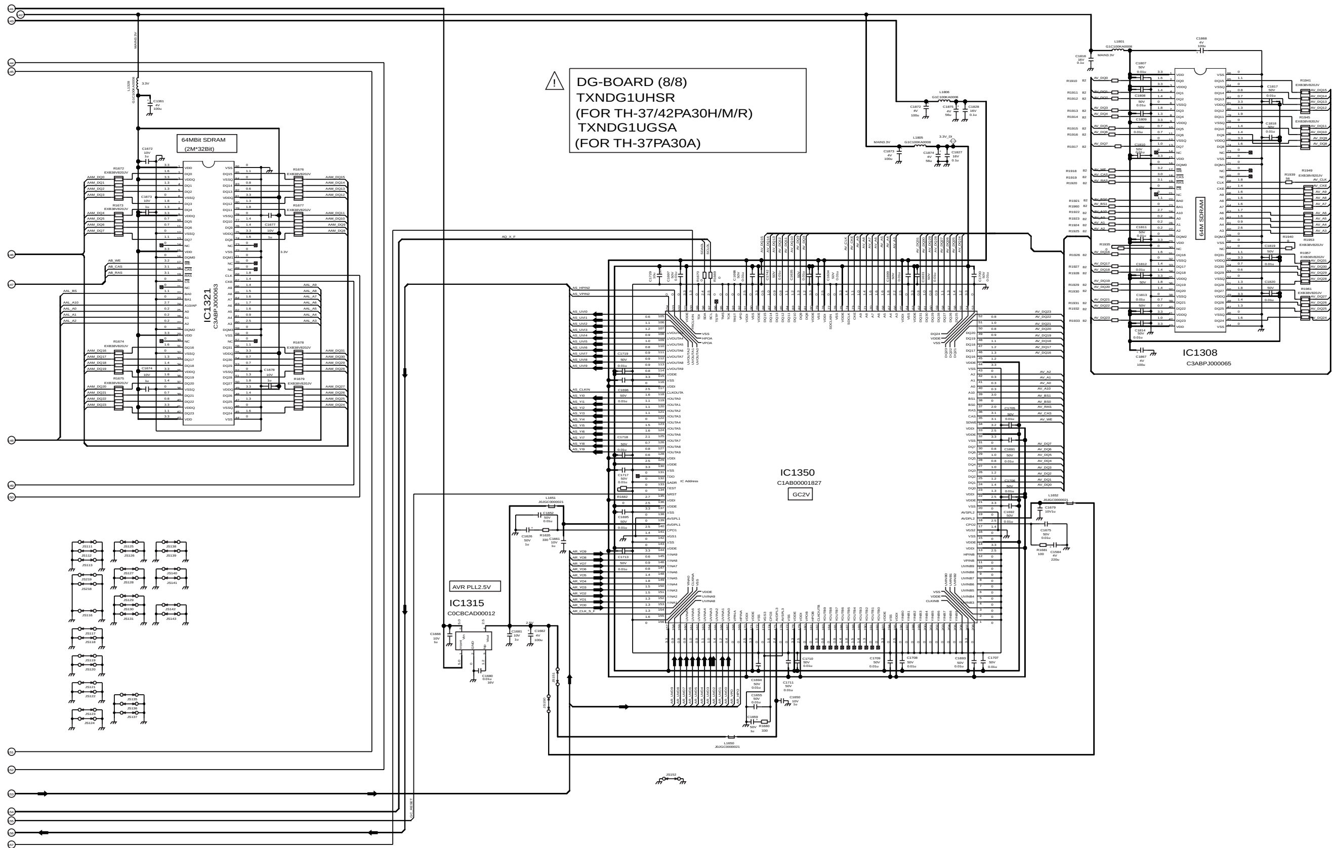
TH-37PA30A, TH-37/42PA30H/M/R DG-Board (8 of 8) Schematic Diagram
