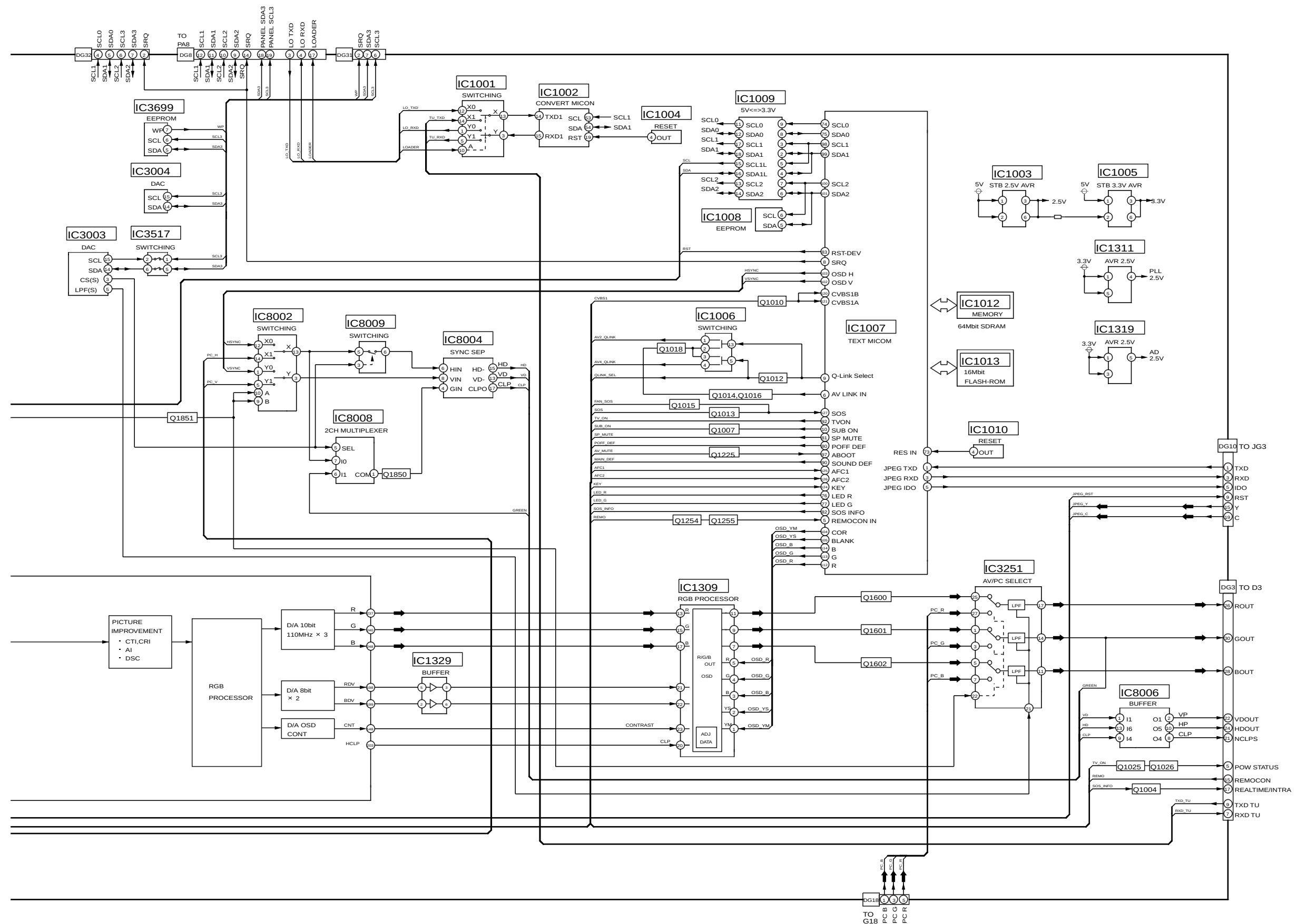
TH-37PA30A, TH-37/42PA30H/M/R DG-Board (2 of 2) Block Diagram
