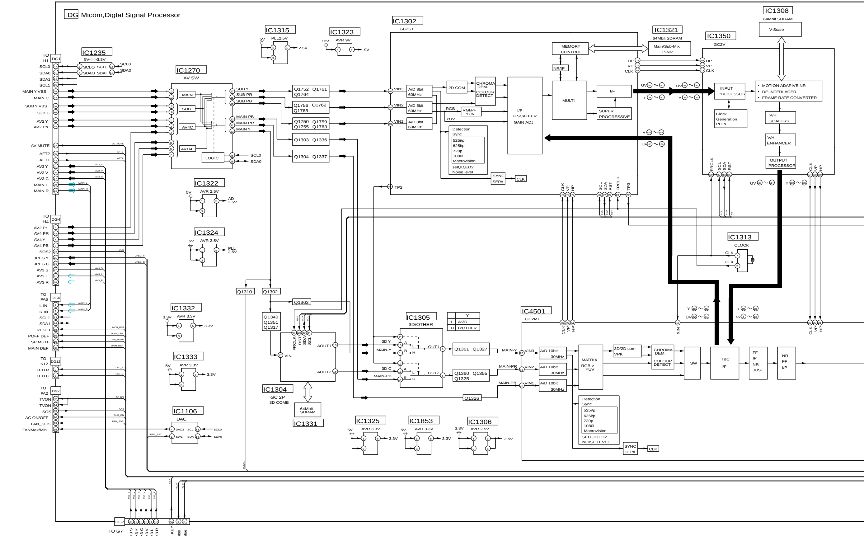
TH-37PA30A,TH-37/42PA30H/M/R DG-Board (1 of 2) Block Diagram
