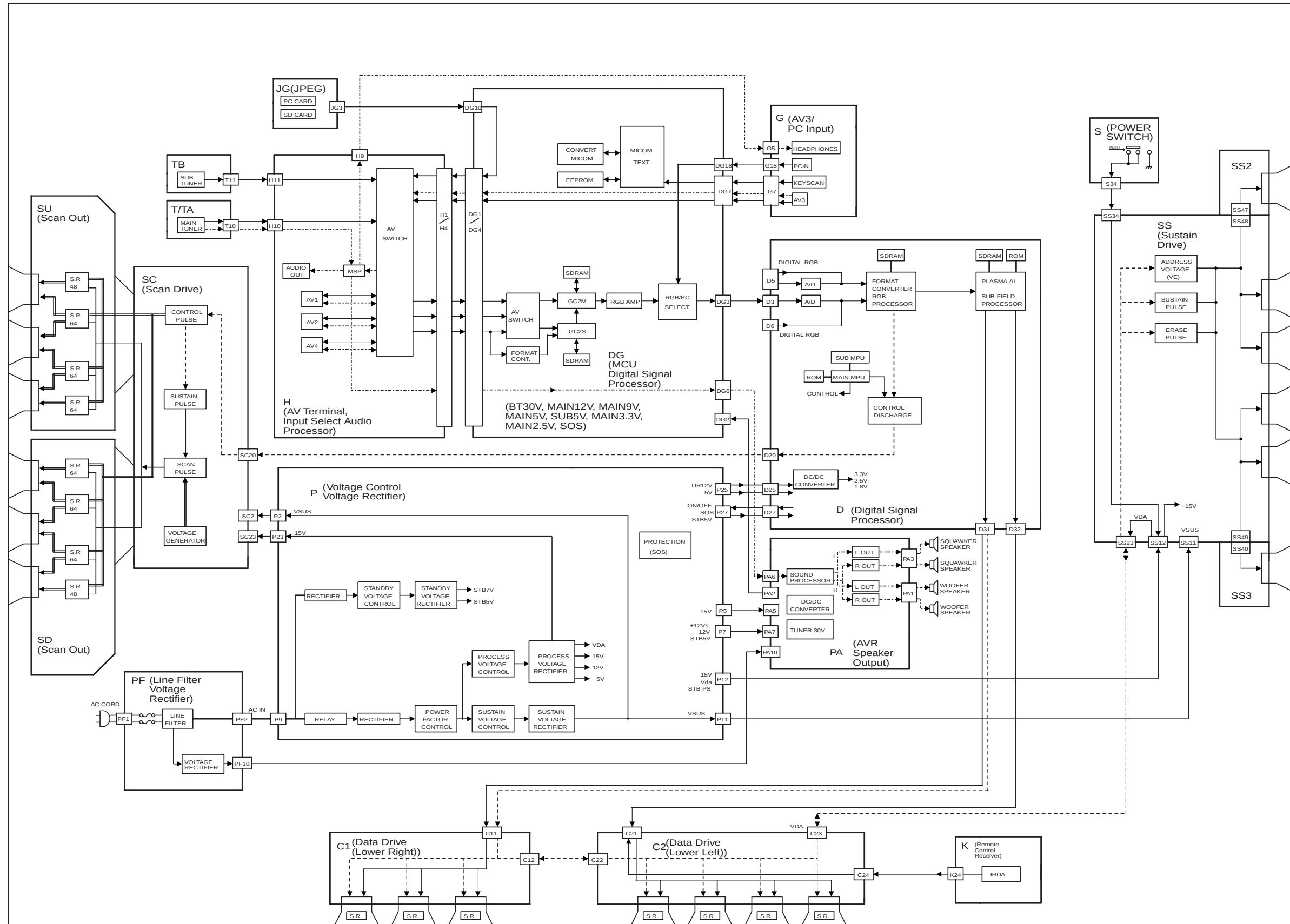
TH-37PA30A,TH-37/42PA30H/M/R Main Block Diagram
