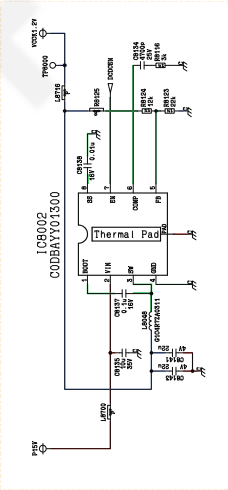
VCC4.2V
