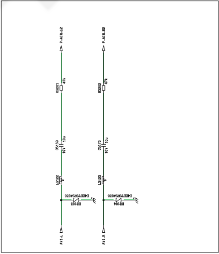
VIDEO/AUDIO IN
