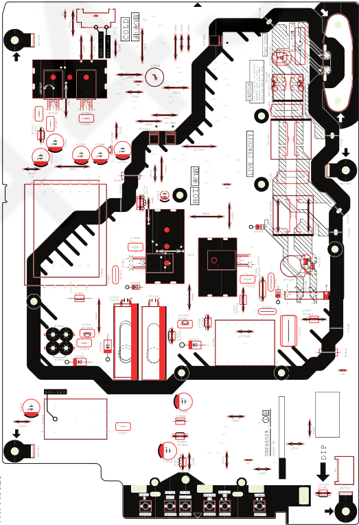
P-BOARD (TOP COMPONENT SIDE) TNPAG029
