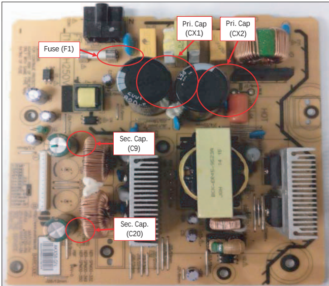
Power PCB
