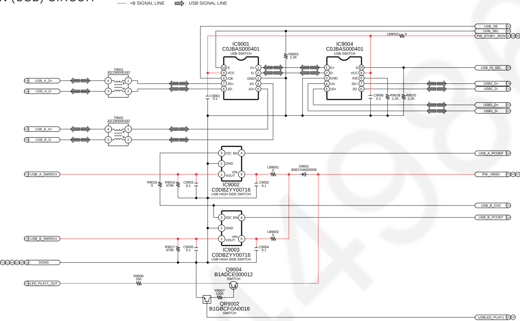
SCHEMATIC DIAGRAM - 10 B MAIN (USB) CIRCUIT
