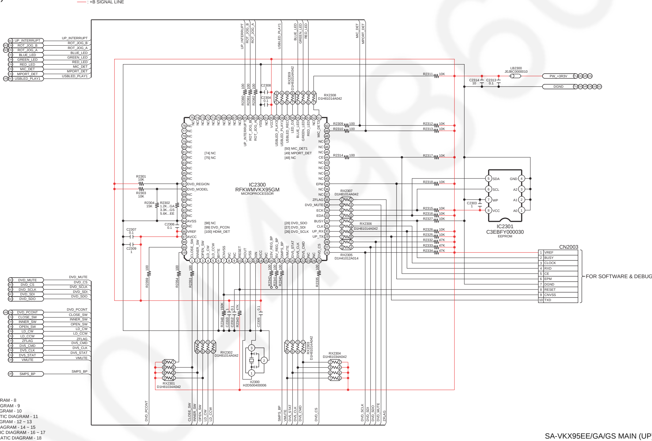
SCHEMATIC DIAGRAM - 8 B MAIN (UP) CIRCUIT
