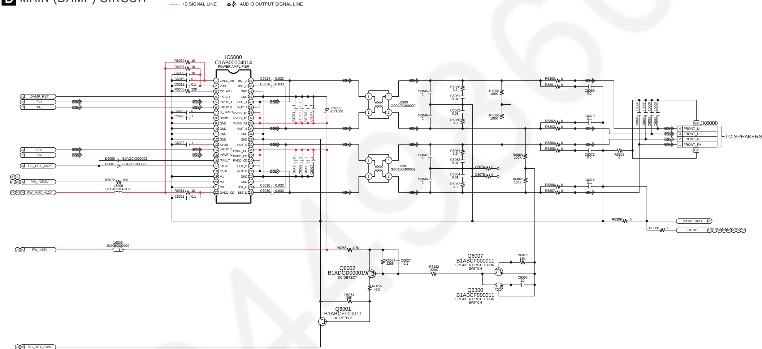
SCHEMATIC DIAGRAM - 13
