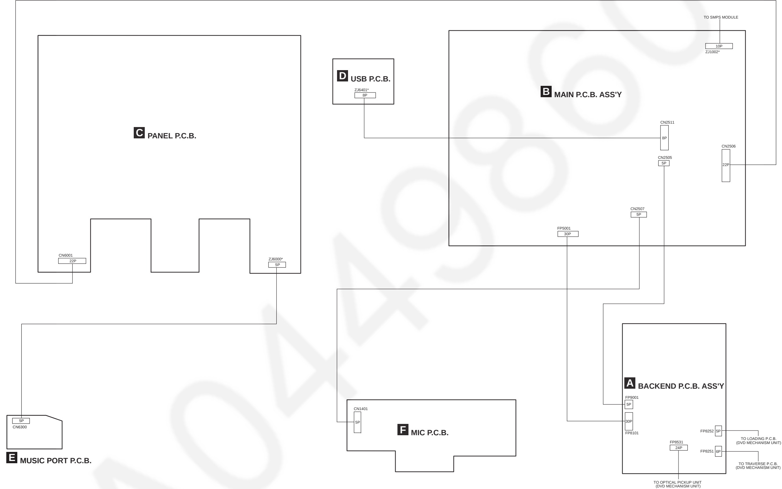
SA-VKX65GA/GS WIRING CONNECTION DIAGRAM
