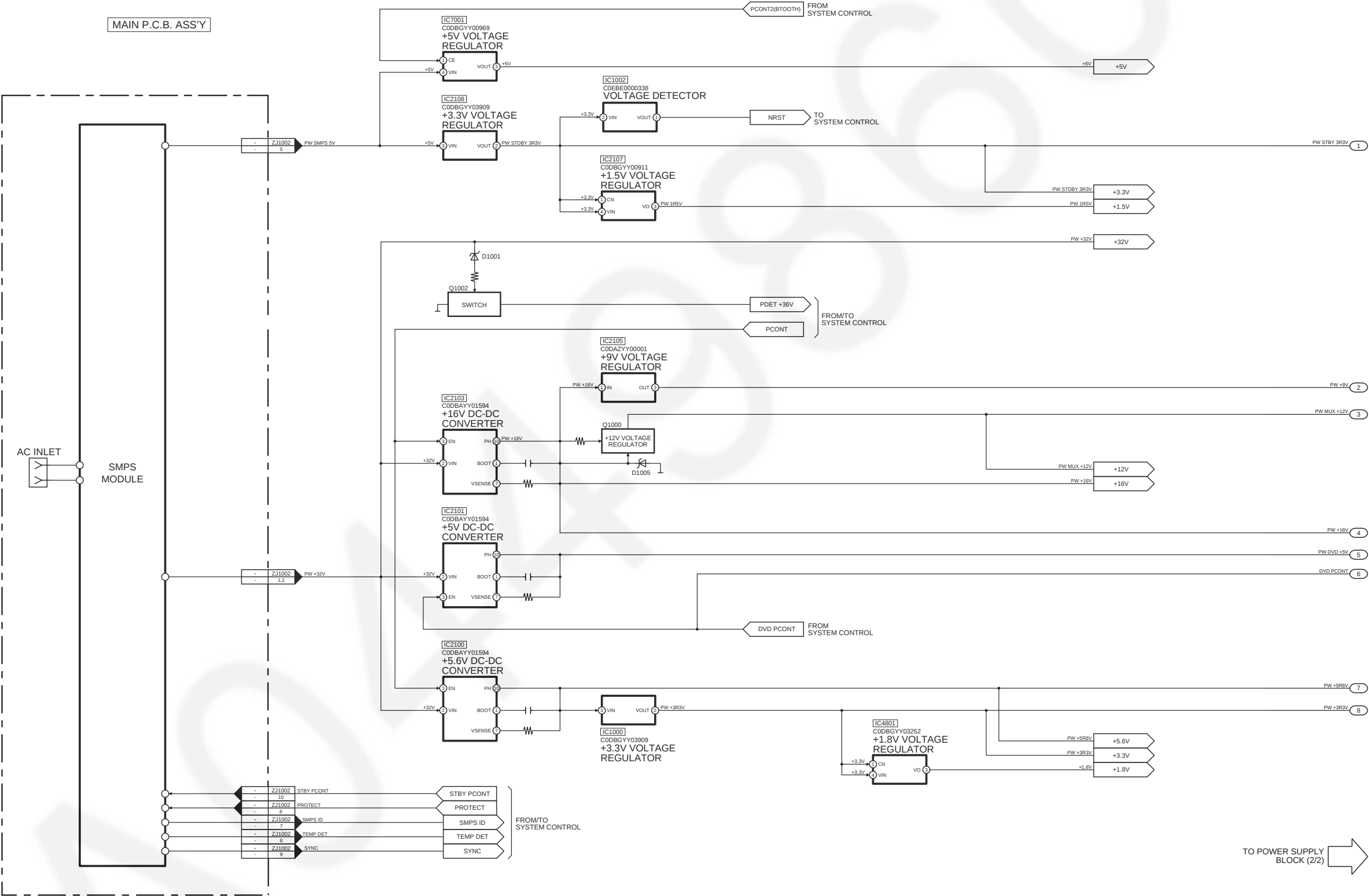
SA-VKX65GA/GS POWER SUPPLY (1/2) BLOCK DIAGRAM
