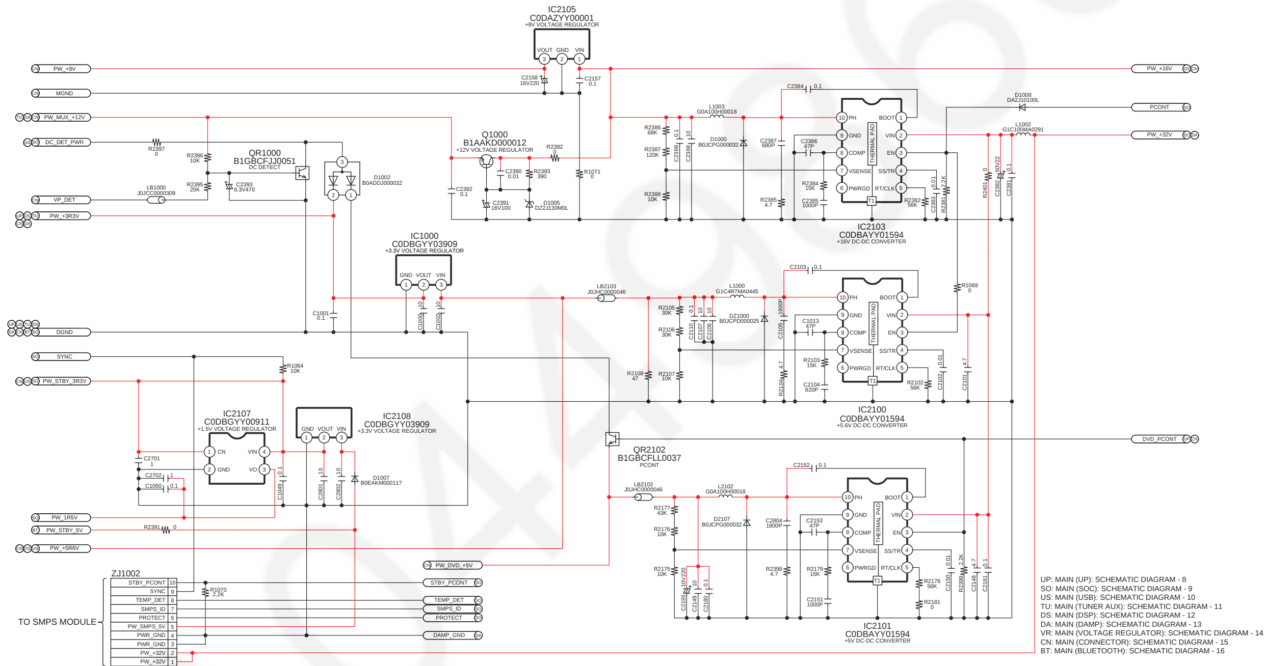
SA-VKX65GA/GS MAIN (VOLTAGE REGULATOR) CIRCUIT
