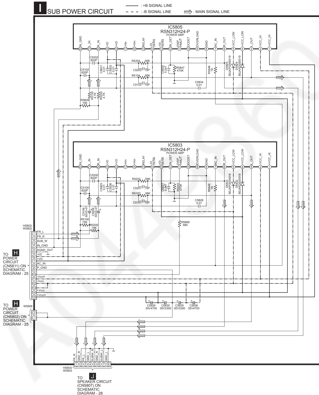
SCHEMATIC DIAGRAM - 26
