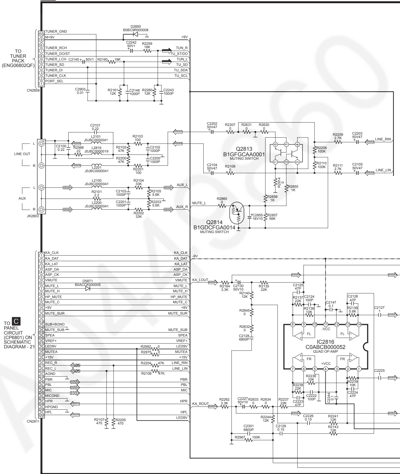
SCHEMATIC DIAGRAM - 9
