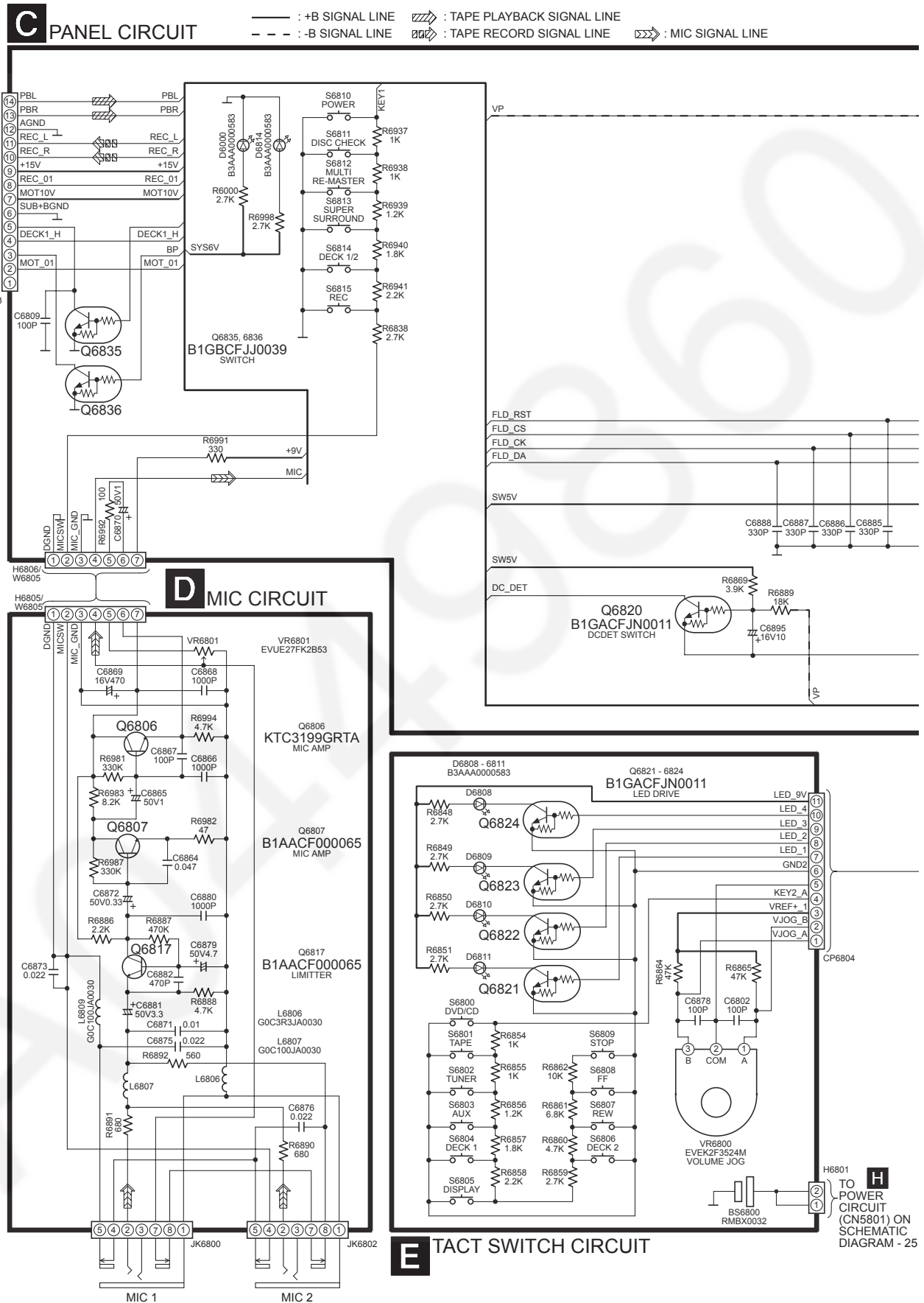
SCHEMATIC DIAGRAM - 18
