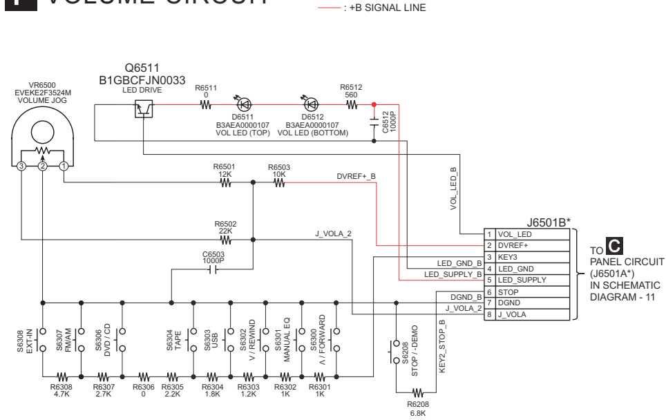
SCHEMATIC DIAGRAM - 12 F VOLUME CIRCUIT
