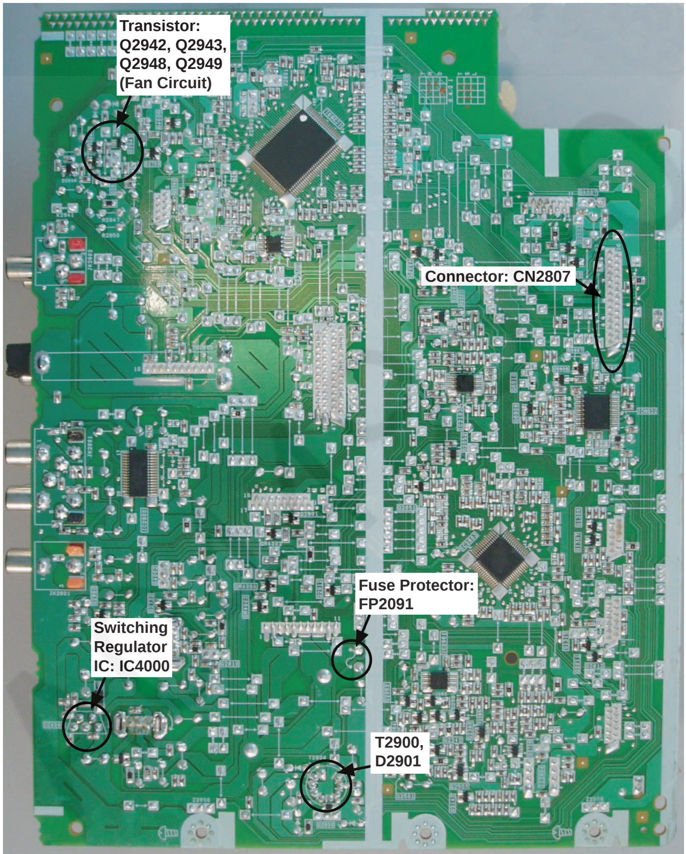
Figure 4 Main P.C.B.
