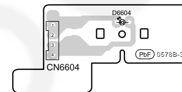
D SIDE BAR (L) LED P.C.B. (REPX0671C)
