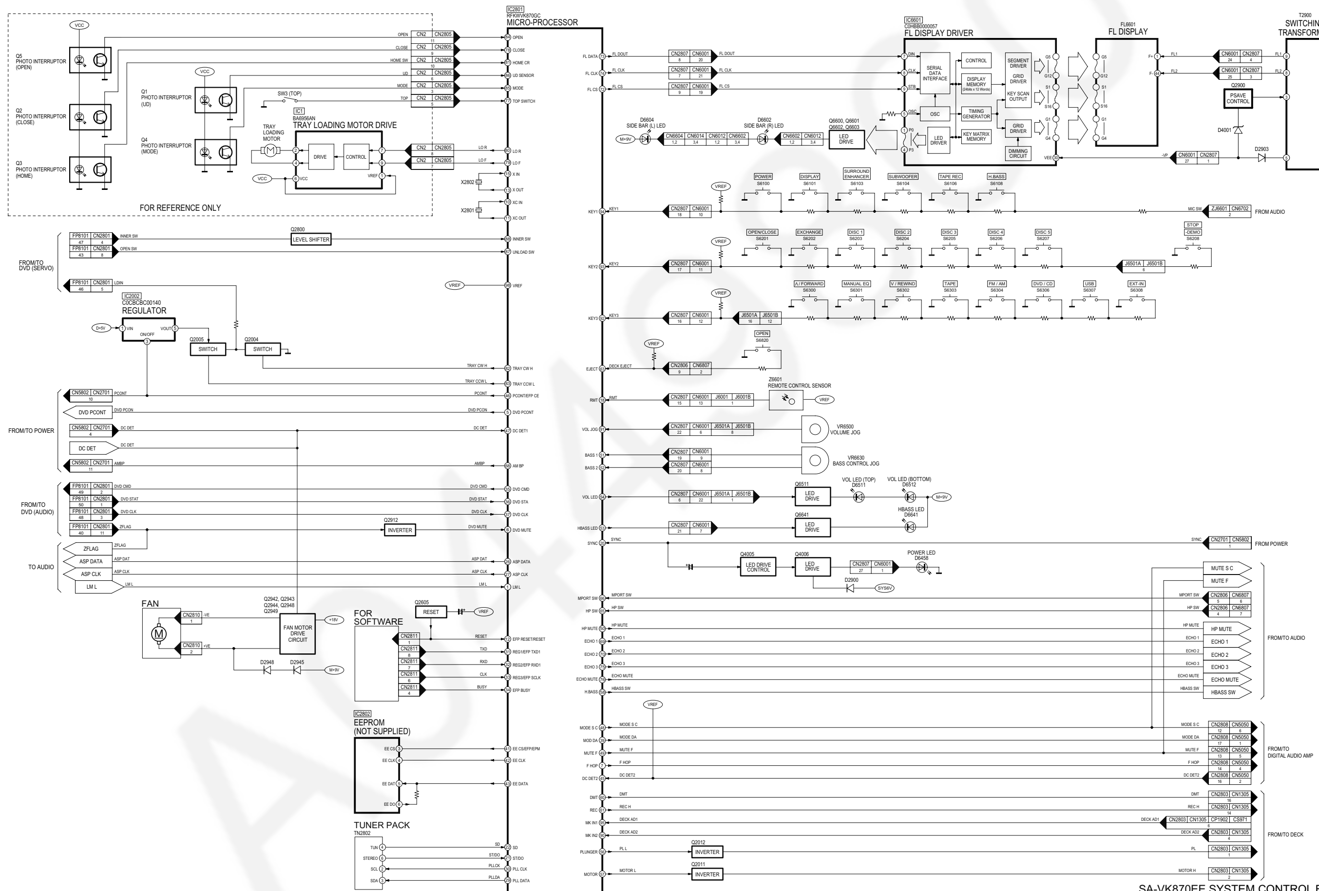
SA-VK870EE SYSTEM CONTROL BLOCK DIAGRAM
