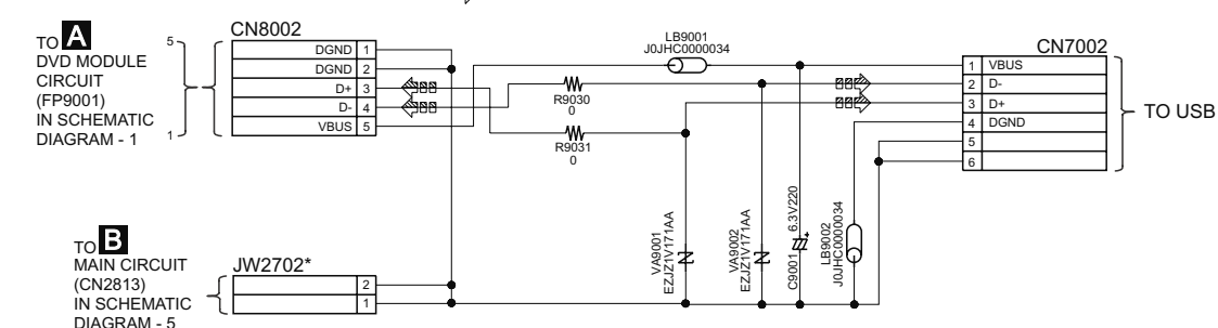
SA-VK870EE TACT SWITCH / MUSIC PORT / REMOTE SENSOR / MIC / USB CIRCUIT
