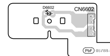
E SIDE BAR (R) LED P.C.B. (REPX0671C)
