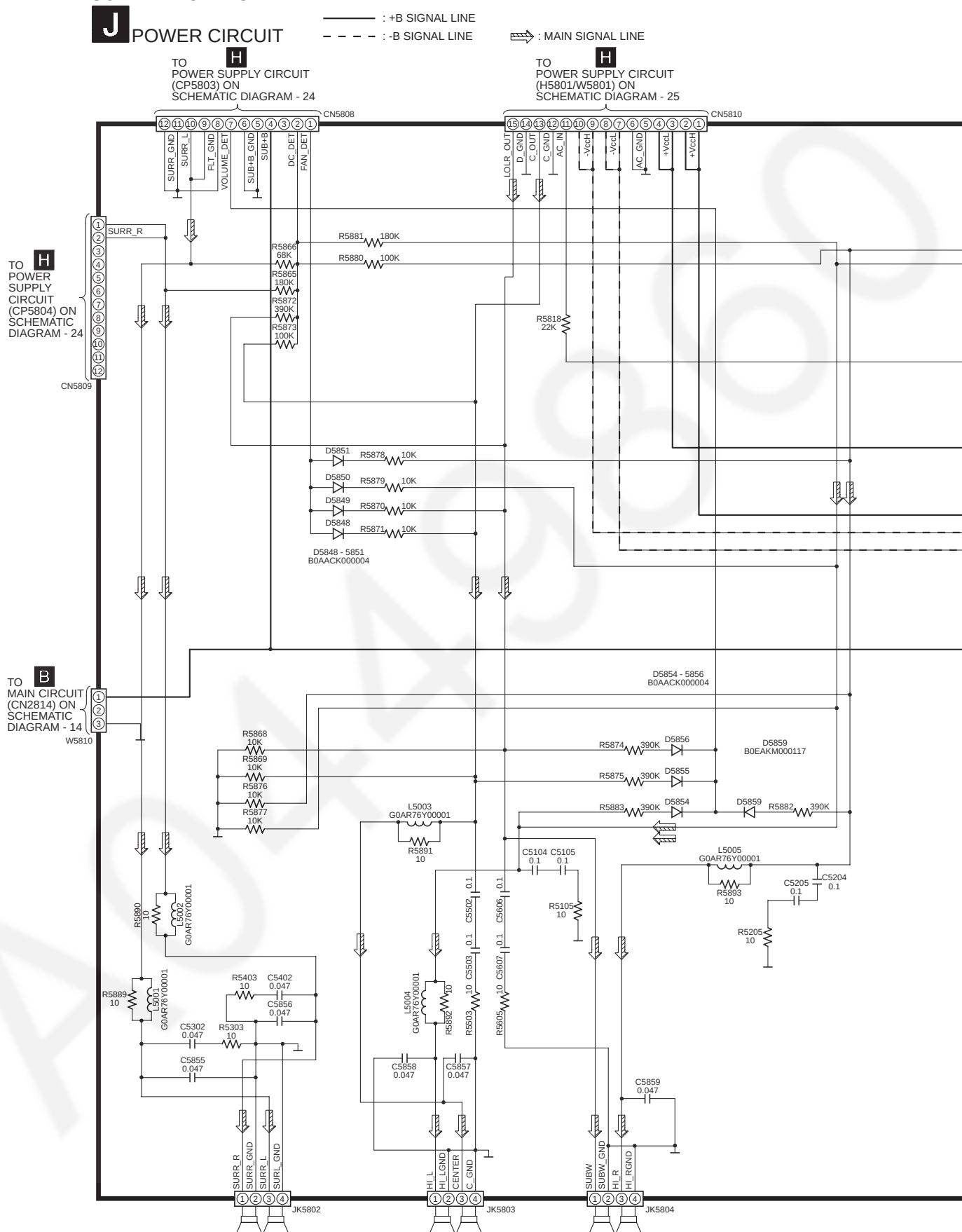
SCHEMATIC DIAGRAM - 27
