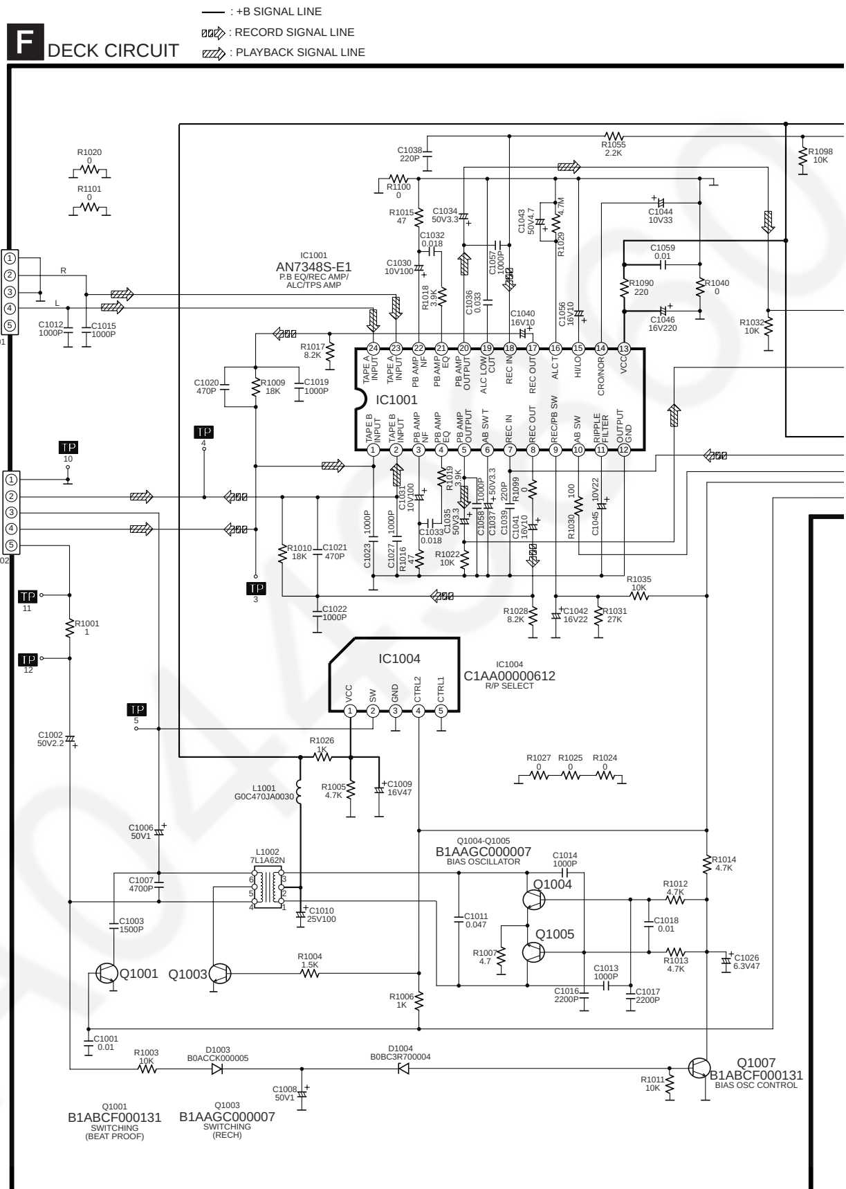
SCHEMATIC DIAGRAM - 22
