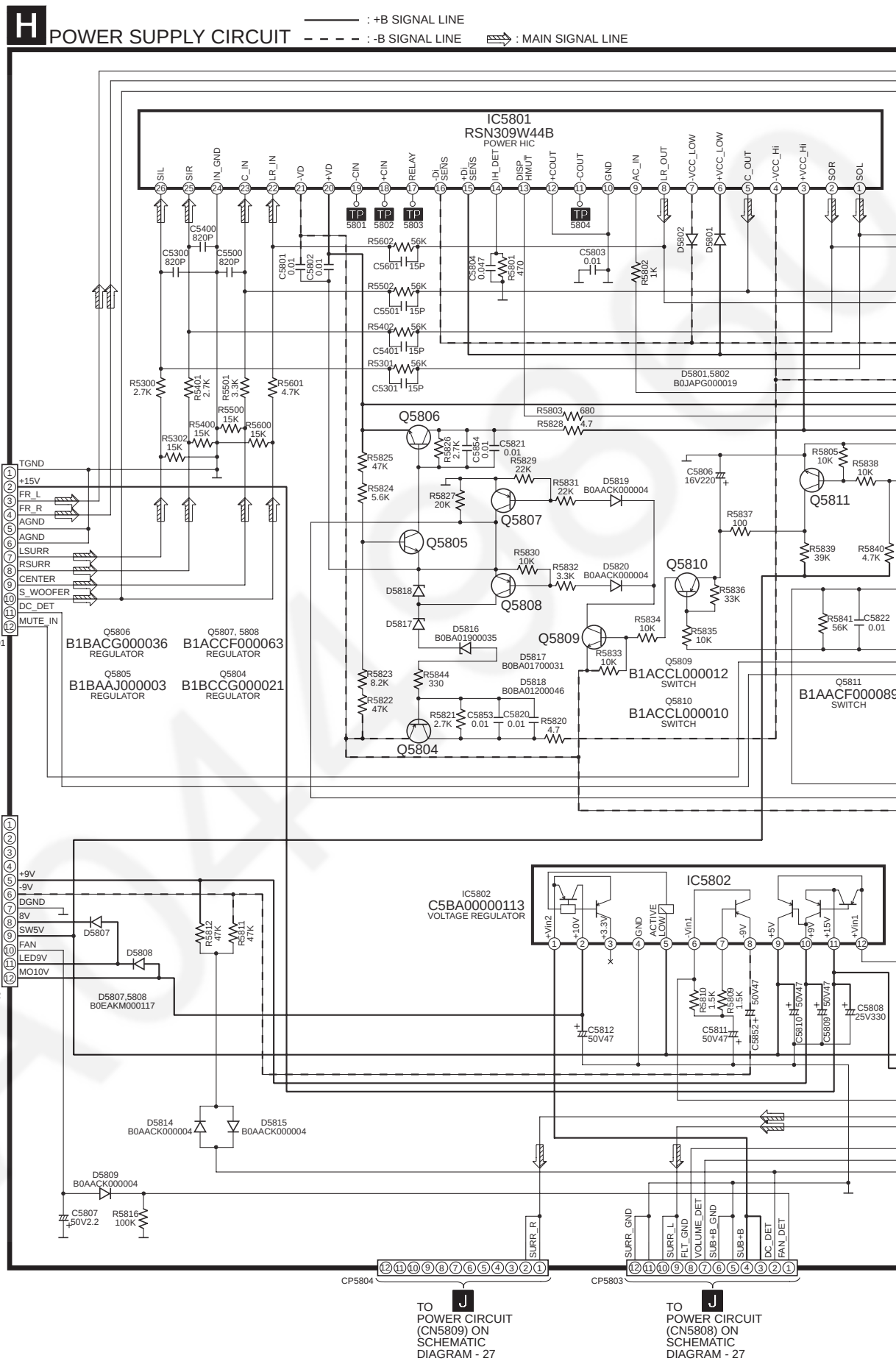
SCHEMATIC DIAGRAM - 24
