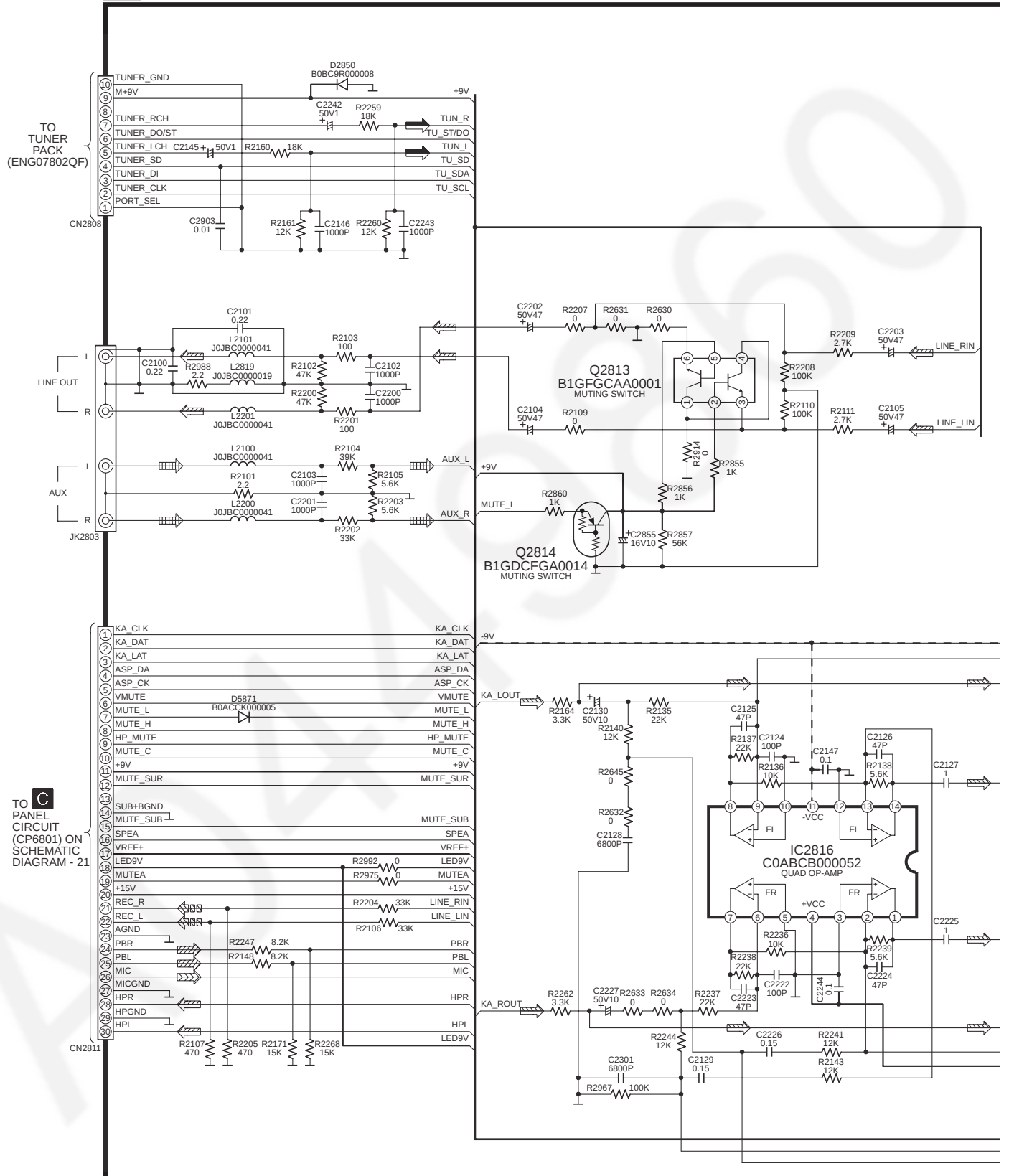
SCHEMATIC DIAGRAM - 9
