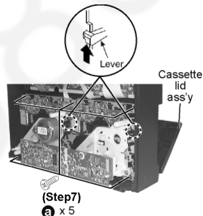
Cassette mechanism
