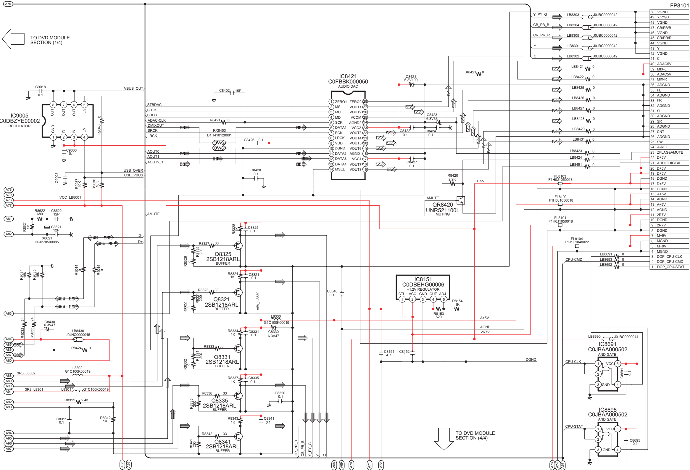
SCHEMATIC DIAGRAM - 2
