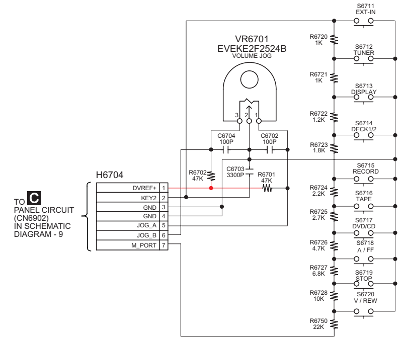
SCHEMATIC DIAGRAM - 10
