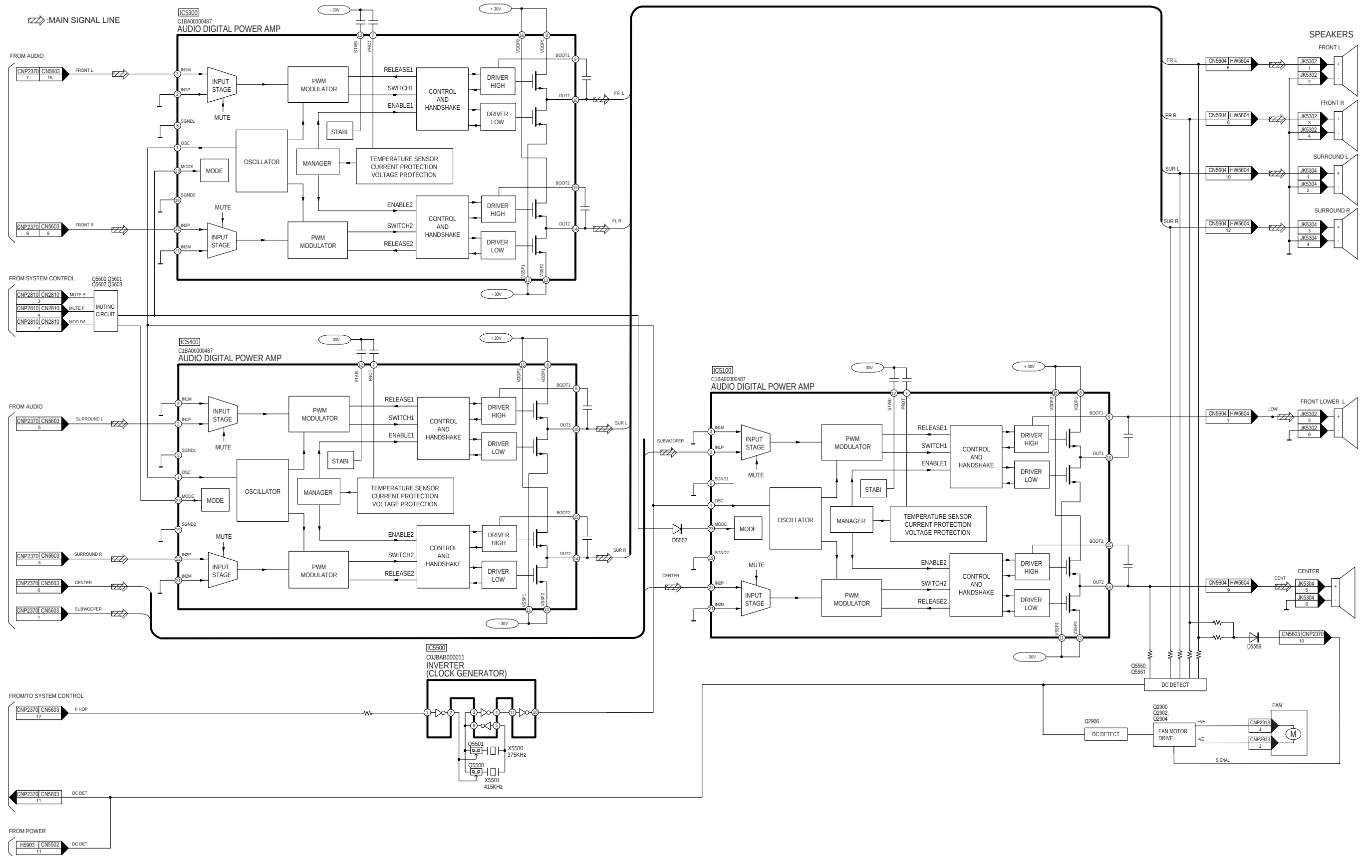
SA-VK760GC/GCS/GCT/GS AUDIO DIGITAL AMP BLOCK DIAGRAM
