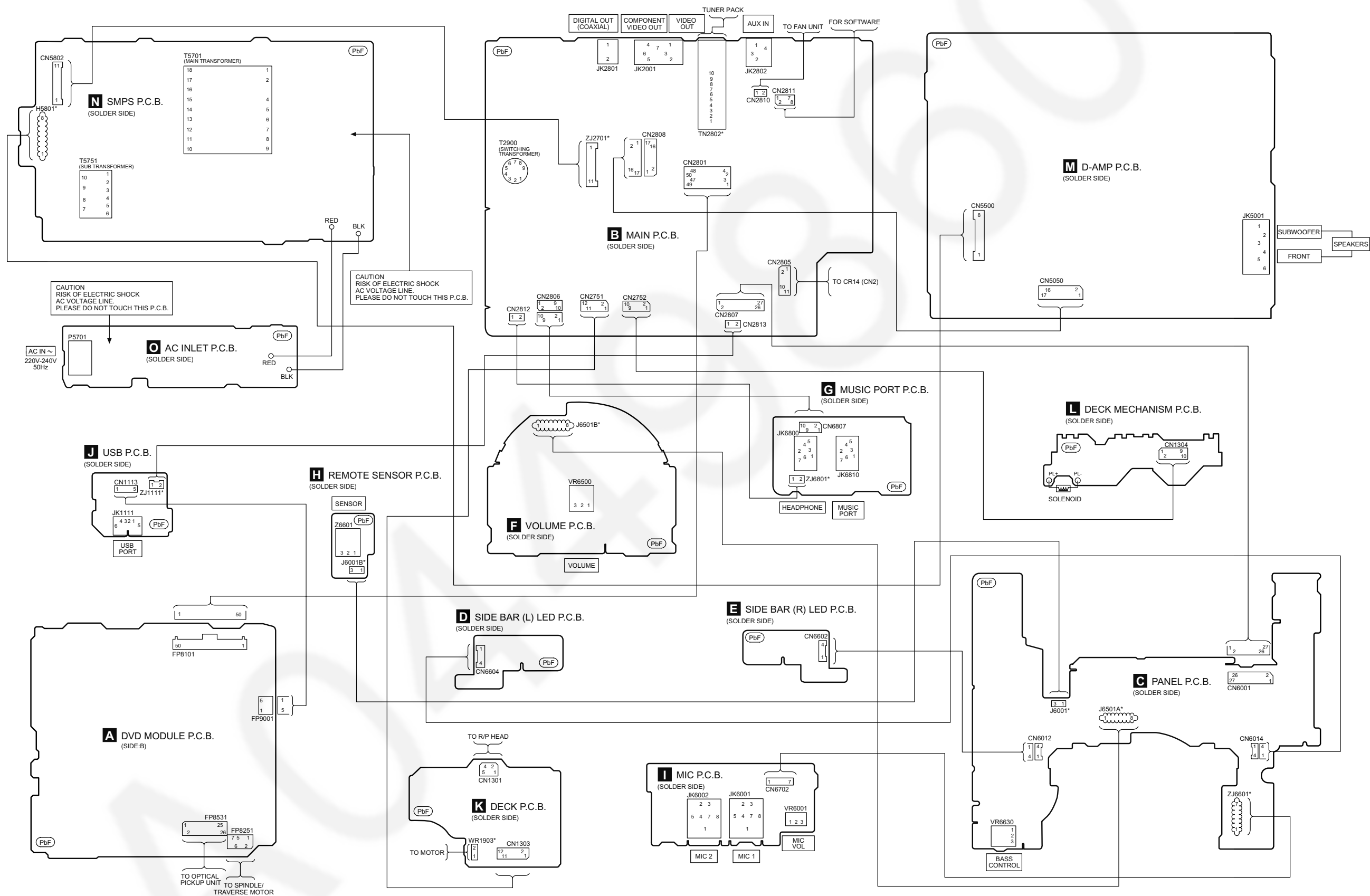
SA-VK680EE WIRING CONNECTION
