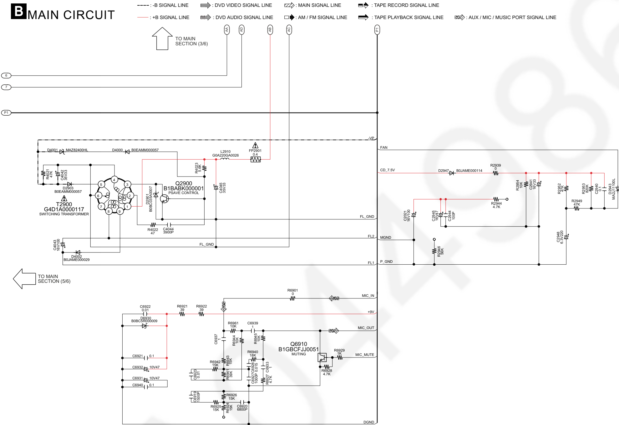
SCHEMATIC DIAGRAM - 10
