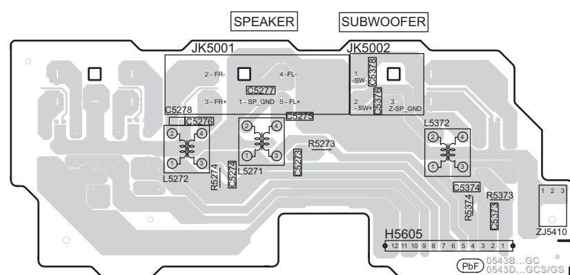
F SPEAKER P.C.B (REPX0594B...GC) (REPX0594D...GCS/GS)
