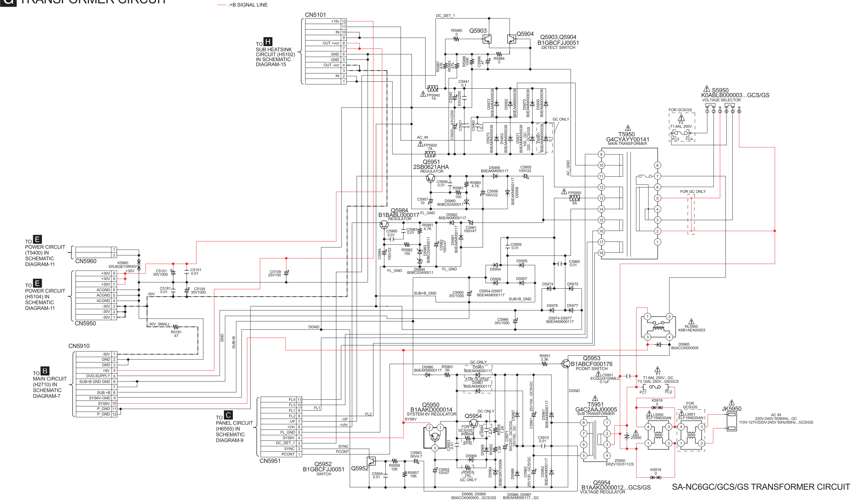
SCHEMATIC DIAGRAM - 14 G TRANSFORMER CIRCUIT
