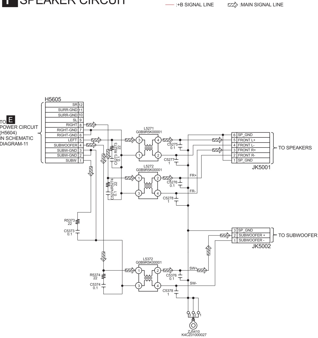
SCHEMATIC DIAGRAM - 13 F SPEAKER CIRCUIT
