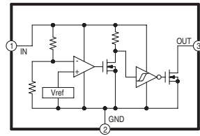
IC7302 RESET IC IC-DETAIL BLOCK DIAGRAM
