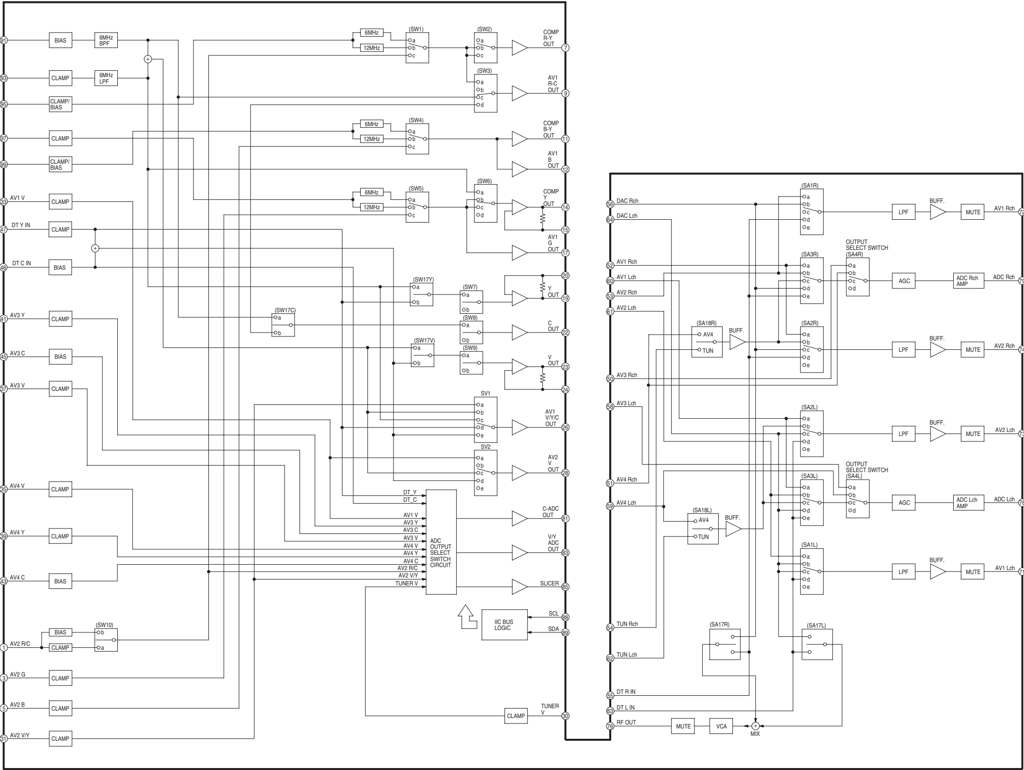
IC3001 VIDEO/AUDIO PROCESSOR IC-DETAIL BLOCK DIAGRAM
