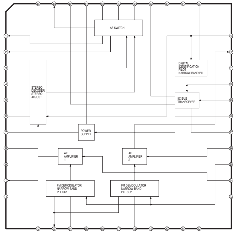
IC7301 DECODER IC IC-DETAIL BLOCK DIAGRAM
