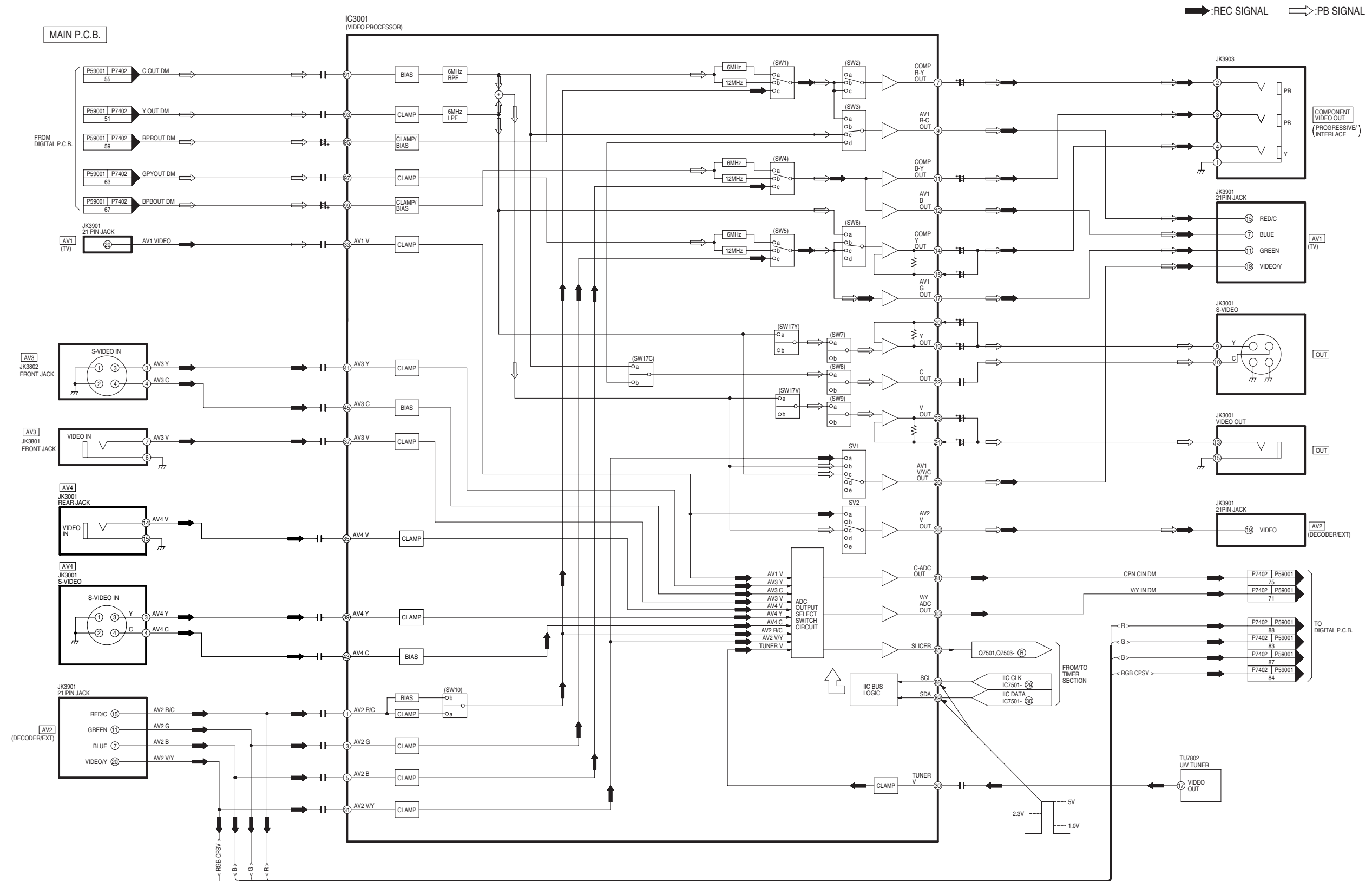
DMR-EH67GN/GC/GCS Analog Video Block Diagram
