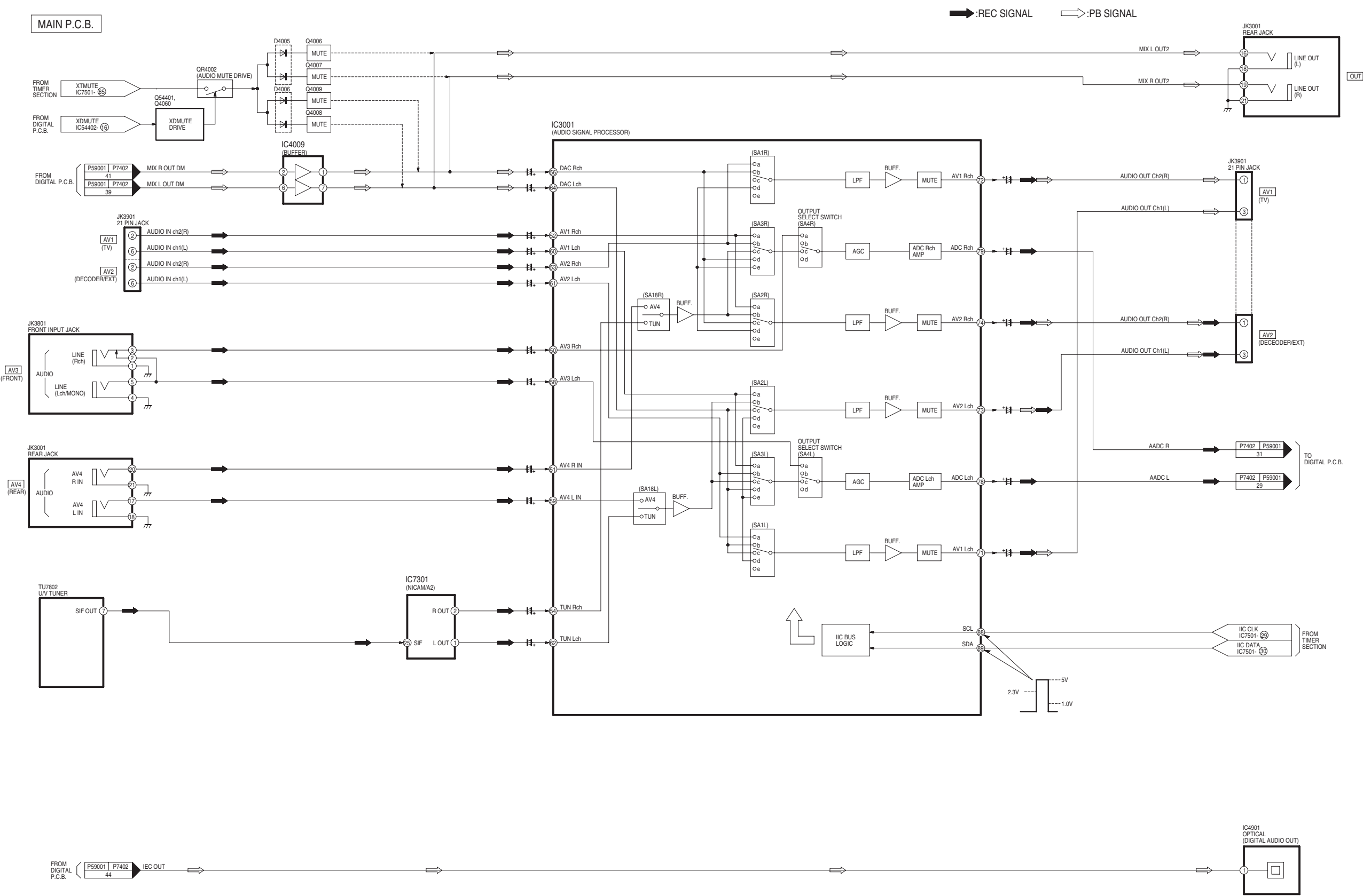
DMR-EH67GN/GC/GCS Analog Audio Block Diagram
