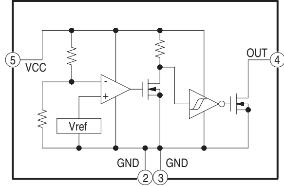
IC1501 RESET IC-DETAIL BLOCK DIAGRAM
