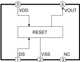
IC7302 RESET IC-DETAIL BLOCK DIAGRAM
