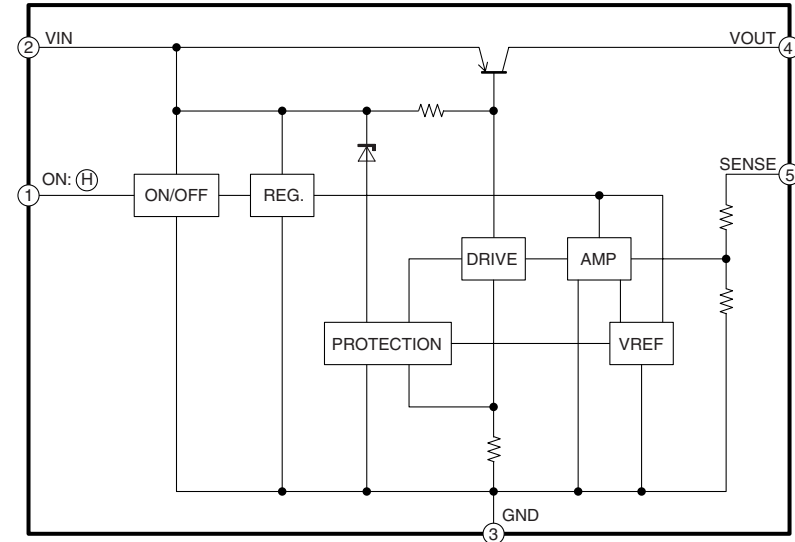
IC1506 DR +5V SWITCHING REGULATOR IC-DETAIL BLOCK DIAGRAM
