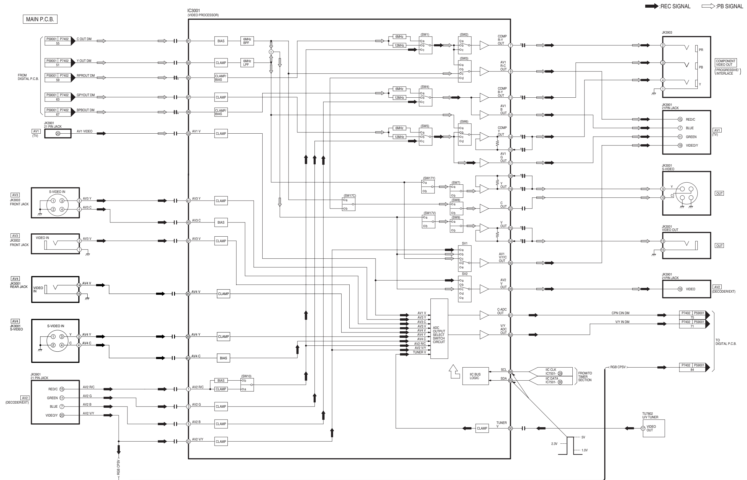
DMR-EH59GA/GC/GN Analog Video Block Diagram
