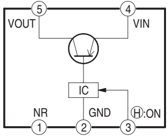
IC4001 AU +5V SWITCHING REGULATOR IC-DETAIL BLOCK DIAGRAM
