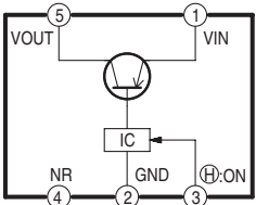
IC7402 BOOSTER +5V SWITCHING REGULATOR IC-DETAIL BLOCK DIAGRAM
