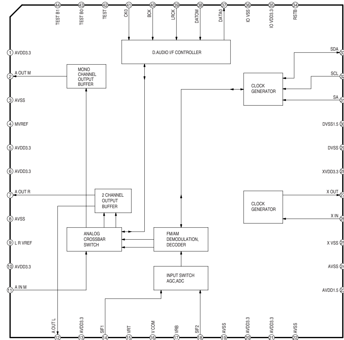
IC7301 DECODER IC-DETAIL BLOCK DIAGRAM
