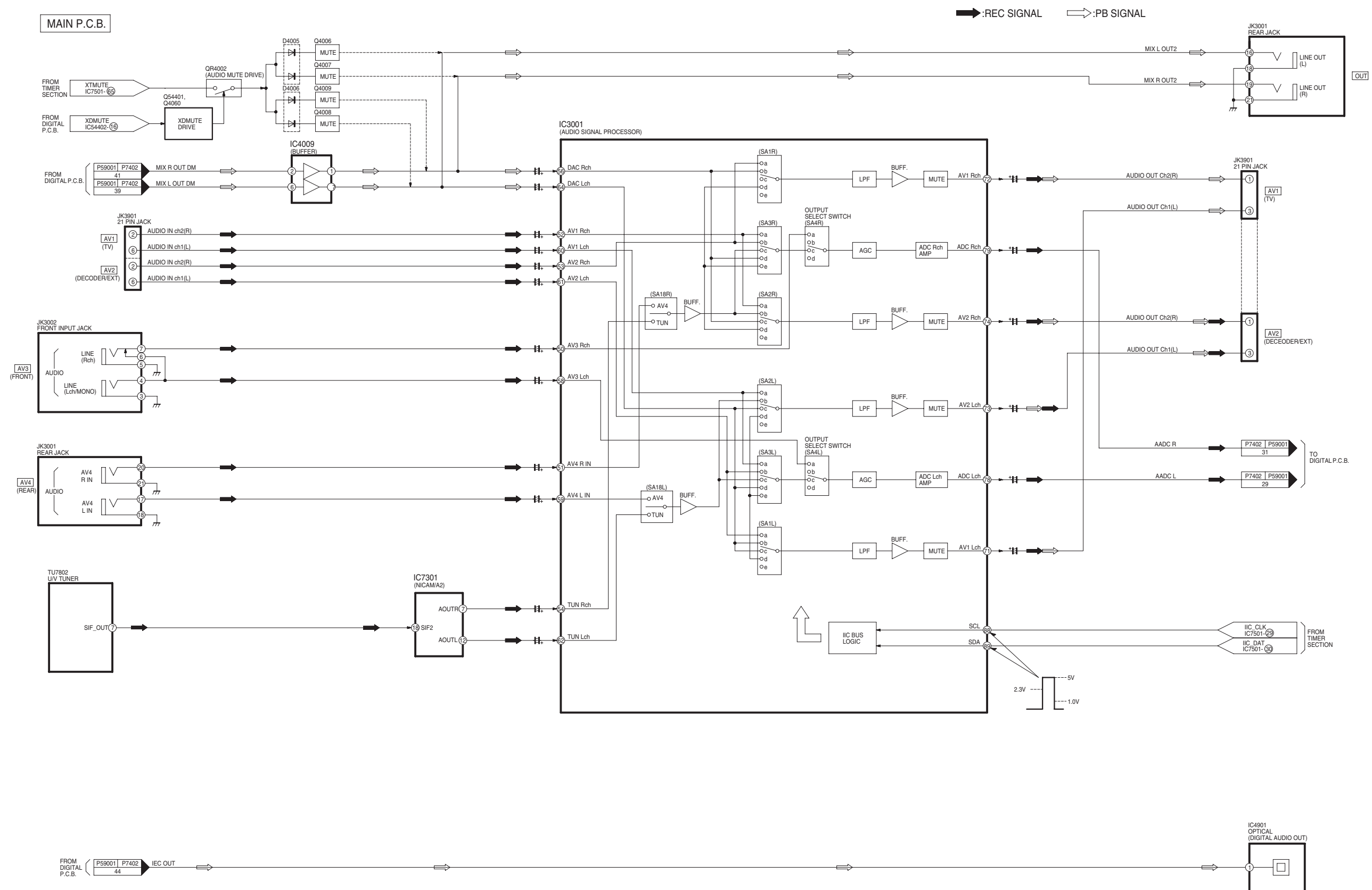
DMR-EH59GA/GC/GN Analog Audio Block Diagram
