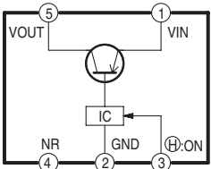
IC7403 PS +5V SWITCHING REGULATOR IC-DETAIL BLOCK DIAGRAM
