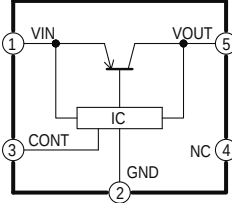
IC7303 +3.3V SWITCHING REGULATOR IC-DETAIL BLOCK DIAGRAM
