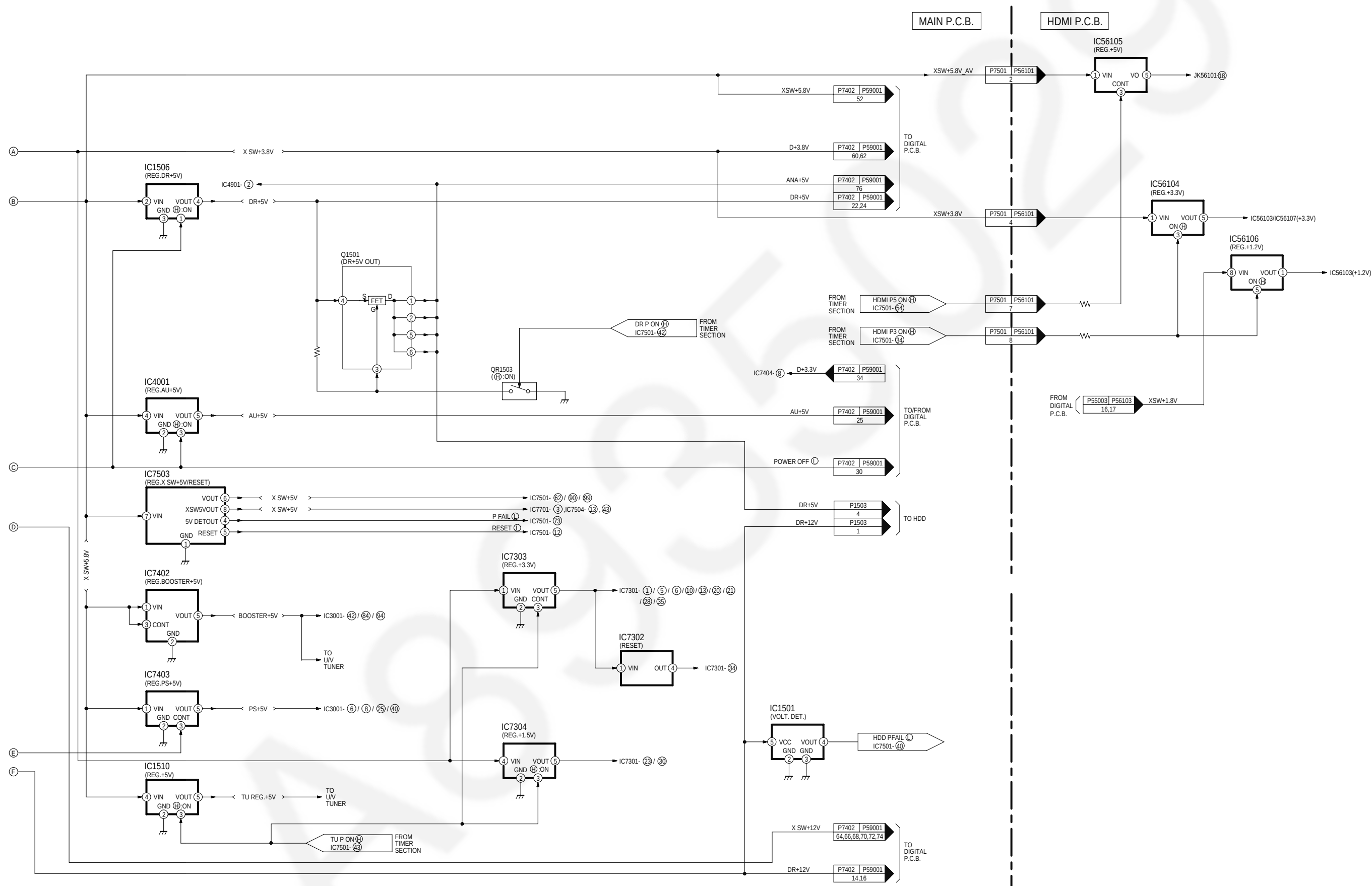
DMR-EH58GN/GC/GCS Power Supply Block Diagram (2/2)
