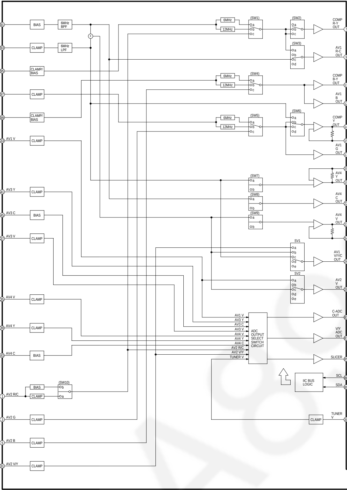
IC3001 VIDEO/AUDIO PROCESSOR IC-DETAIL BLOCK DIAGRAM
