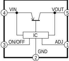
IC7304 +1.5V SWITCHING REGULATOR IC-DETAIL BLOCK DIAGRAM
