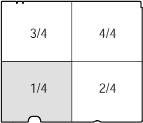
DMR-EH58GN/GC/GCS Main P.C.B. (RFKB79183ET) (1/4 Section)
