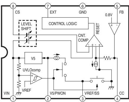
IC1601 SWITCHING IC IC-DETAIL BLOCK DIAGRAM
