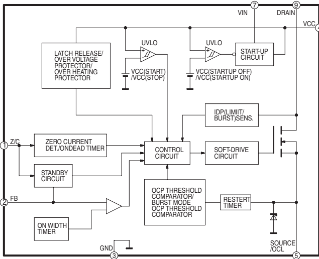
IC1150 SWITCHING IC IC-DETAIL BLOCK DIAGRAM
