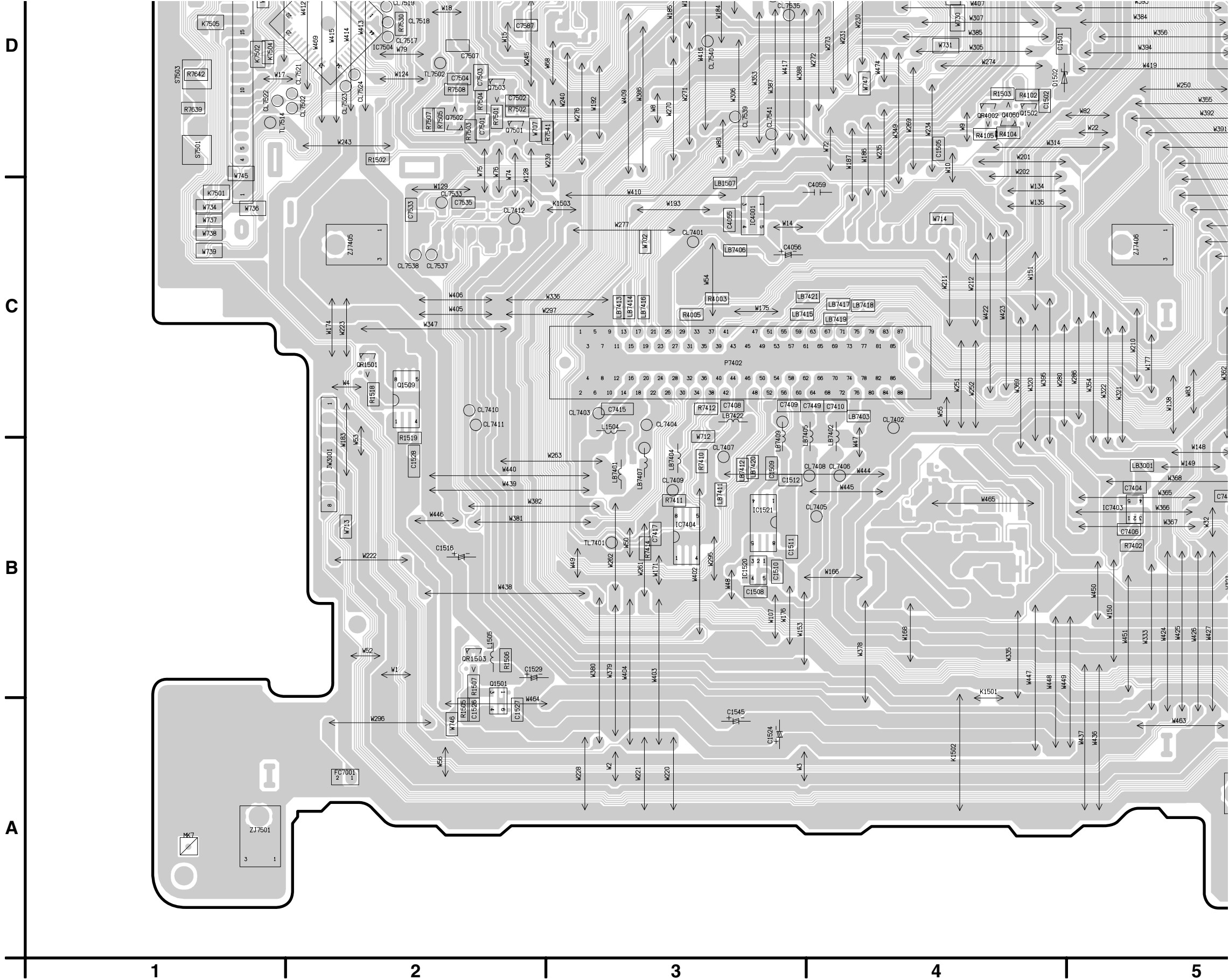
DMR-EH57GN Main P.C.B. (RFKB79156DT) (1/4 Section)
