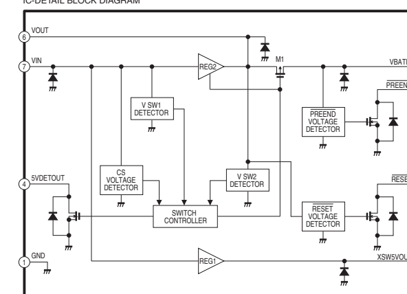
IC7503 RESET,REGULATORR IC IC-DETAIL BLOCK DIAGRAM
