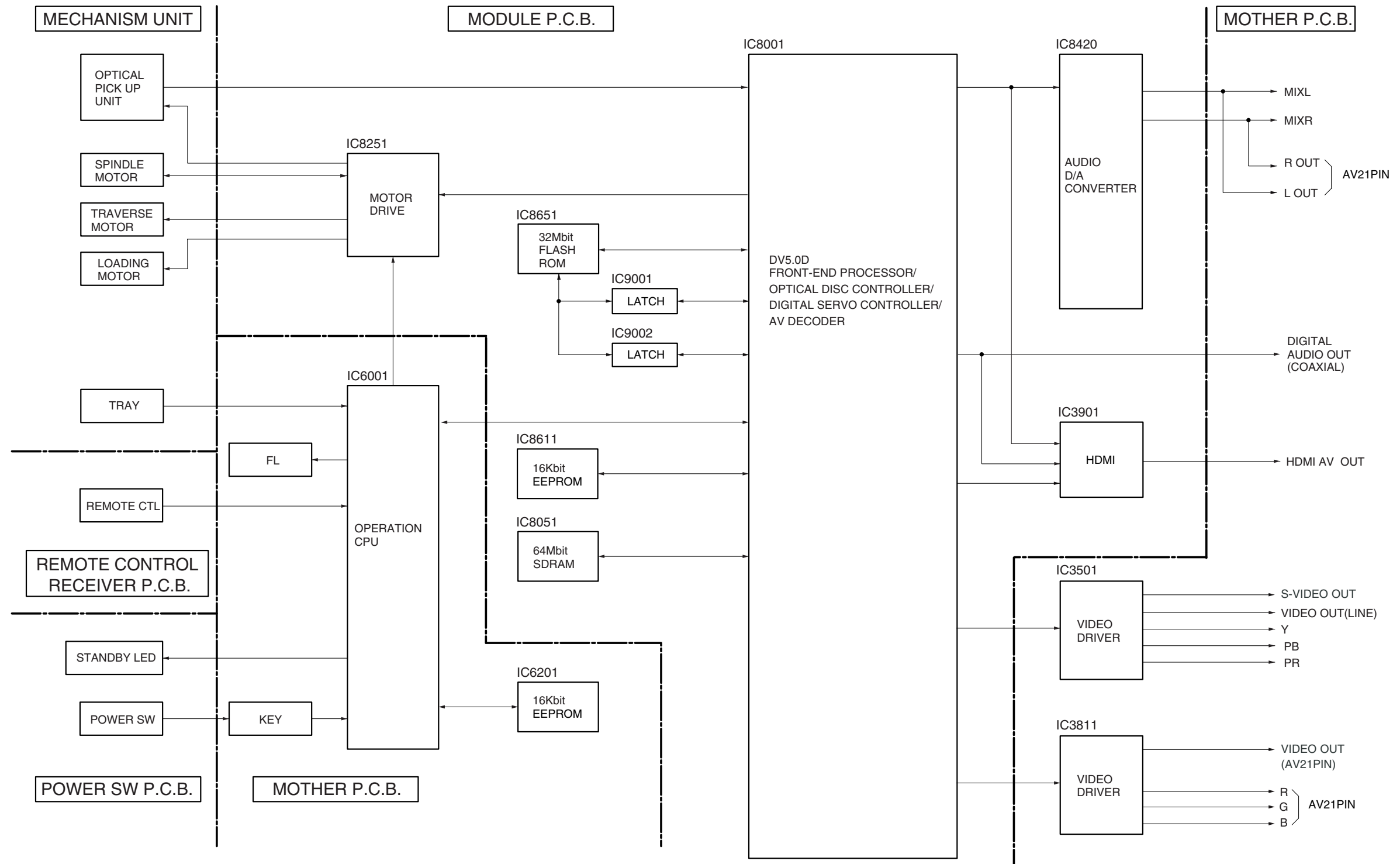
DVD-S54E/EB/EG OVERALL BLOCK DIAGRAM
