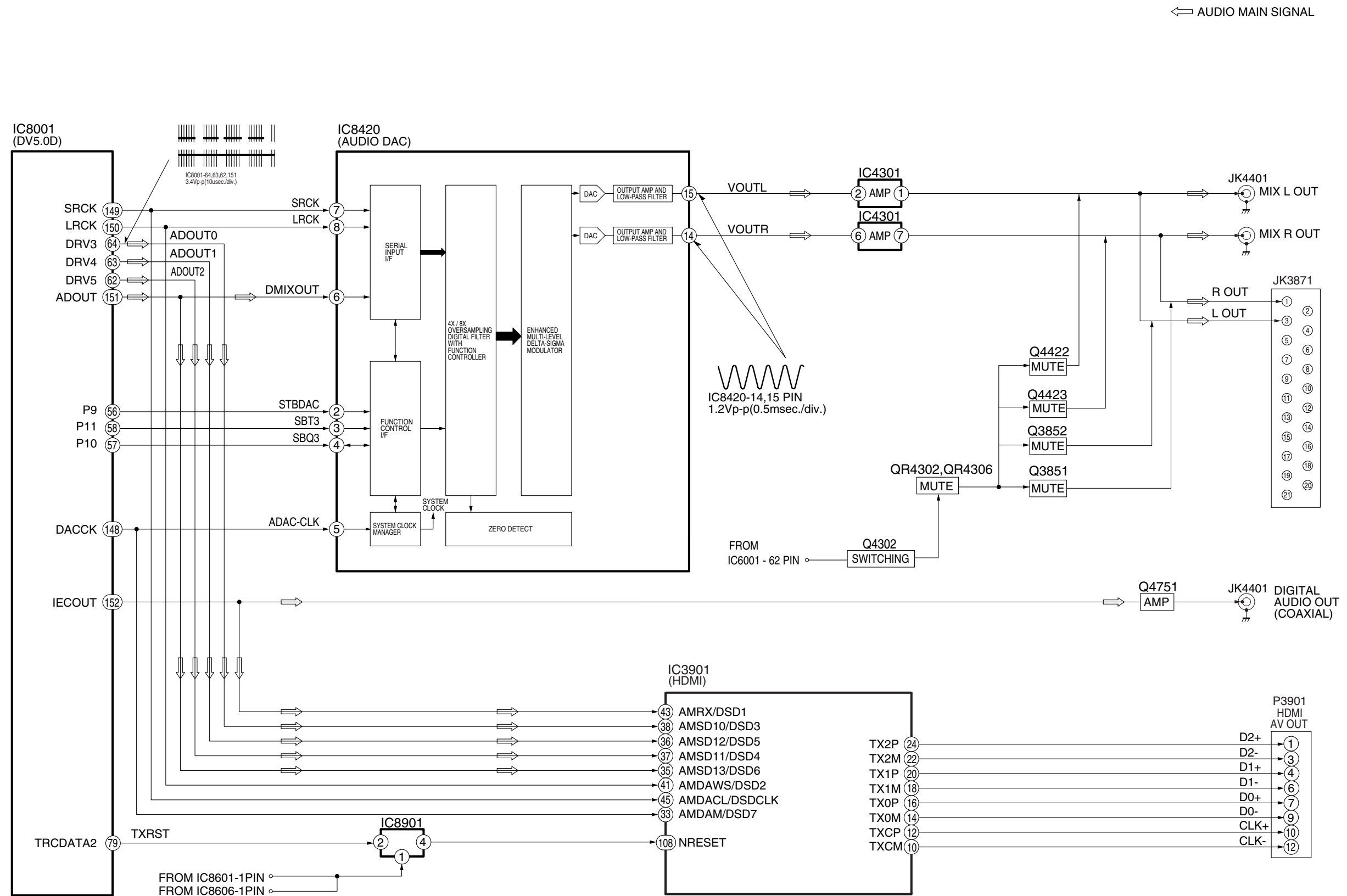
DVD-S54E/EB/EG AUDIO BLOCK DIAGRAM
