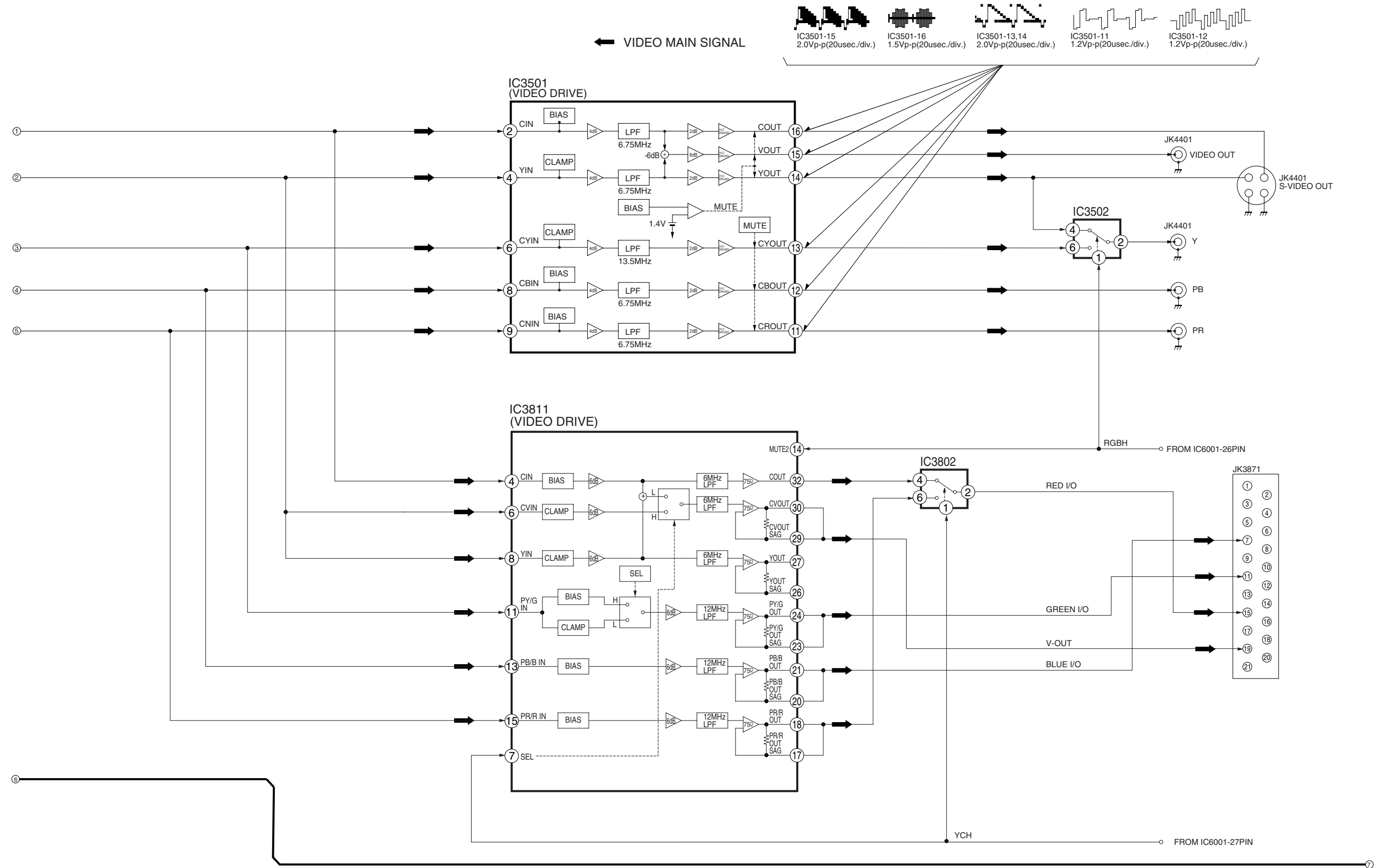
DVD-S54E/EB/EG VIDEO BLOCK DIAGRAM
