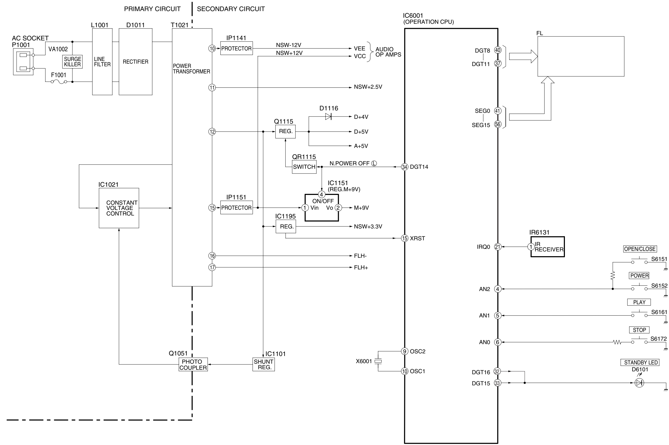
DVD-S54E/EB/EG POWER SUPPLY BLOCK DIAGRAM
