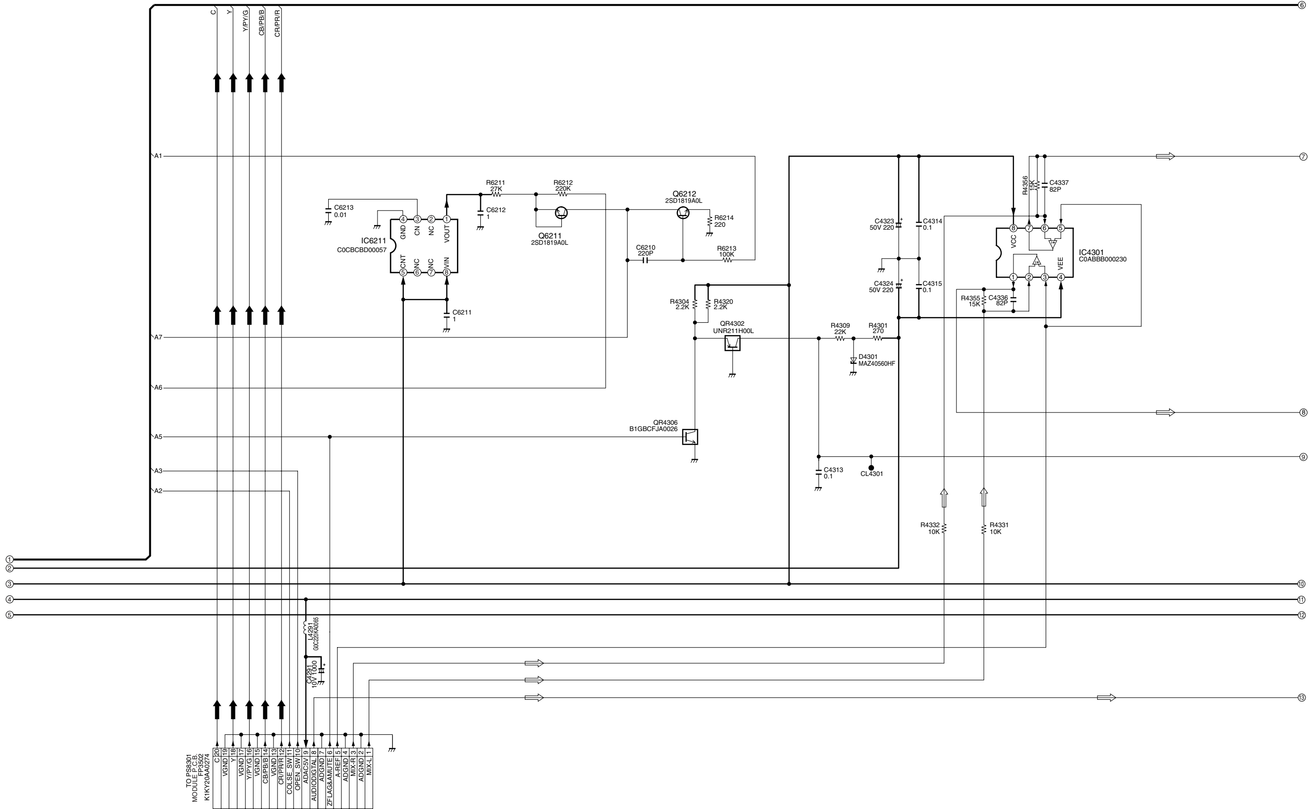
DVD-S54E/EB/EG FRONT & AV OUT SECTION (MOTHER P.C.B.(2/2)) SCHEMATIC DIAGRAM
