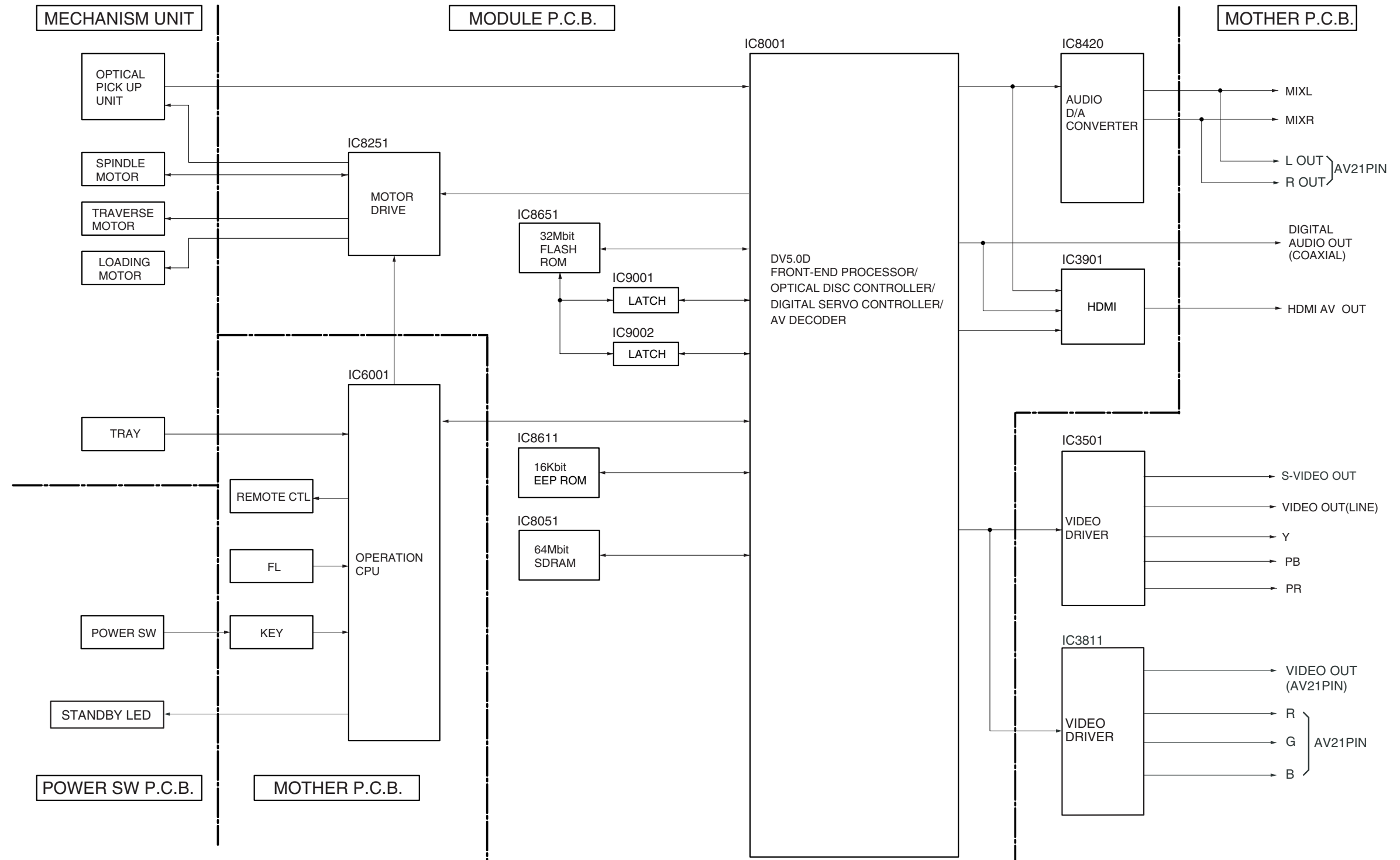
DVD-S53E/EB/EG OVERALL BLOCK DIAGRAM
