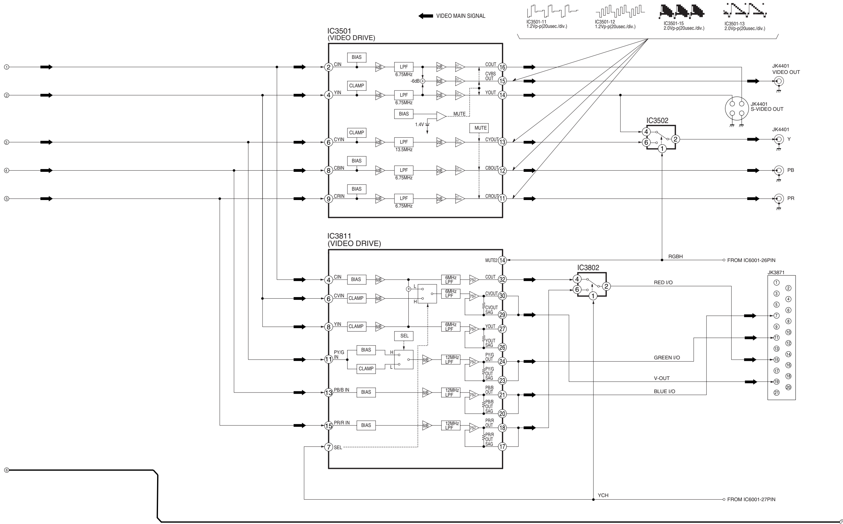
DVD-S53E/EB/EG VIDEO BLOCK DIAGRAM
