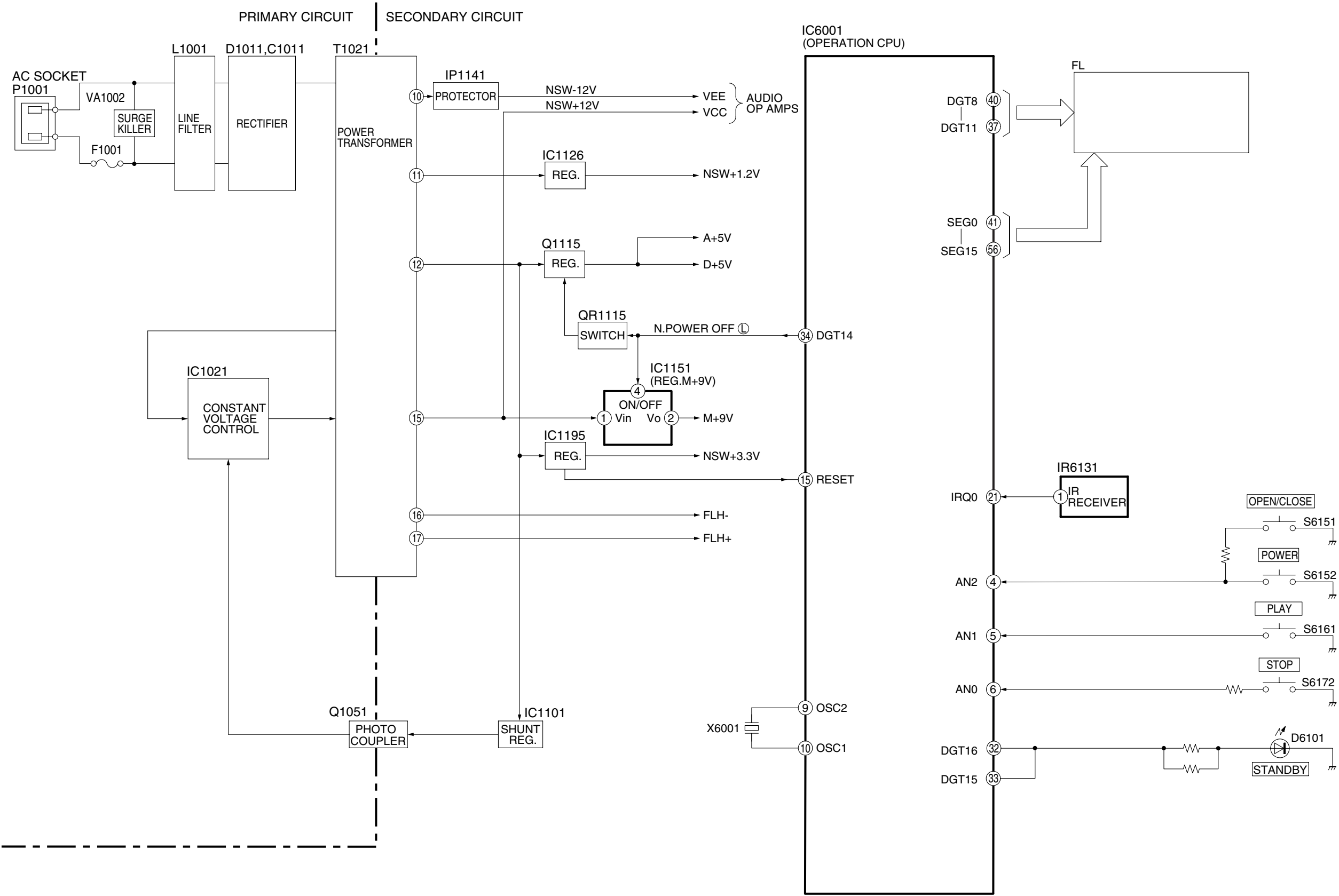
DVD-S53E/EB/EG POWER SUPPLY BLOCK DIAGRAM
