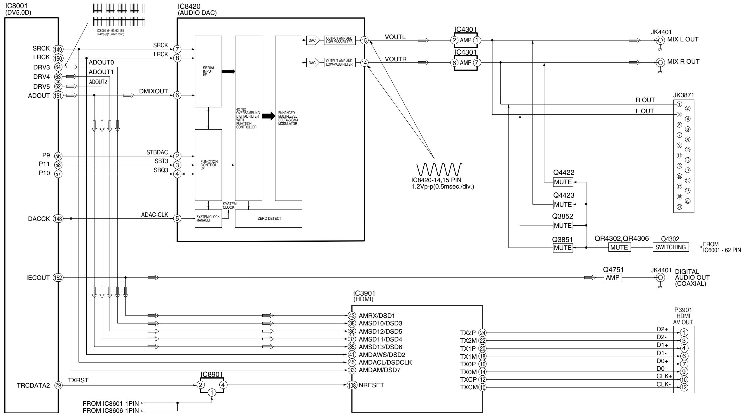
DVD-S53E/EB/EG AUDIO BLOCK DIAGRAM
