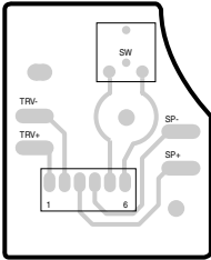
TRV AND SP MOTOR P.C.B.
