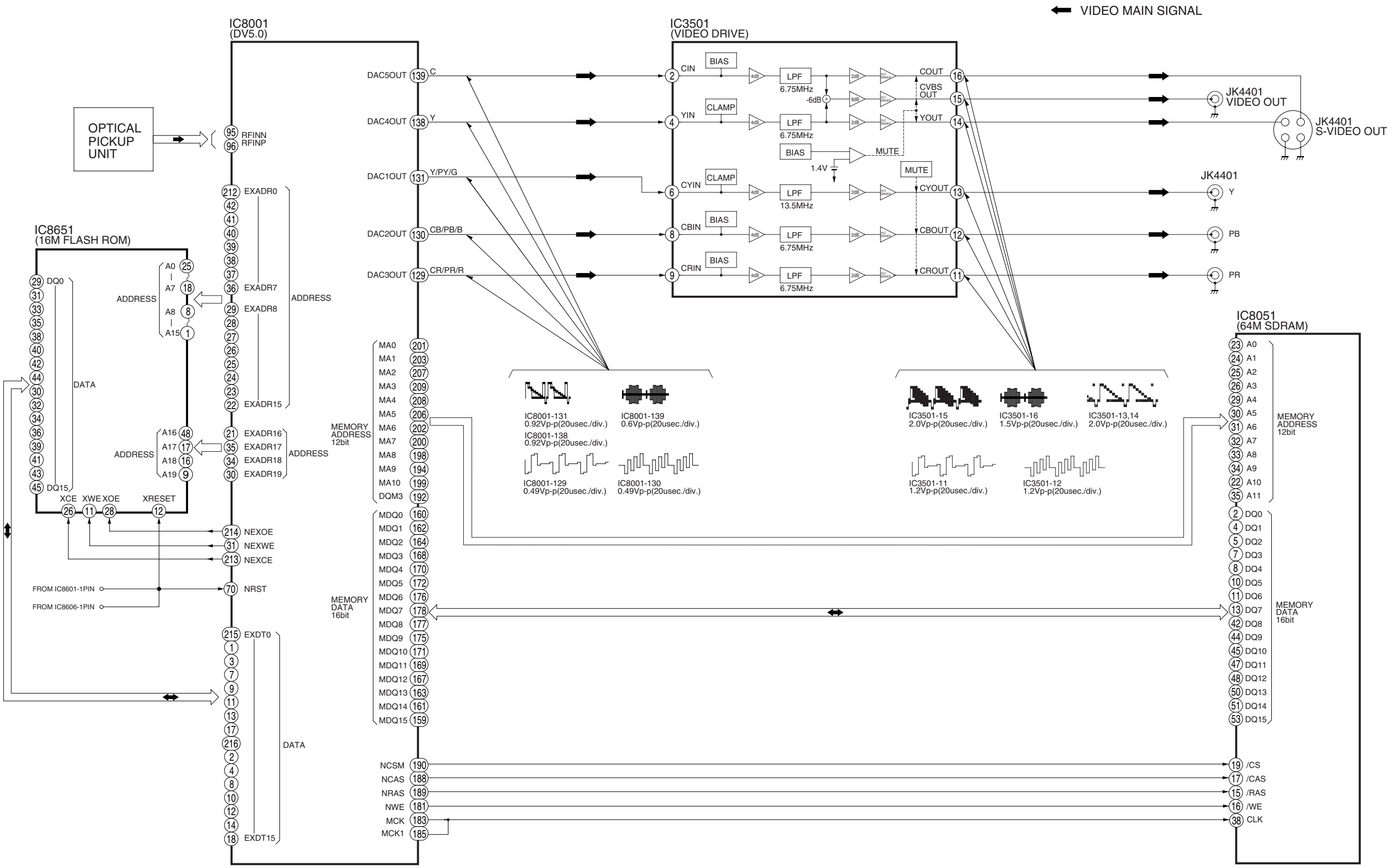
DVD-S33GC/GCA/GCS/GCU/GN VIDEO BLOCK DIAGRAM
