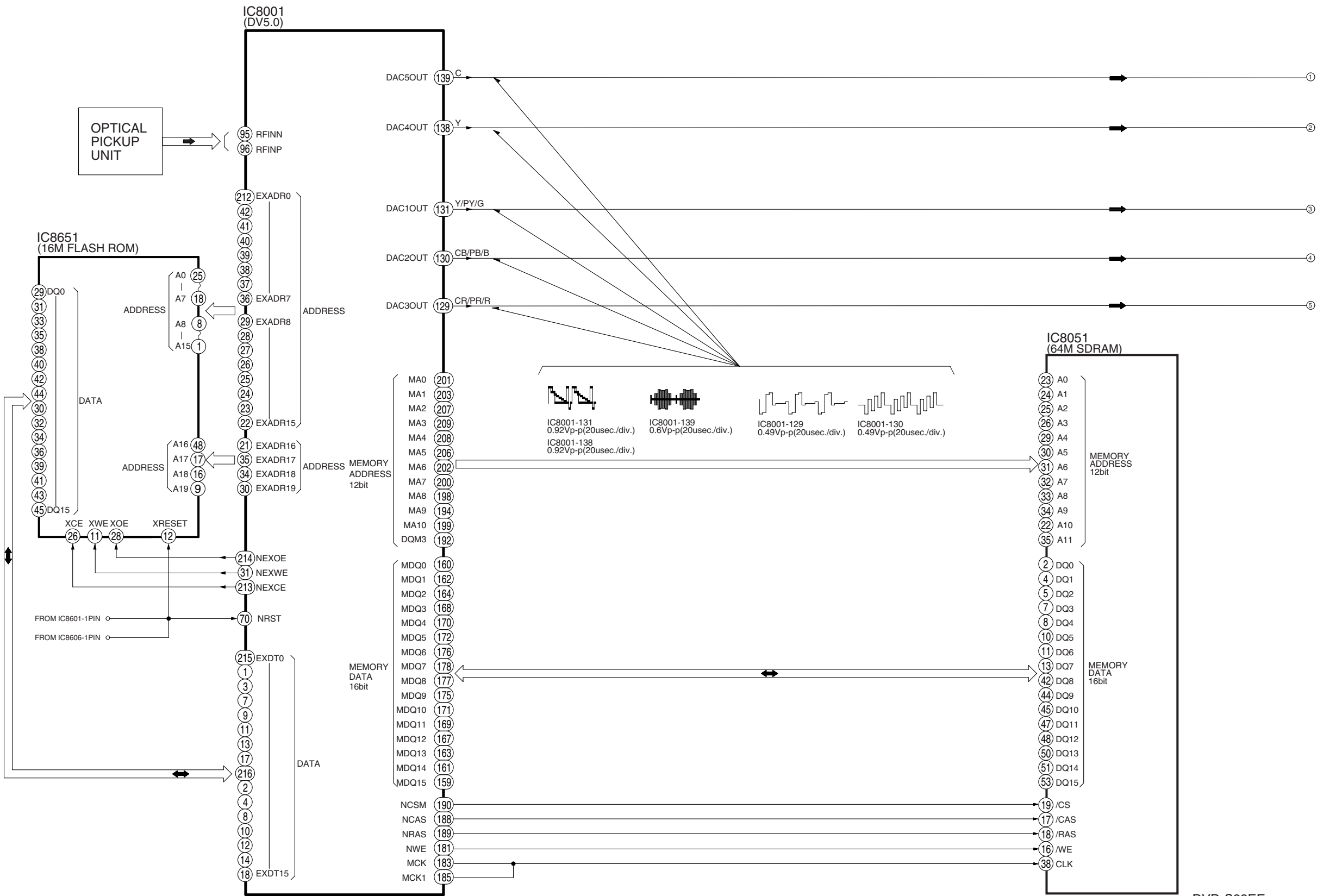
DVD-S33EE VIDEO BLOCK DIAGRAM
