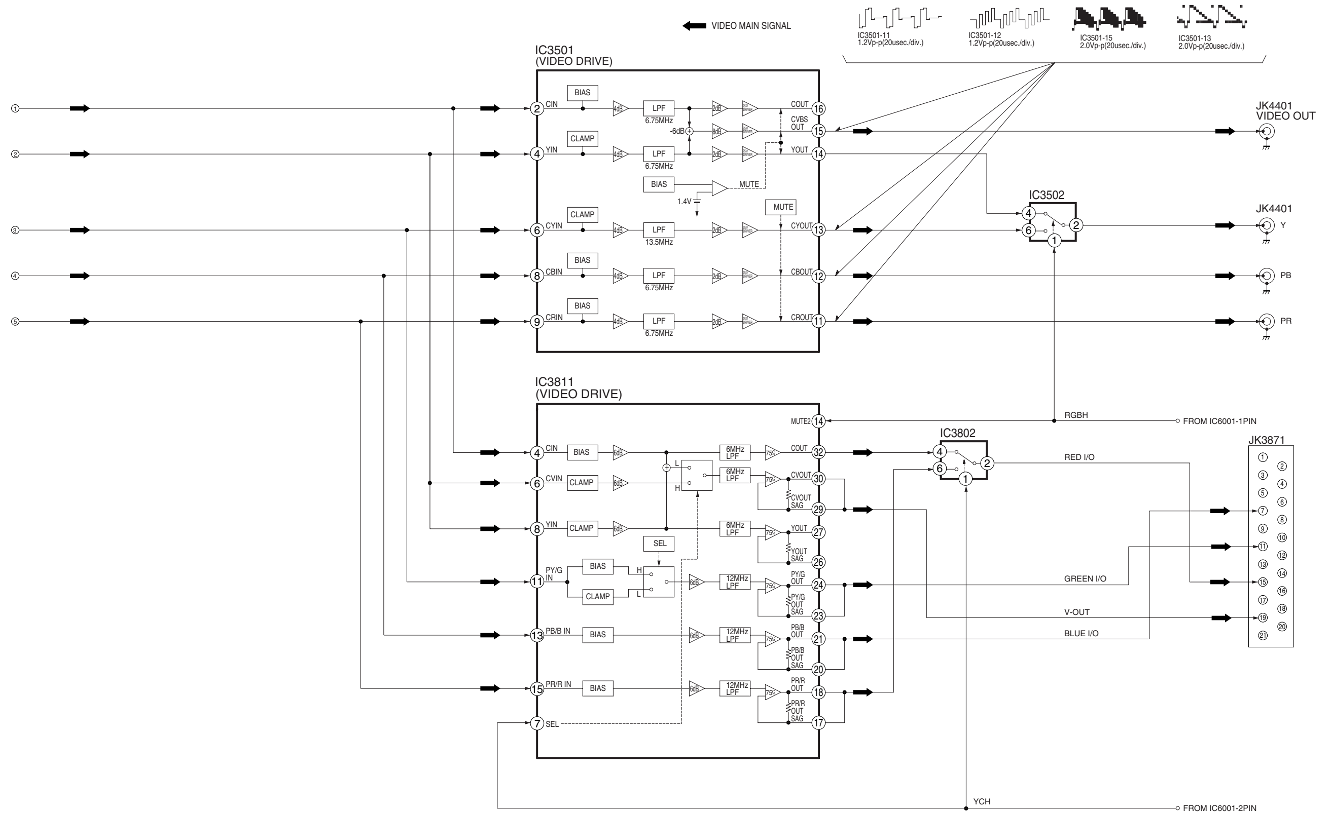
DVD-S33EE VIDEO BLOCK DIAGRAM
