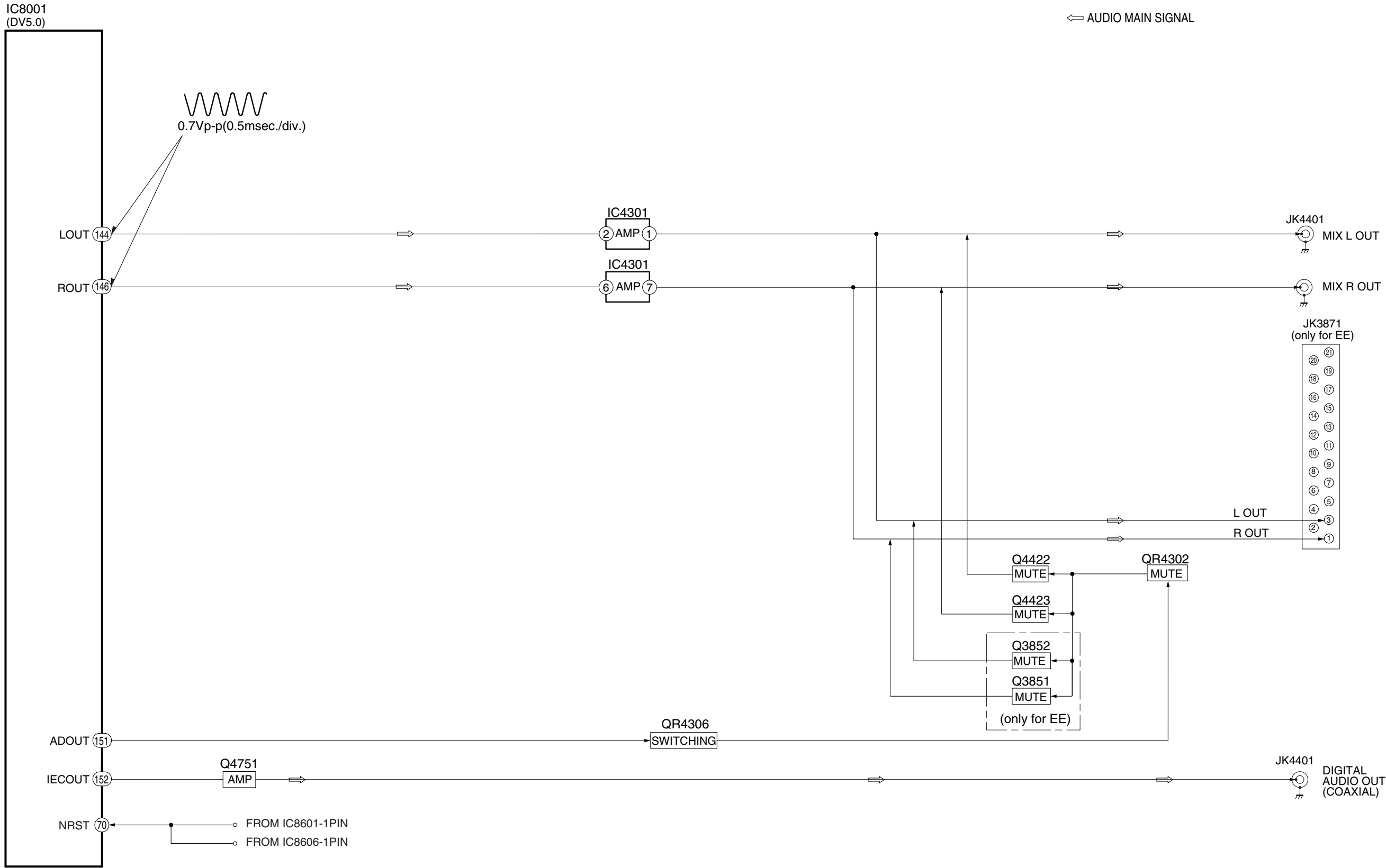
DVD-S33EE/GC/GCA/GCU/GCS/GN AUDIO BLOCK DIAGRAMA
