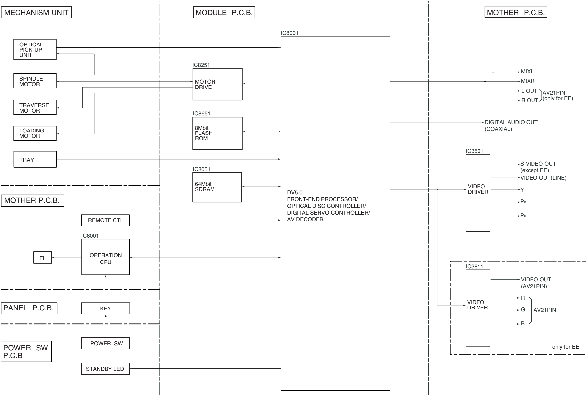
DVD-S325EE/GC/GCA/GCS/GCU OVERALL BLOCK DIAGRAM
