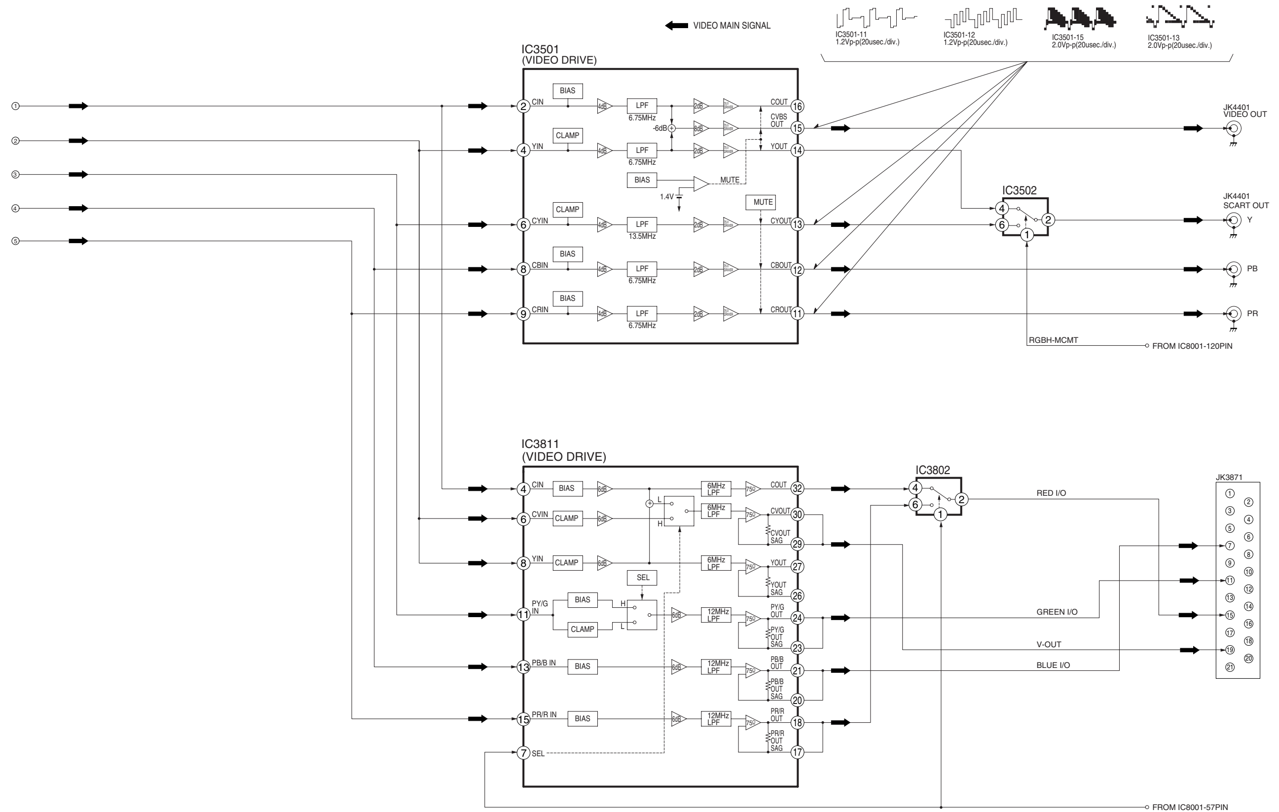
DVD-S325EE VIDEO BLOCK DIAGRAM
