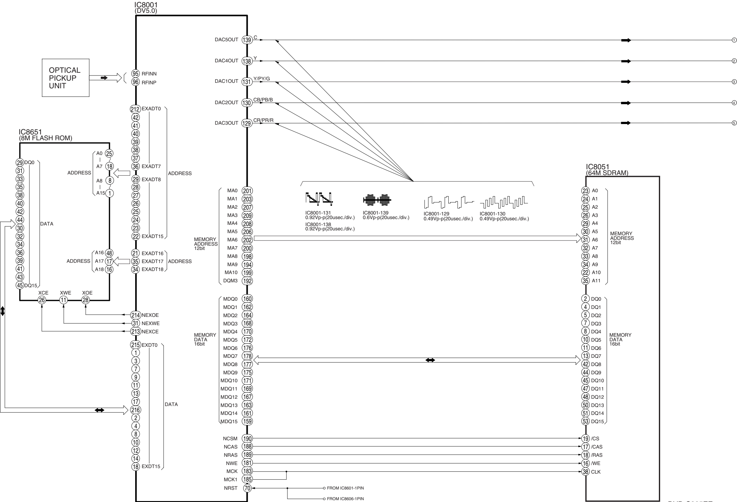
DVD-S325EE VIDEO BLOCK DIAGRAM
