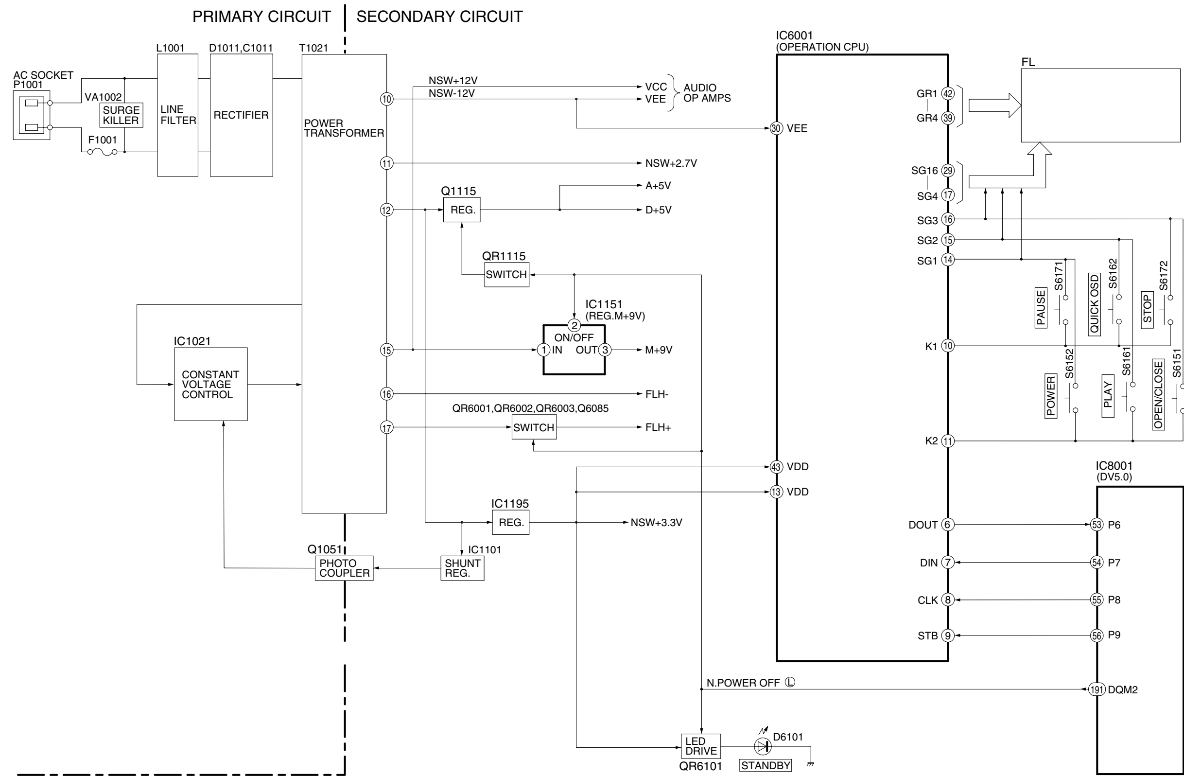
DVD-S325EE/GC/GCA/GCS/GCU POWER SUPPLY BLOCK DIAGRAM
