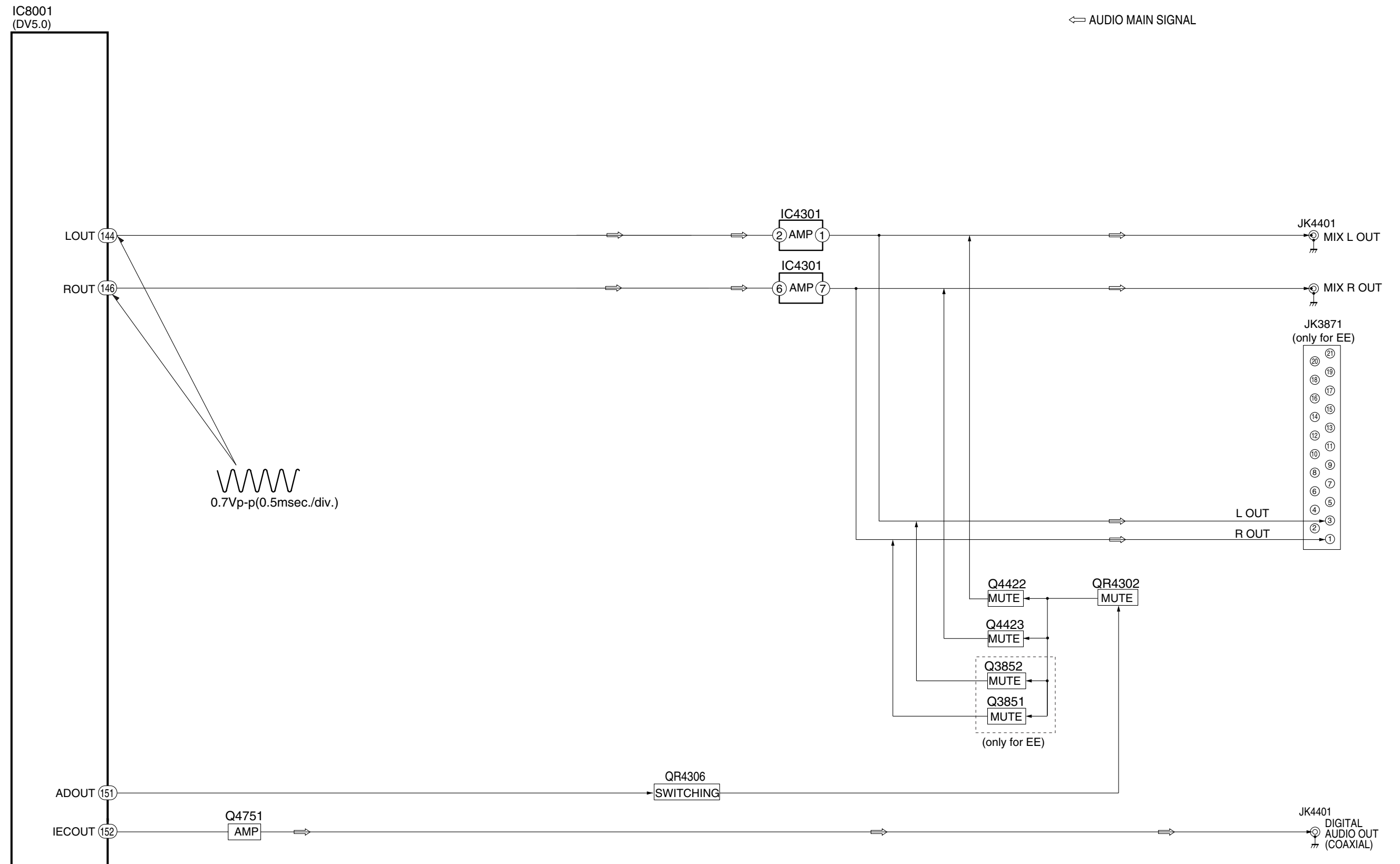
DVD-S325EE/GC/GCA/GCS/GCU AUDIO BLOCK DIAGRAMA
