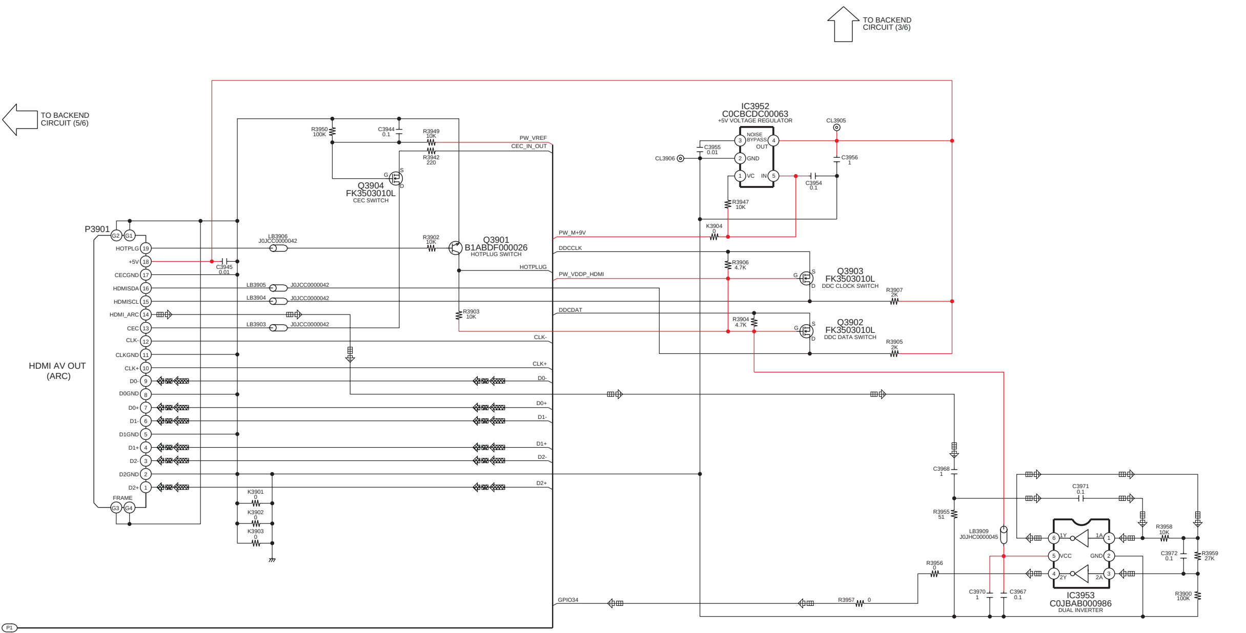
1/6 2/6 3/6 4/6 5/6 6/6 SA-XH73GA/GAX,SA-XH75GA/GAX/GK/GS BACKEND CIRCUIT
