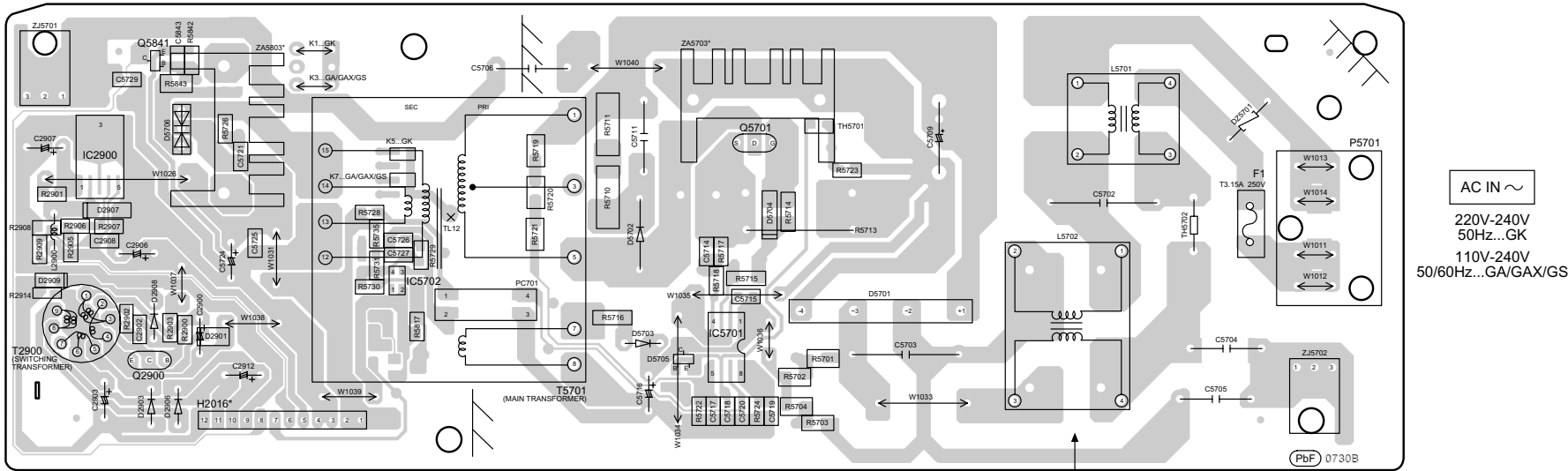
E SMPS P.C.B. (REP4764C...GA/GAX/GS) (REP4764D...GK)
