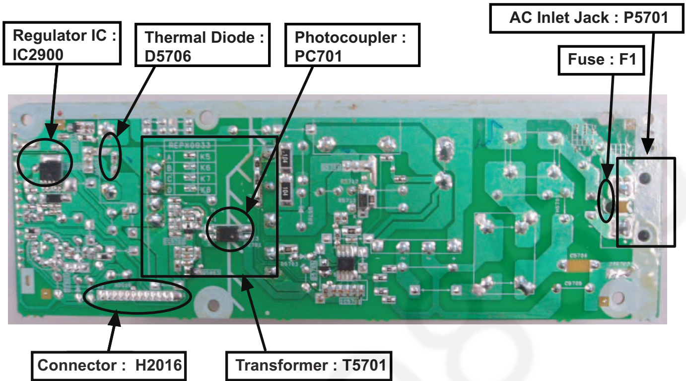
Figure 10-1 SMPS P.C.B.
