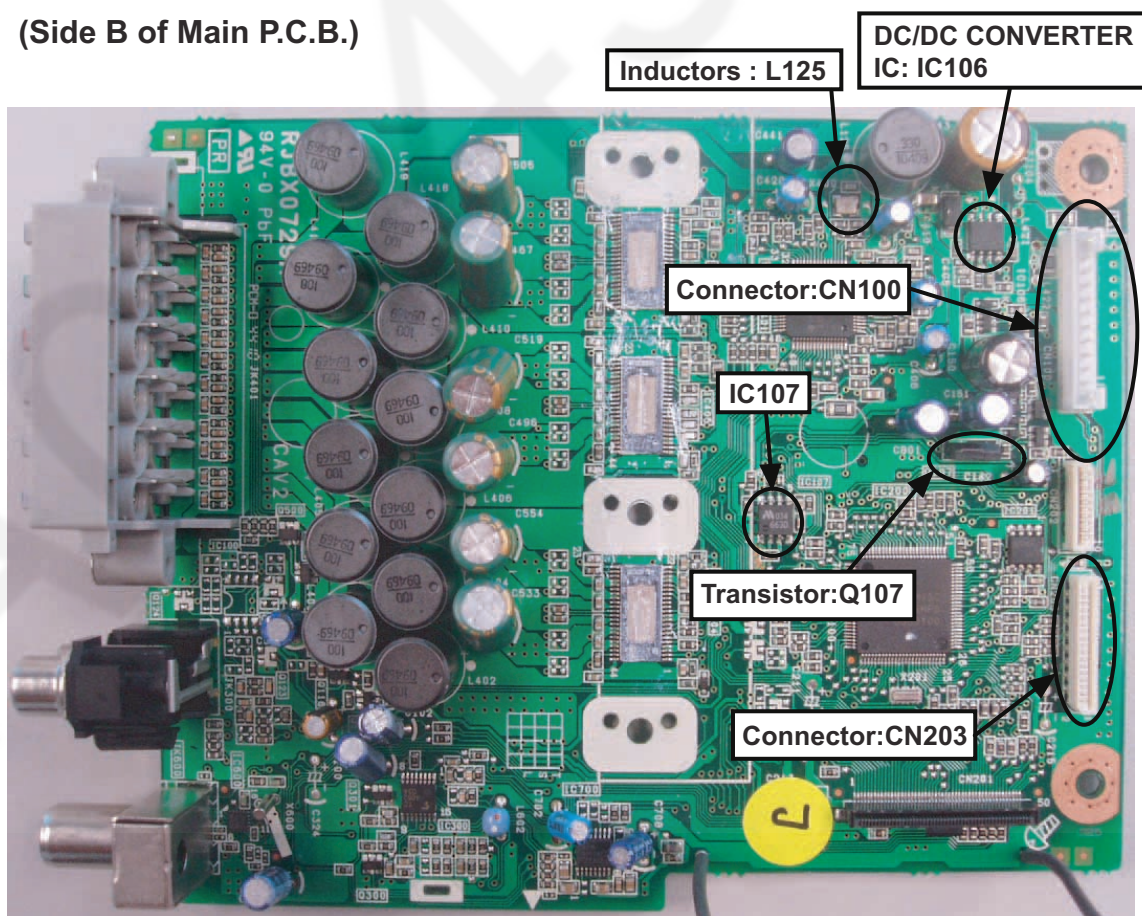
Figure 10-2. Main P.C.B.
