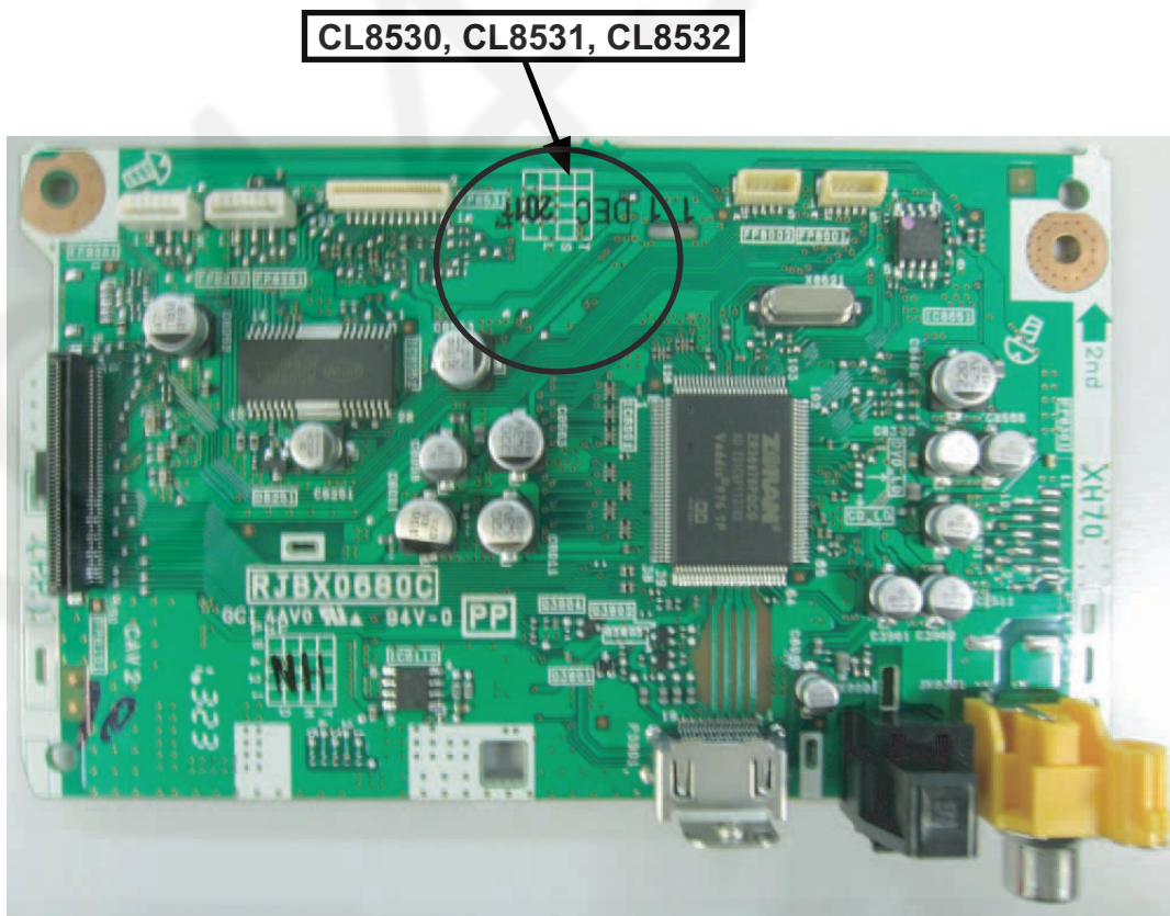
Figure 10-3 Backend P.C.B.
