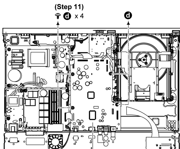
Main P.C.B. (Step 12)
