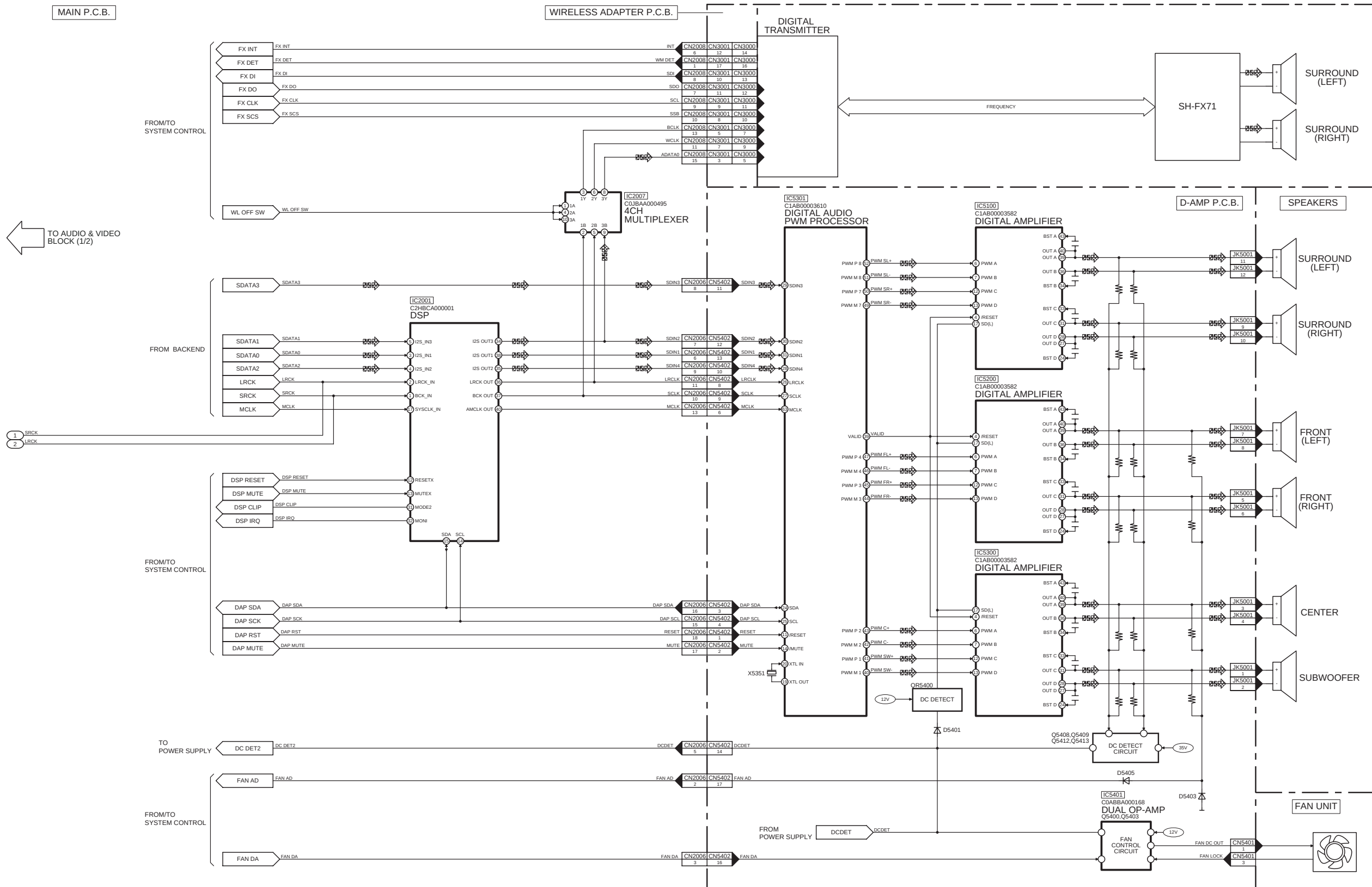
SA-XH185EE/GS AUDIO & VIDEO (2/2) BLOCK DIAGRAM
