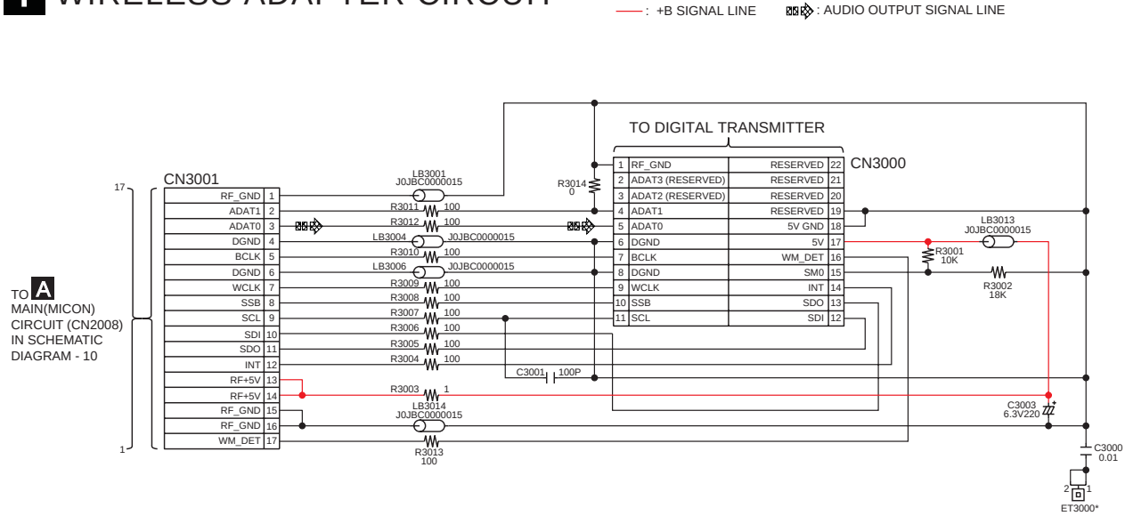
SCHEMATIC DIAGRAM - 22 I WIRELESS ADAPTER CIRCUIT
