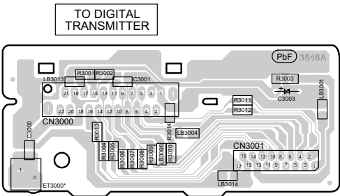
I WIRELESS ADAPTER P.C.B. (REP4762A)
