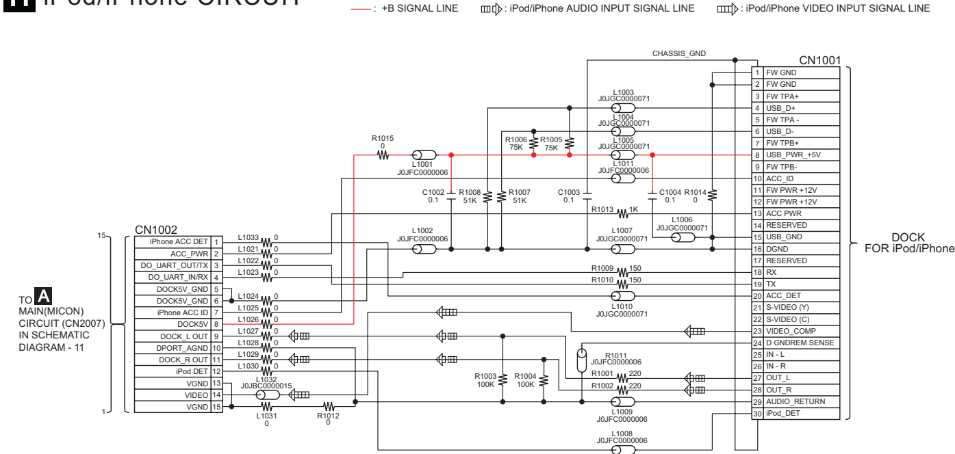
SCHEMATIC DIAGRAM - 22 H iPod/iPhone CIRCUIT
