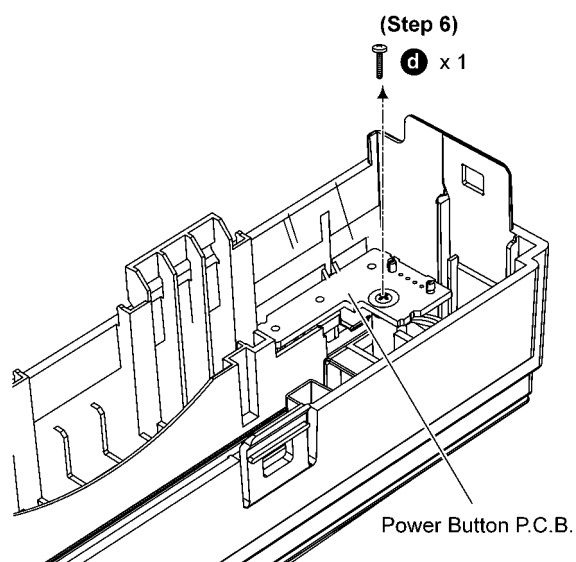
Step 7 Lift up Power Button P.C.B..
