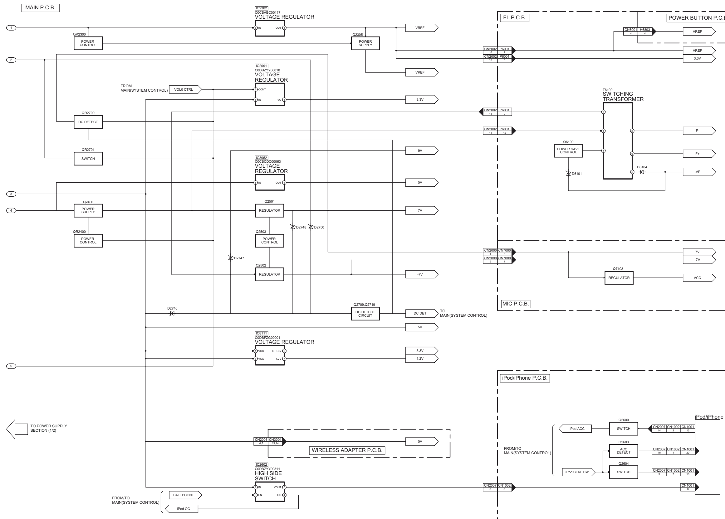
SA-PT980GA/GS/GW POWER SUPPLY(2/2) BLOCK DIAGRAM
