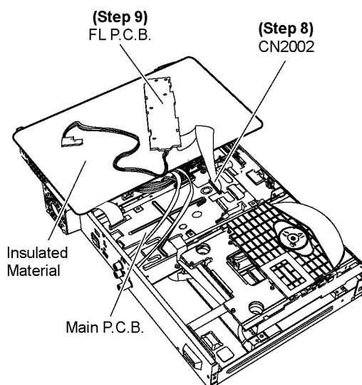
Step 9 Proceed to check & repair FL P.C.B..
