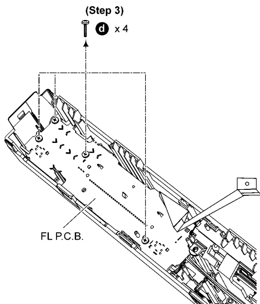
Step 4 Release 1 catch on FL P.C.B..
