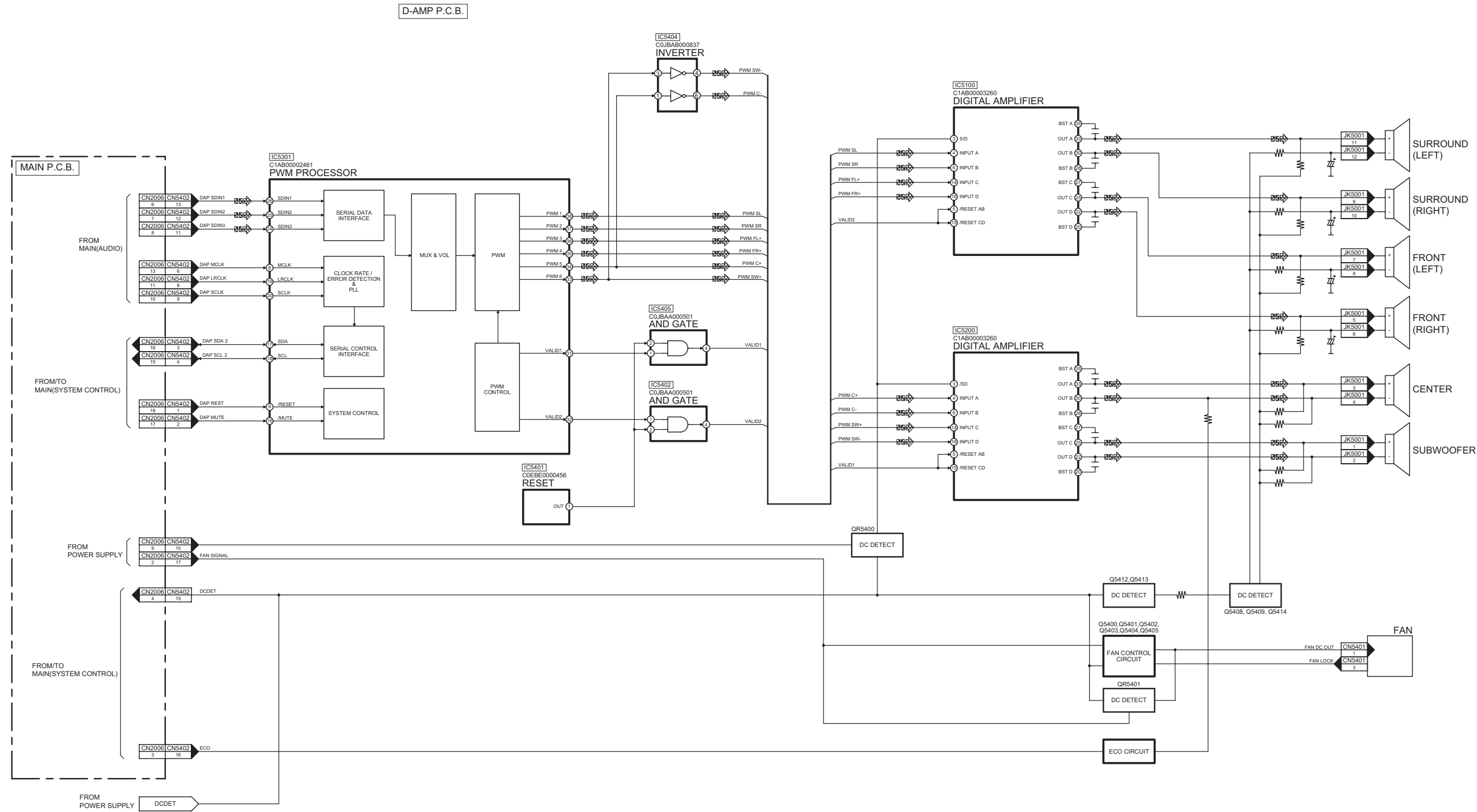
SA-PT980GA/GS/GW DIGITAL AUDIO BLOCK DIAGRAM
