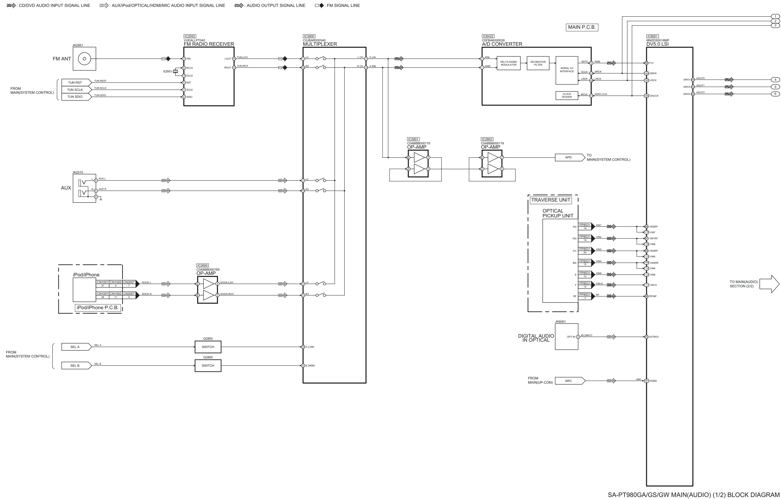
SA-PT980GA/GS/GW MAIN(AUDIO) (1/2) BLOCK DIAGRAM
