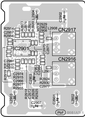
E POWER P.C.B. (REPX0801AB...GW) (REPX0801BB...GA/GS)
