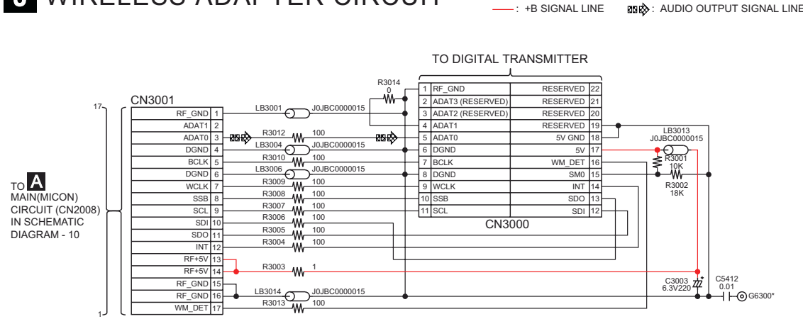
J WIRELESS ADAPTER CIRCUIT
