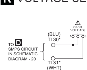
K VOLTAGE SELECTOR CIRCUIT
