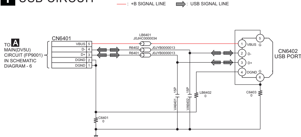
I USB CIRCUIT
