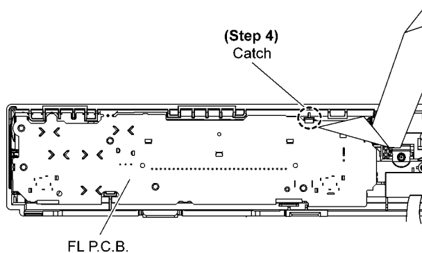
Step 5 Lift up FL P.C.B..
