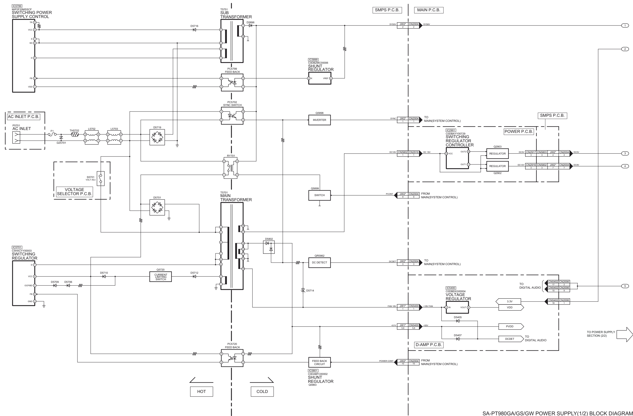
SA-PT980GA/GS/GW POWER SUPPLY(1/2) BLOCK DIAGRAM
