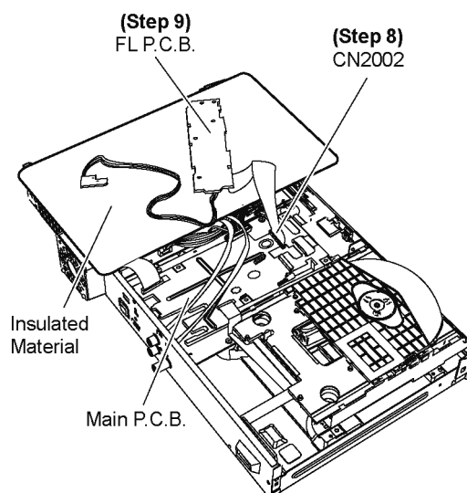
Step 9 Proceed to check & repair FL P.C.B..
