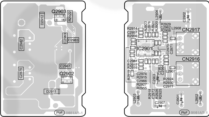
E POWER P.C.B. (REPX0801AB...GW) (REPX0801BB...GA/GS)
